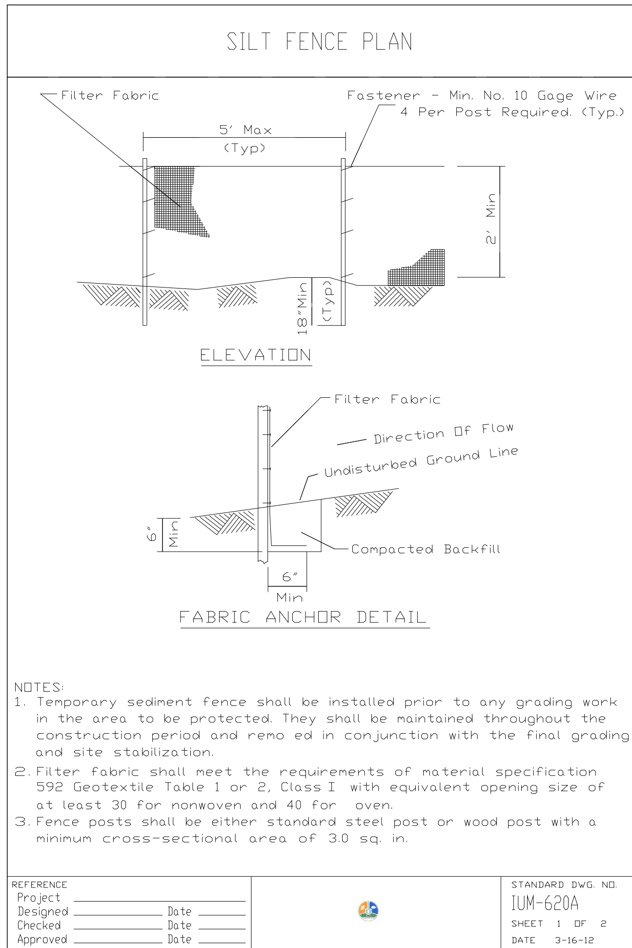
5 Silt Fence D1 NOT TO SCALE
