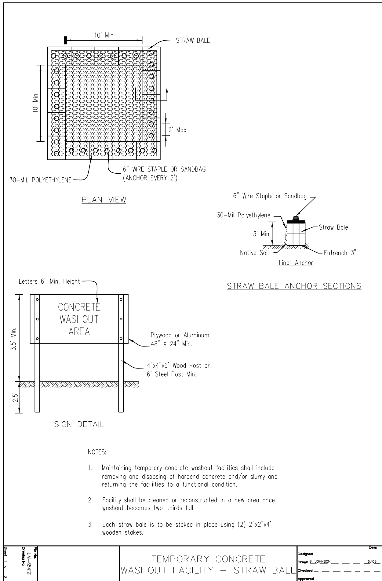
4 Concrete Washout D1 NOT TO SCALE
