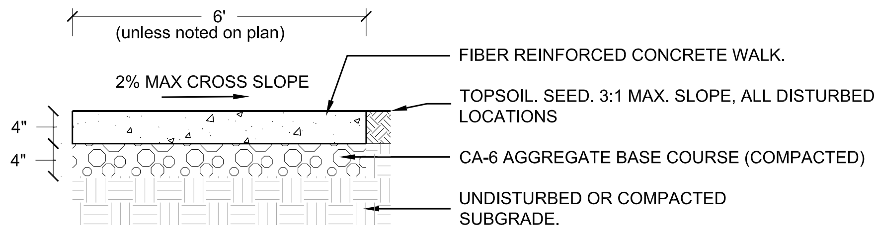
1 Sidewalk Section D1 NOT TO SCALE
