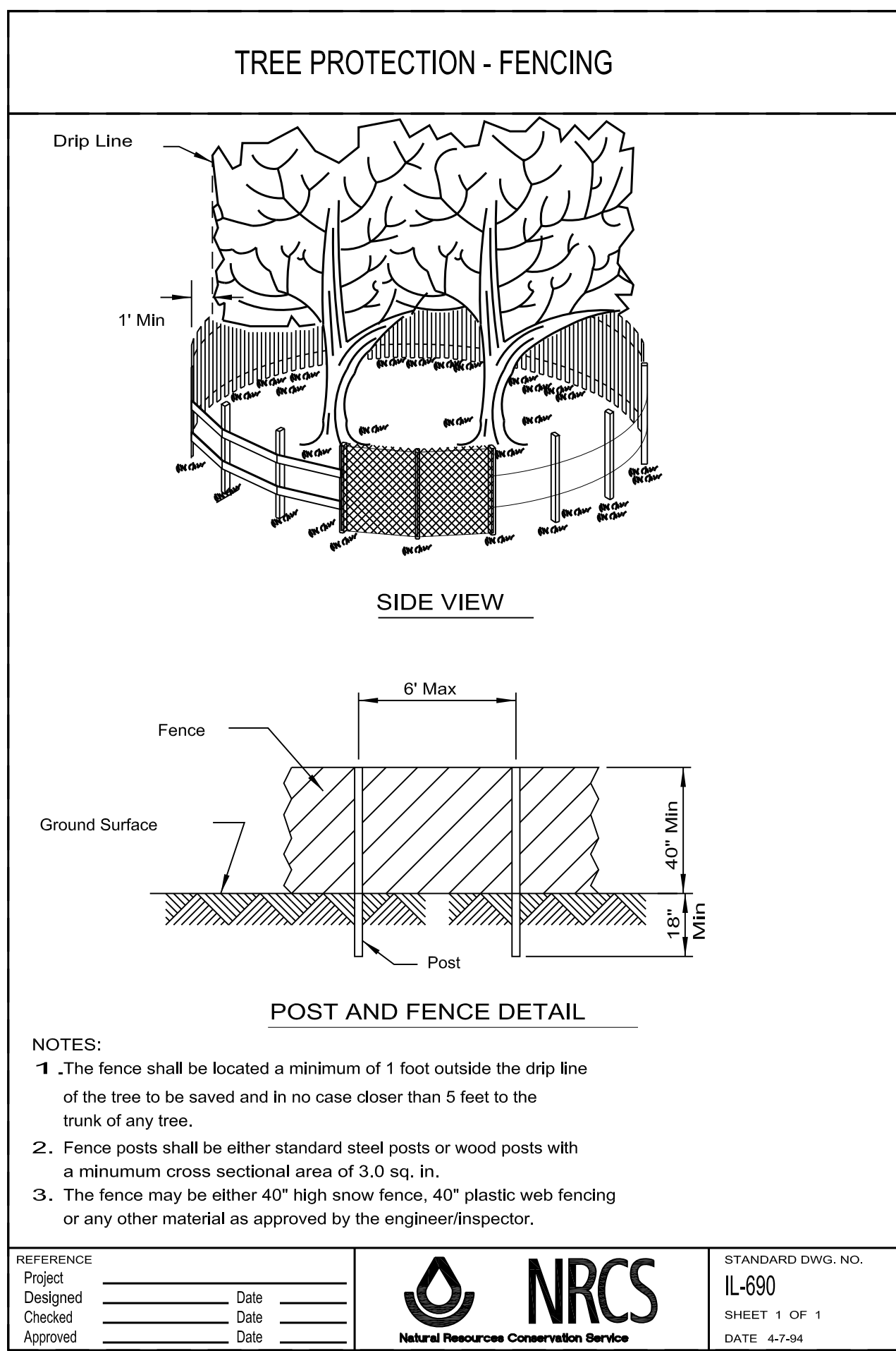
3 Tree Protection D1 NOT TO SCALE
