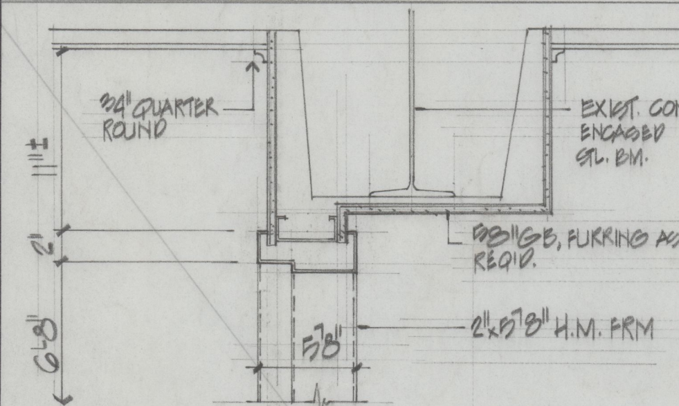
1 HEAD DETAIL 3 1/2" = 1'-0"
