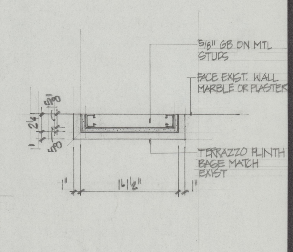
8 ARCH DETAIL 2 1/2 = 10'
