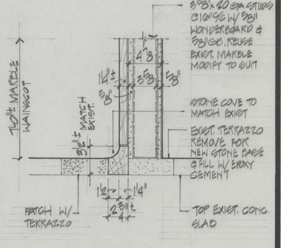
10 BASE DETAIL 2 1/2 = 10'
