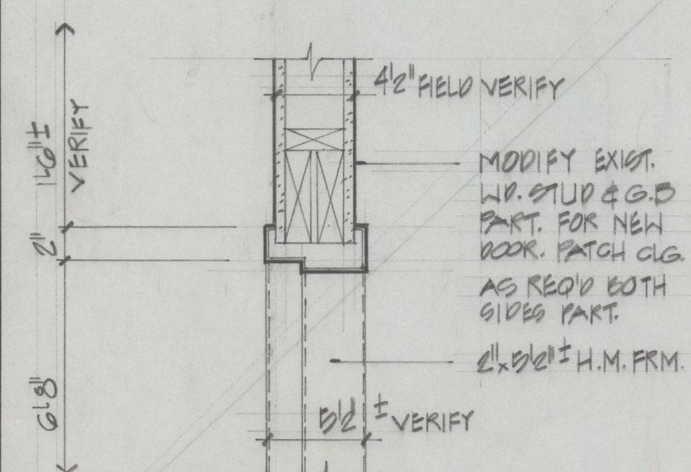
3 HEAD DETAIL 3 1/2" = 1'-0"
