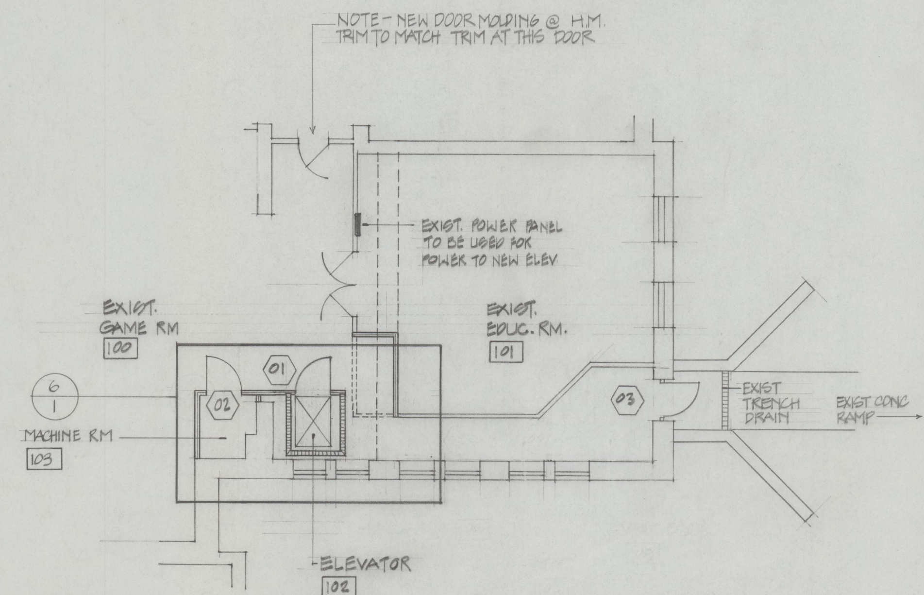
LOWER LEVEL PLAN 1/8" = 1'-0"
