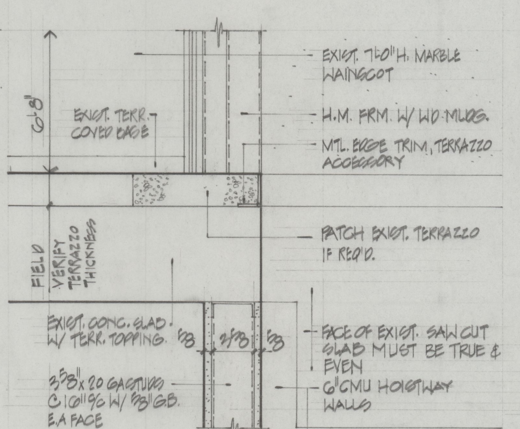
6 SILL DETAIL 2 1/2 = 10'
