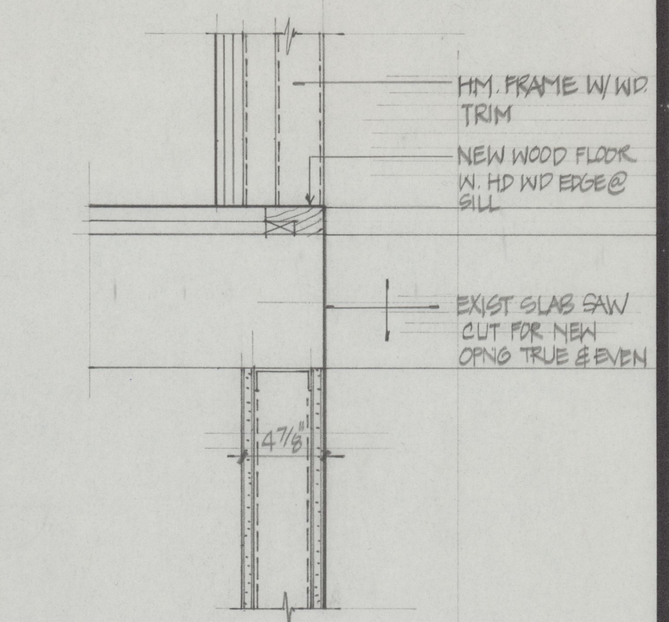
7 SILL DETAIL 2 1/2 = 10'
