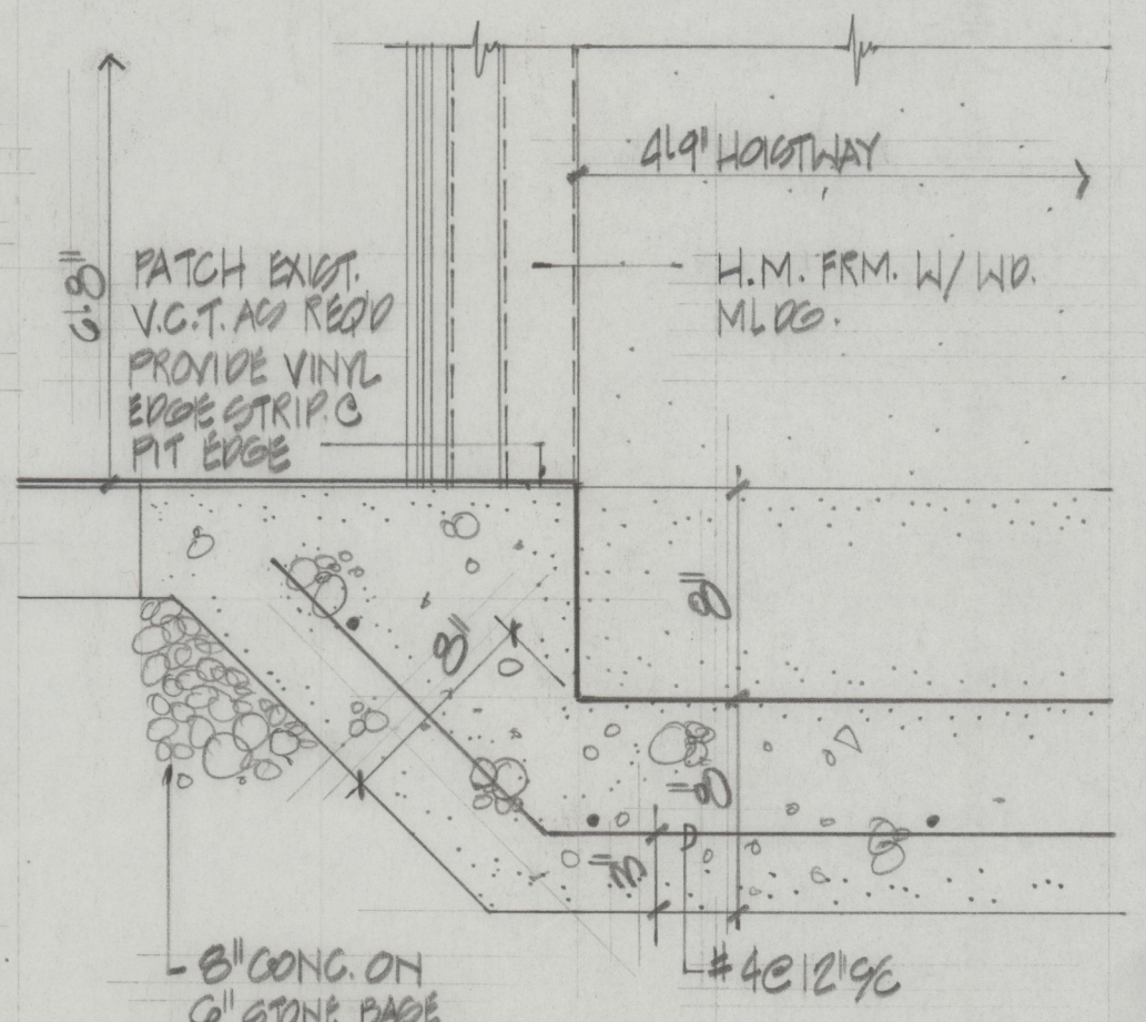
5 SILL DETAIL 2 1/2 = 10'
