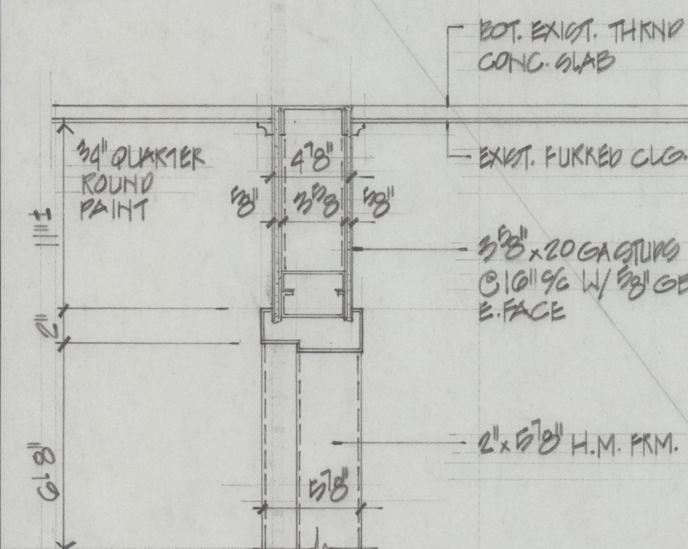
1 HEAD DETAIL 3 1/2" = 1'-0"
