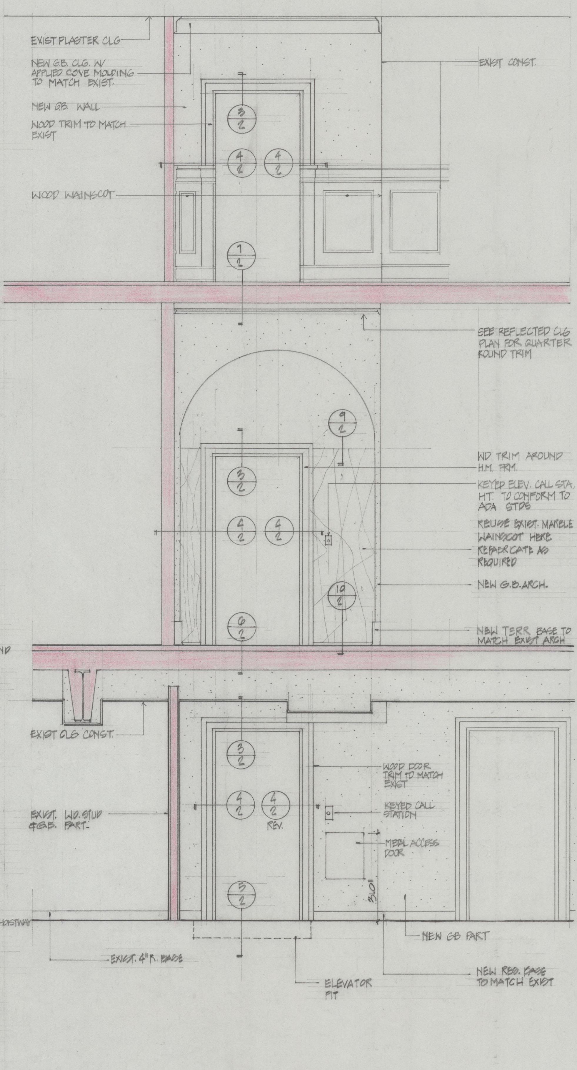
2 HOISTWAY ENTRANCE ELEVATIONS 2 1/2 = 10'
