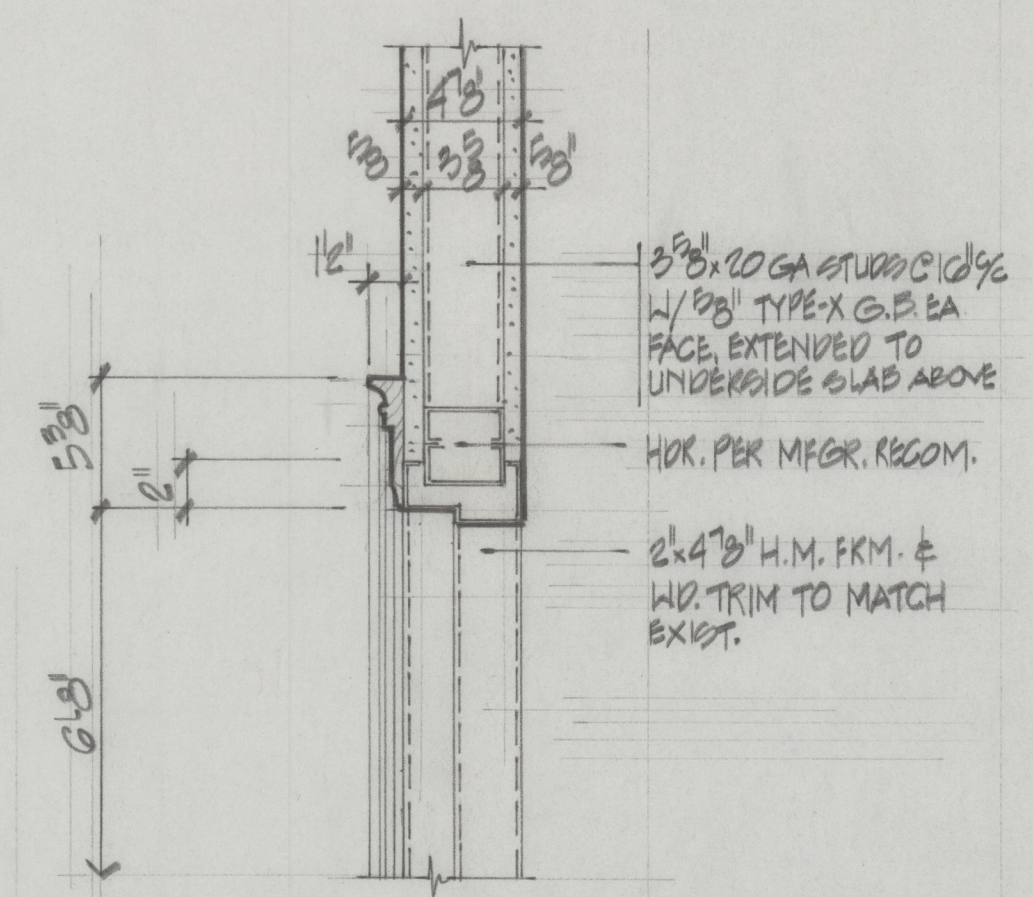
3 HEAD DETAIL 2 1/2 = 10'
