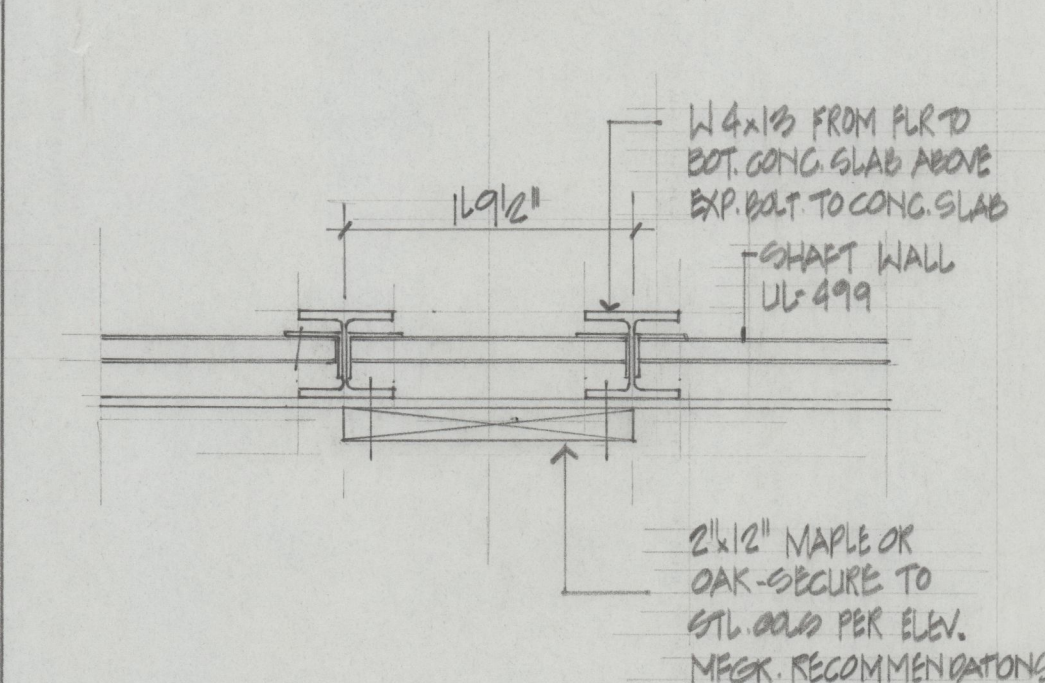
9 ELEVATOR HOISTWAY DETAIL 3 1/2" = 1'-0"
