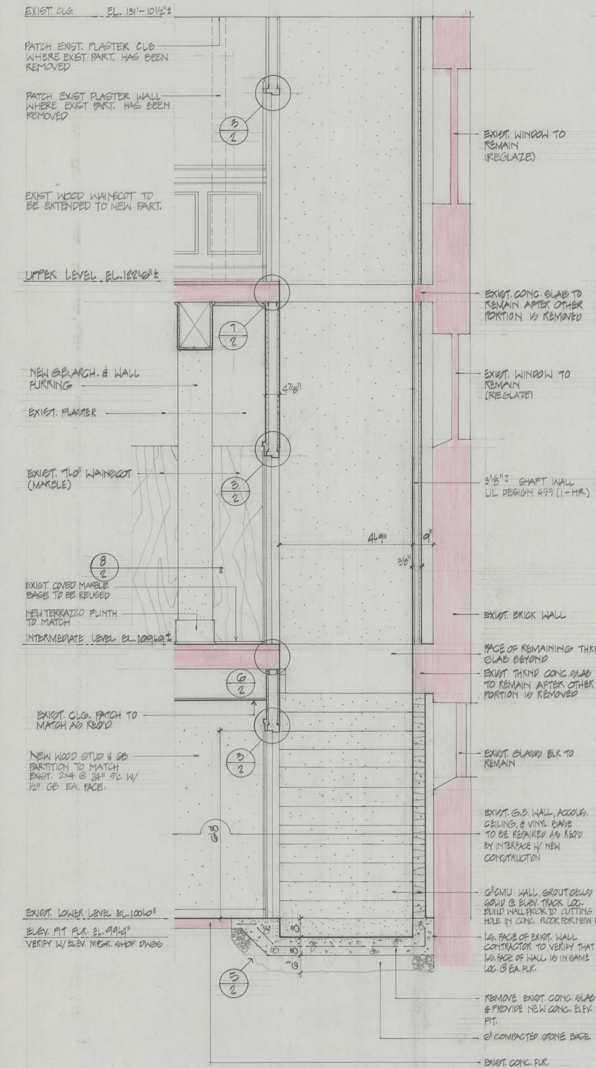
1 HOISTWAY SECTION 2 1/2 = 10'
