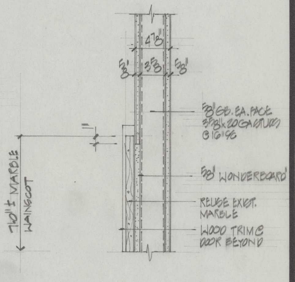
9 WAINSCOT DETAIL 2 1/2 = 10'
