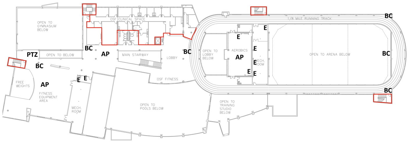
Second Floor - Layout
