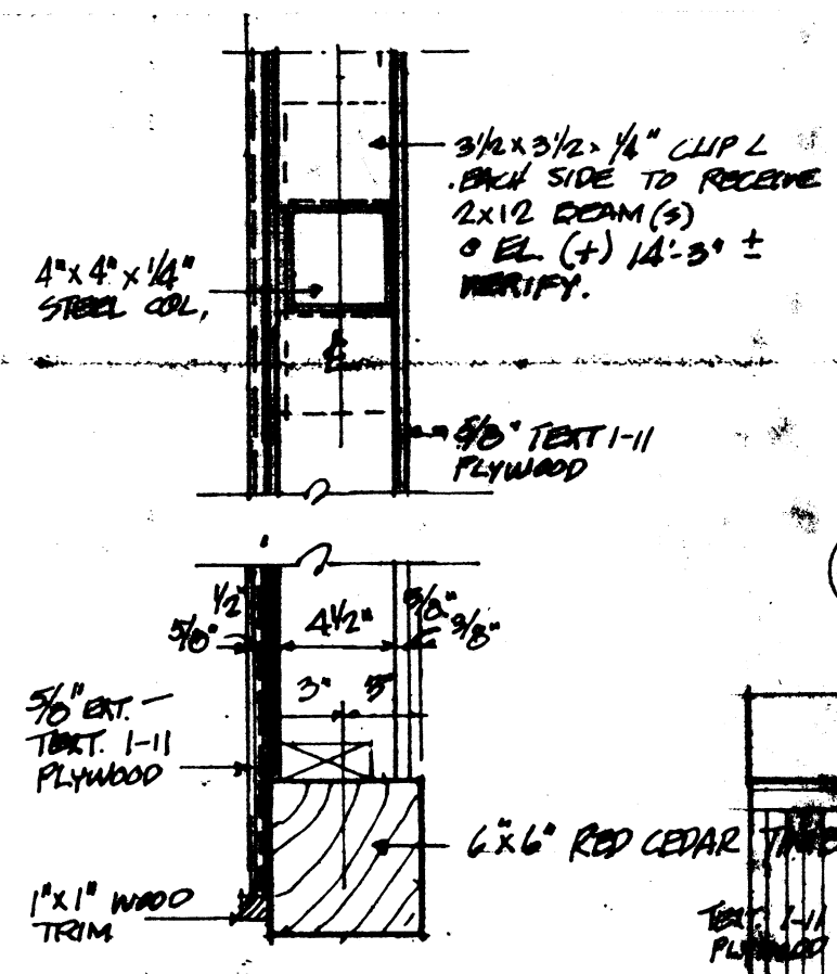
DETAIL 20 PLAN VIEW SCALE 1/2" = 1'-0"
