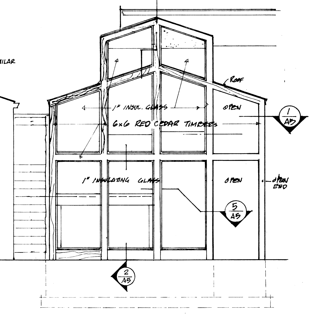
ELEVATION 9 SCALE 1/4" = 1'-0"
