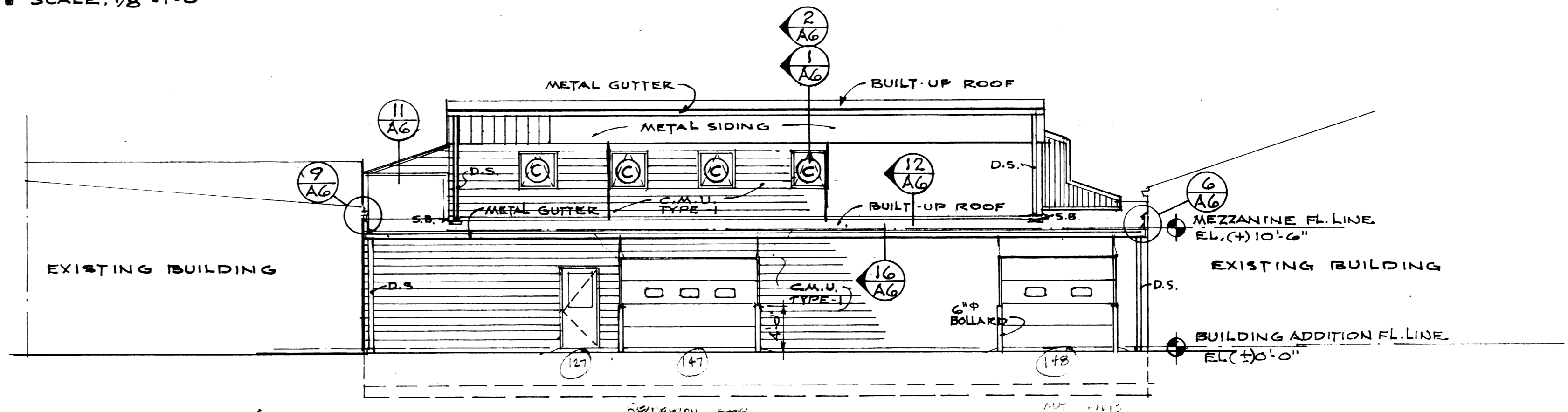
6 PARTIAL EAST ELEVATION SCALE: 1/8" = 1'-0"
