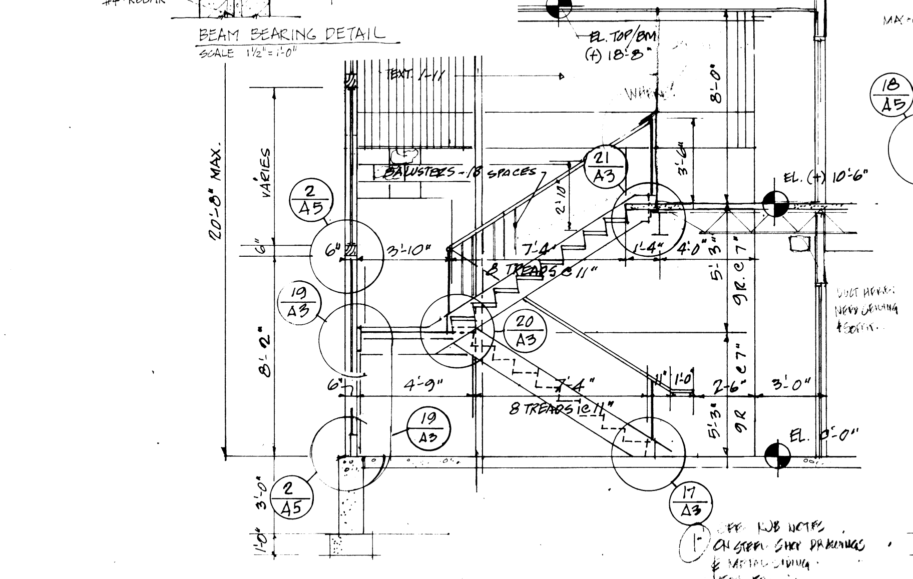
SECTION 17 SCALE 1/4" = 1'-0"
