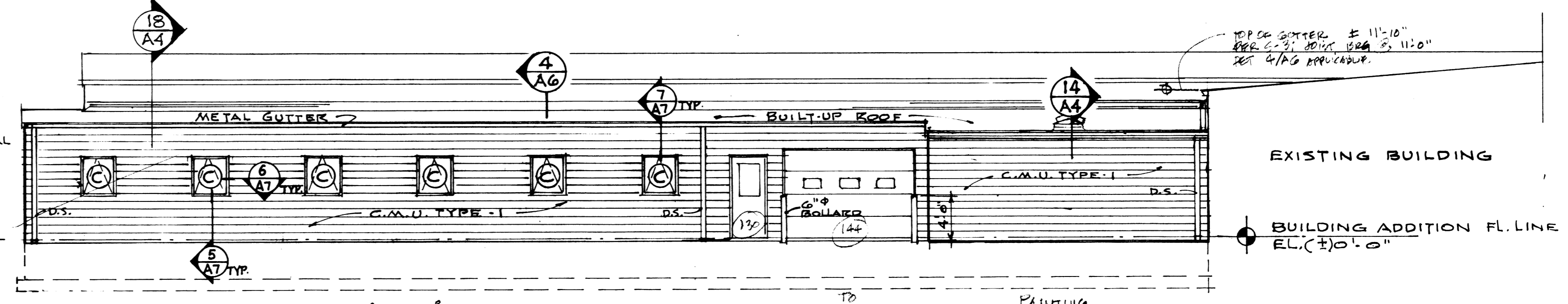
11 PARTIAL EAST ELEVATION SCALE: 1/8" = 1'-0"
