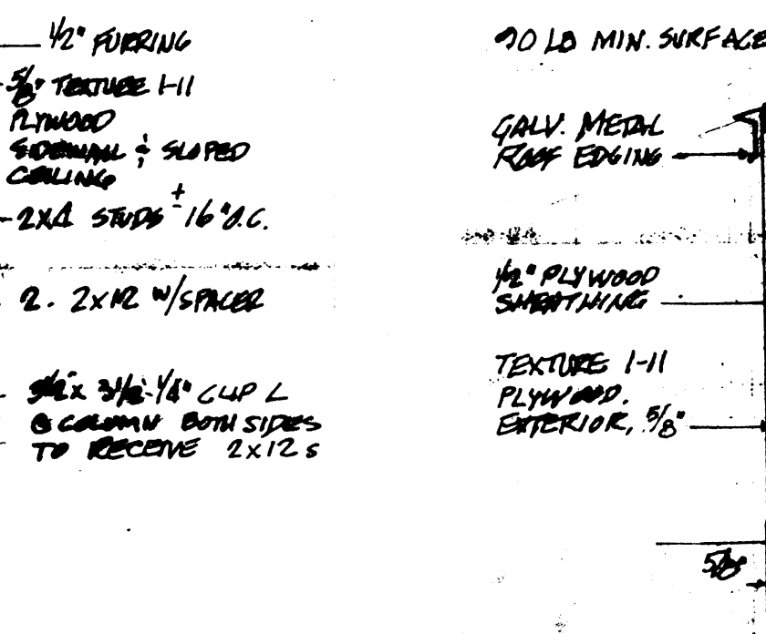
DETAIL 10 SCALE 1/2" = 1'-0"
