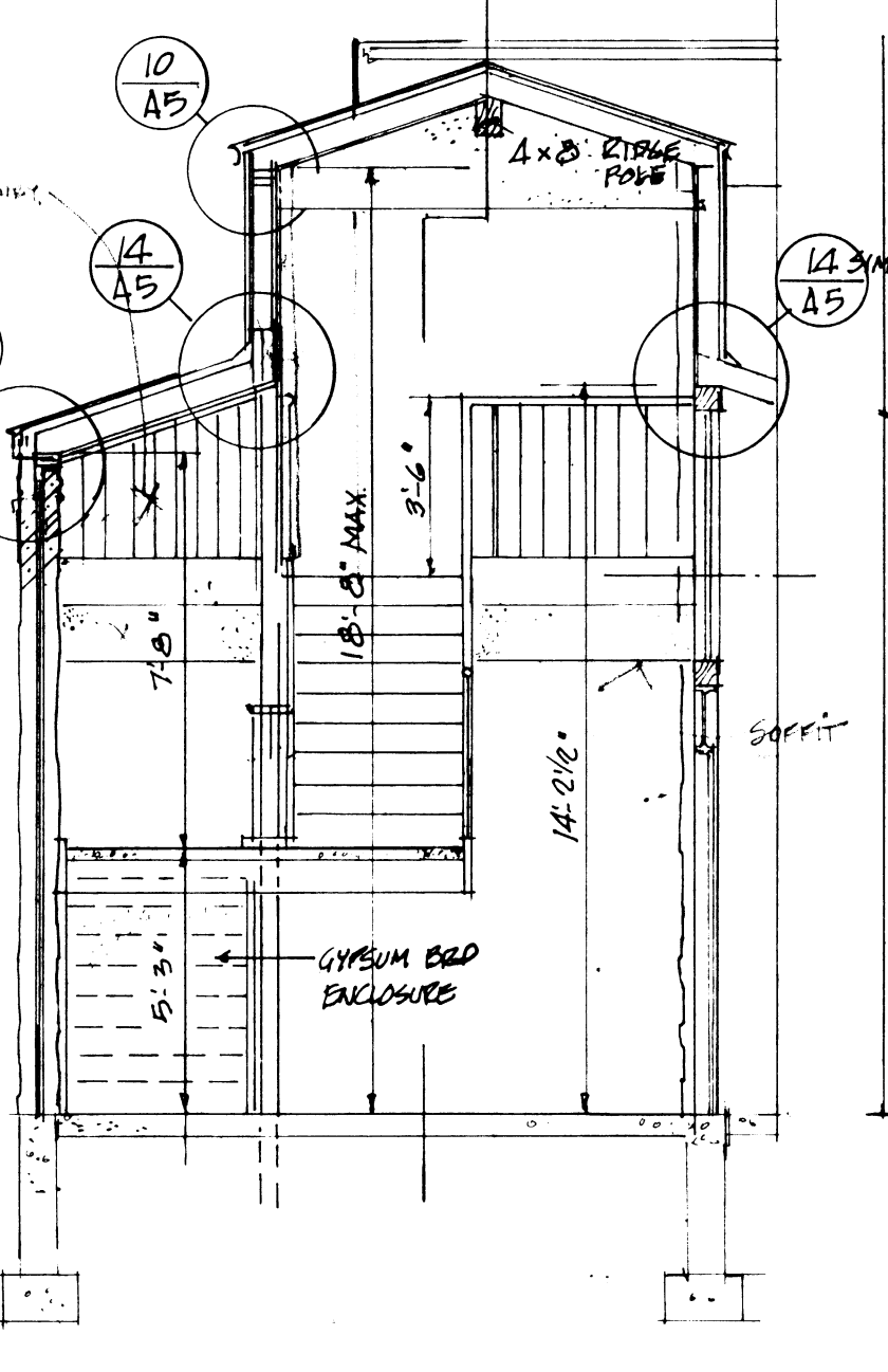
SECTION 13 SCALE 1/4" = 1'-0"
