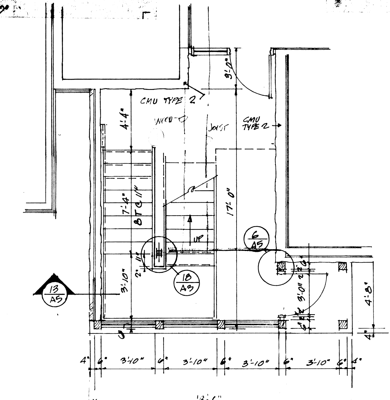
FIRST FLOOR STAIR PLAN 5 SCALE 1/8" = 1'-0"
