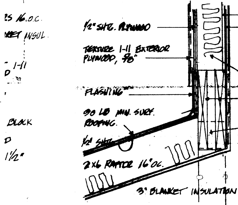
DETAIL 14 SCALE 1/2" = 1'-0"
