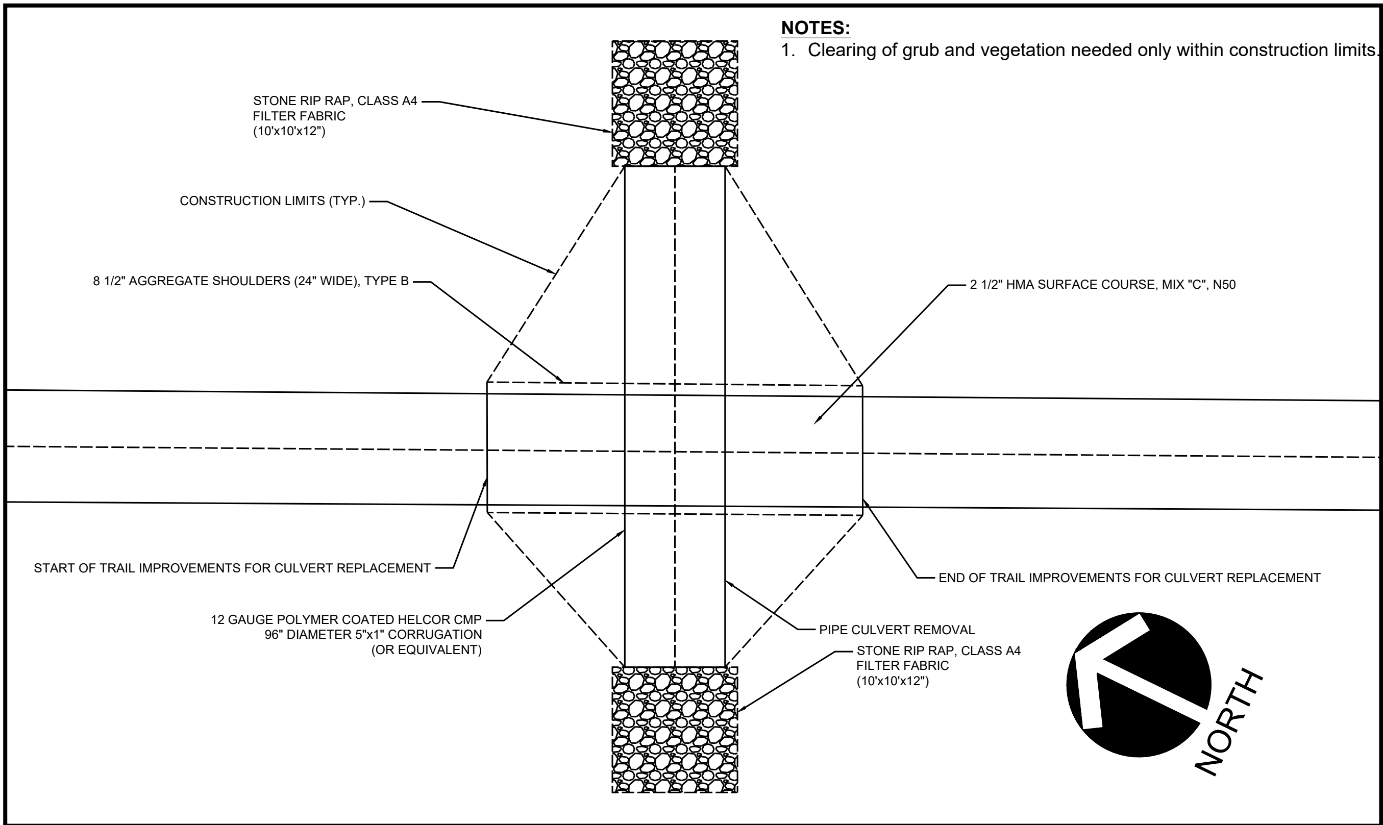
1 CULVERT/PATH PLAN VIEW 1" = 10'
