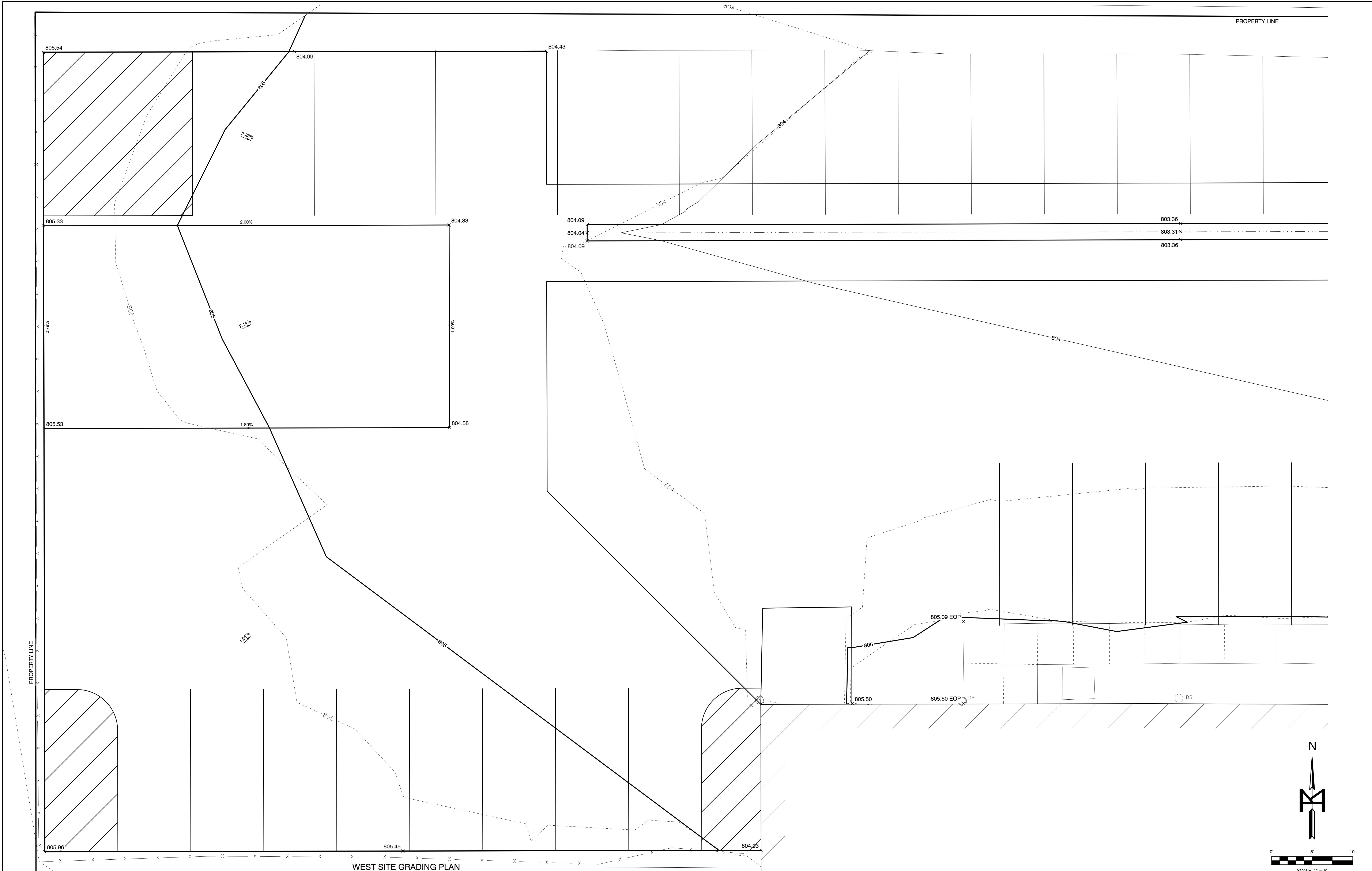
WEST SITE GRADING PLAN SCALE: 1" = 5'
