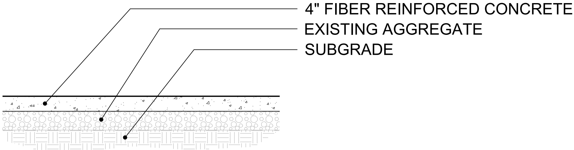
2 Alternate "B" Concrete Path 6 NOT TO SCALE
