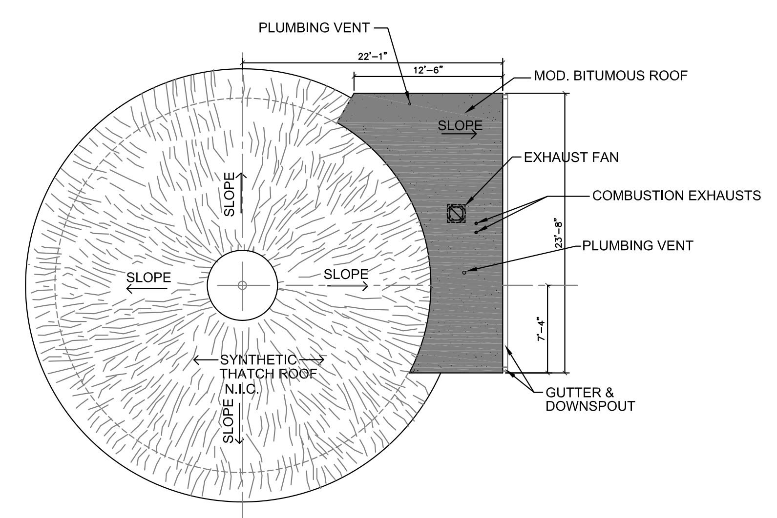
2 Existing / Revised Small Animals House Roof Plan RF3 1/8" = 1'-0"
