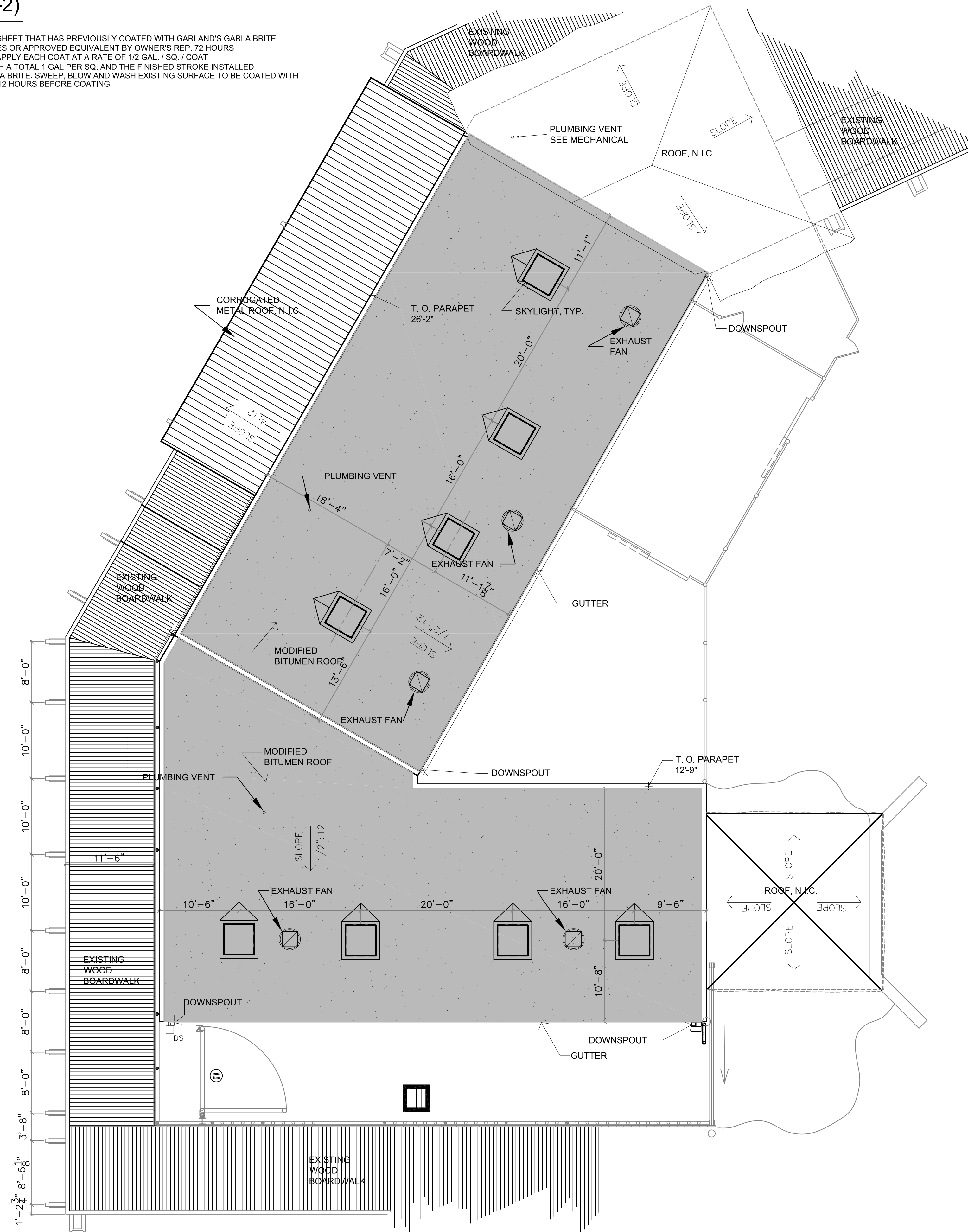
1 Existing / Revised North Night House Roof Plan RF1 1/8" = 1'-0"
