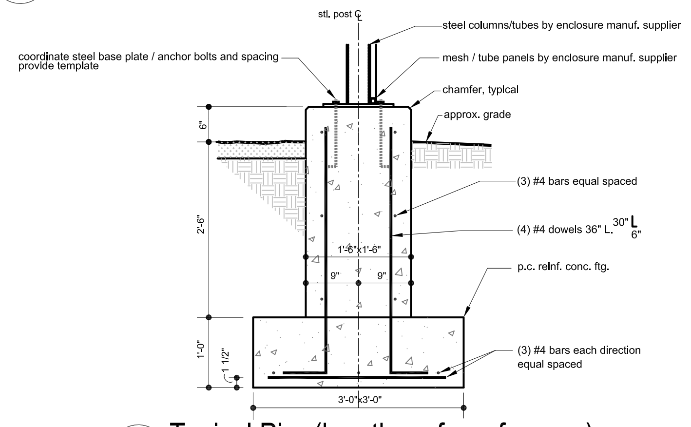
4 Typical Pier (by others for reference) A2 1" = 1'-0"
