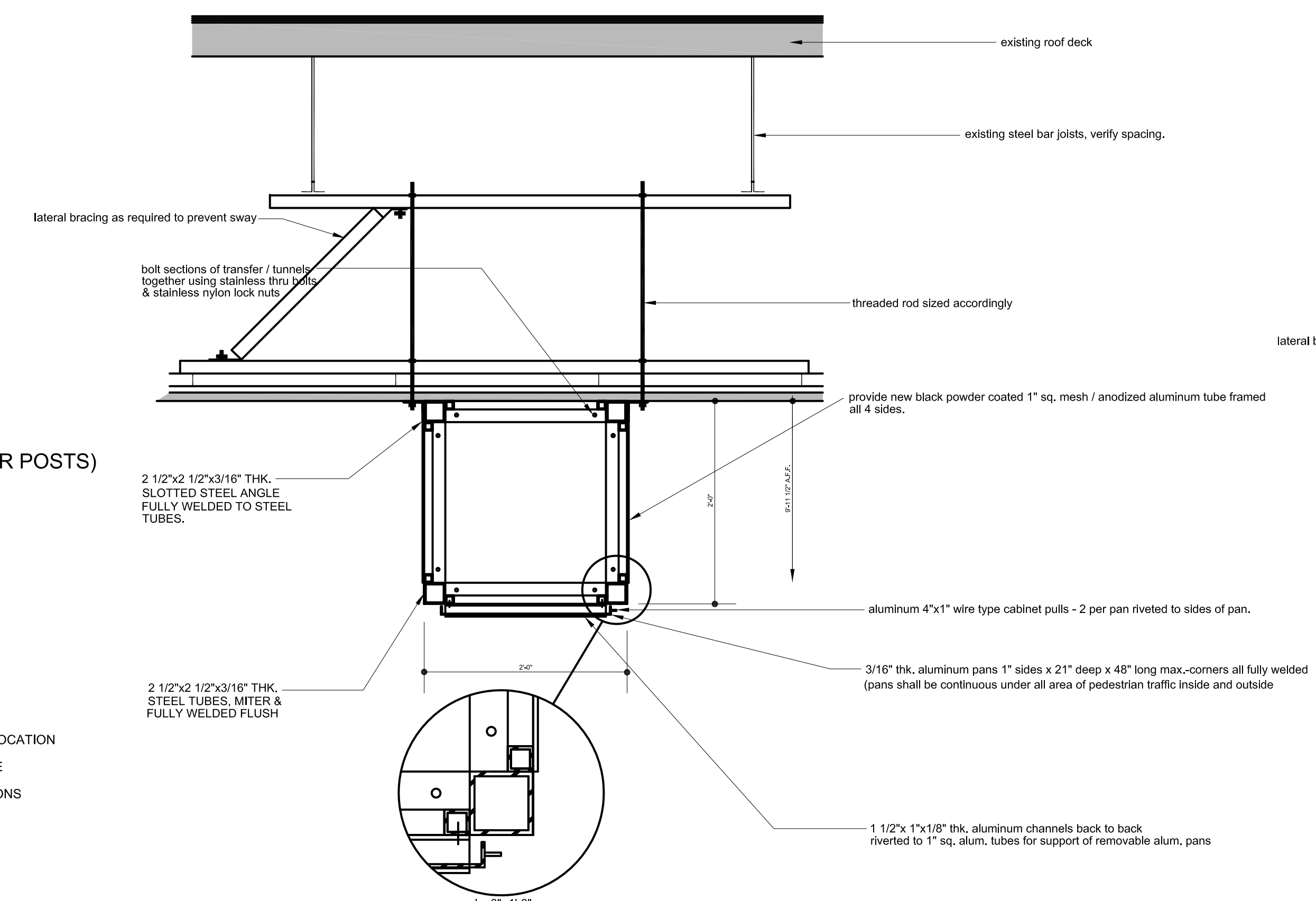
2 Detail Section Thru Transfer / Tunnel Ceiling A2 1" = 1'-0"
