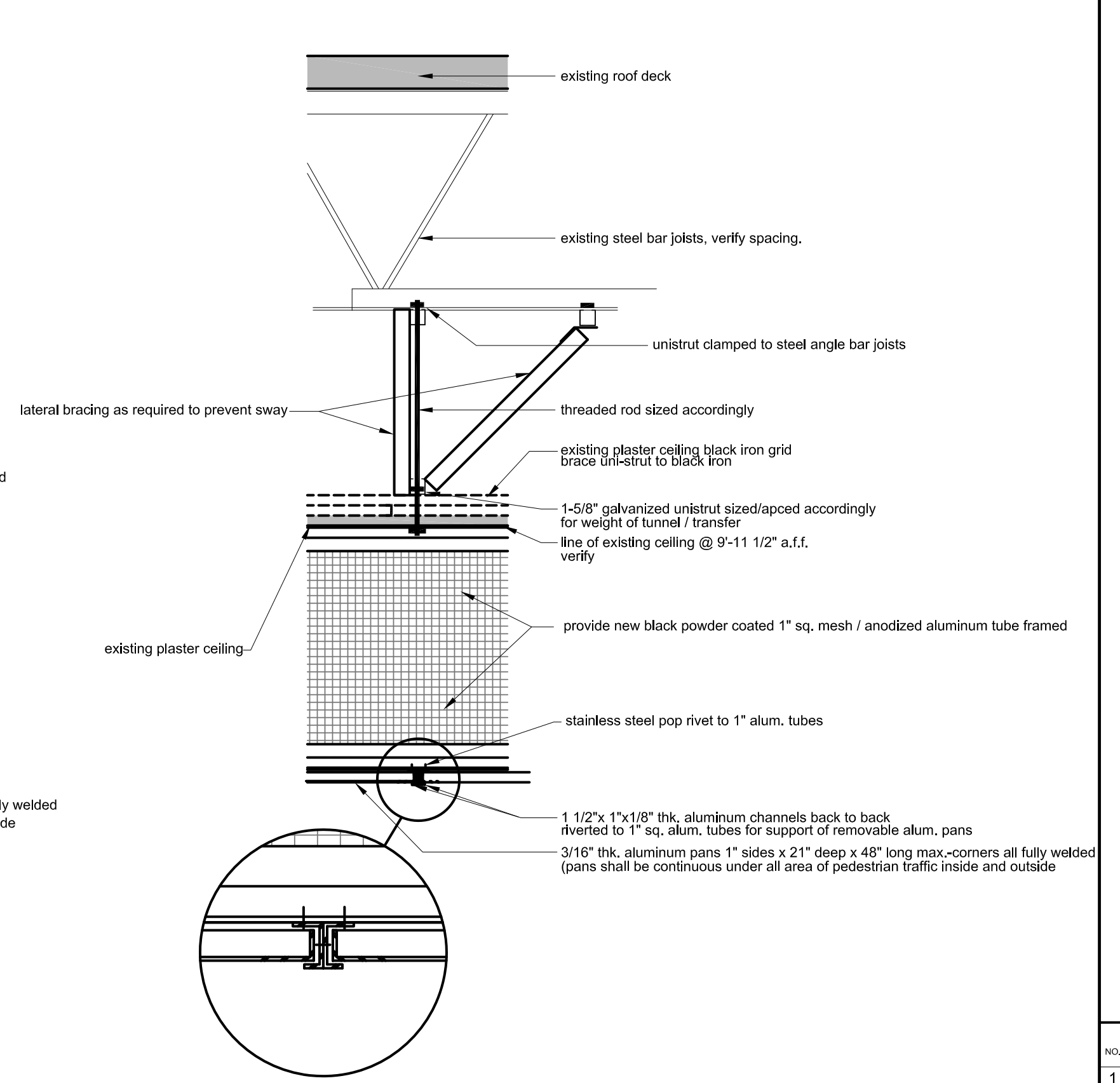
3 Detail Section Elevation Thru Transfer / Tunnel Ceiling A2 1" = 1'-0"
