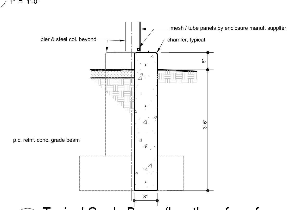
5 Typical Grade Beam (by others for reference) A2 1" = 1'-0"
