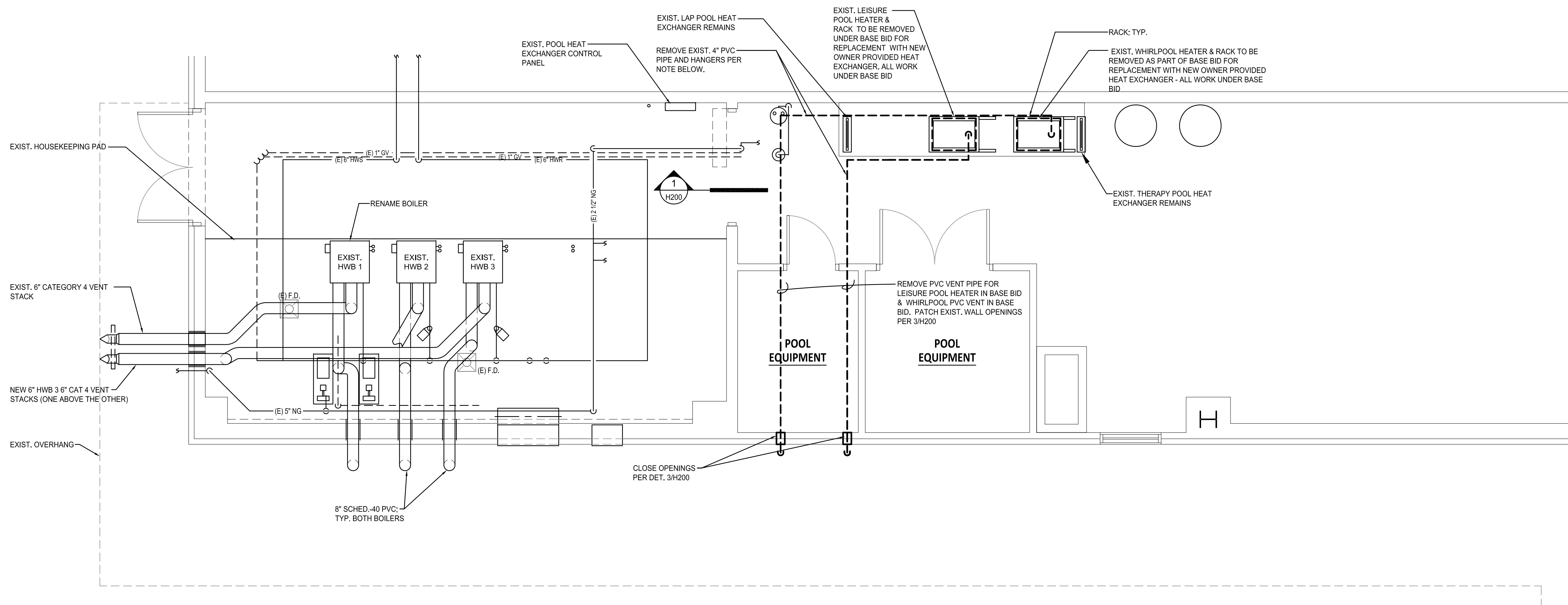
2 Vent Pipe Pool Heater Plan - Demolition / Revised H100 scale: 1/4" = 1'-0"
