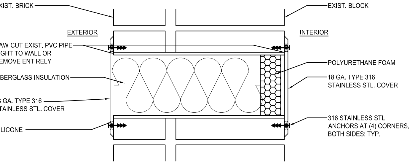
3 Existing Opening Finish Cover Detail H200 not to scale
