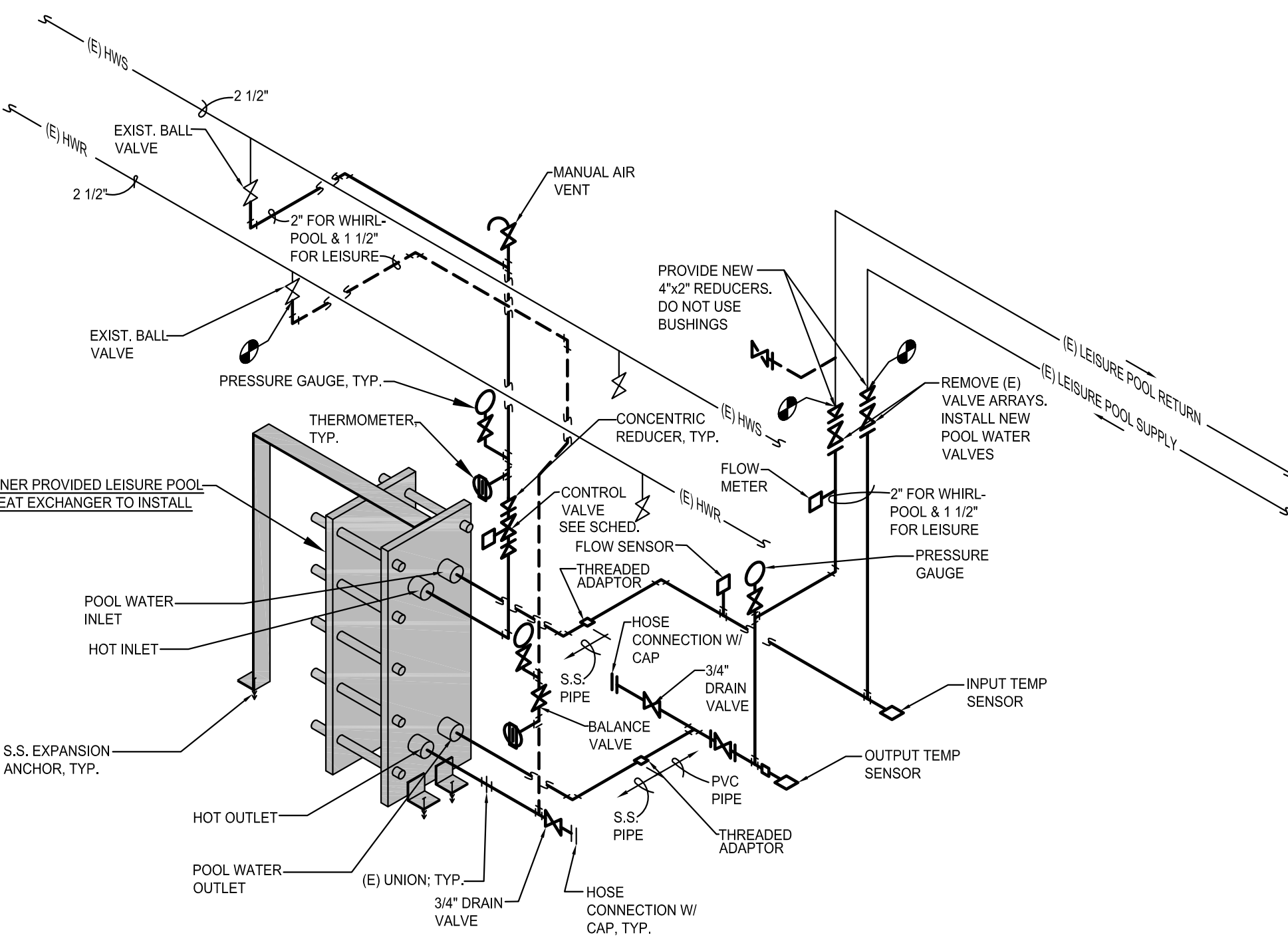
2 Leisure Pool Heat Exchanger Schematic (Whirlpool Sim.) (Both Base Bid) H200 not to scale
