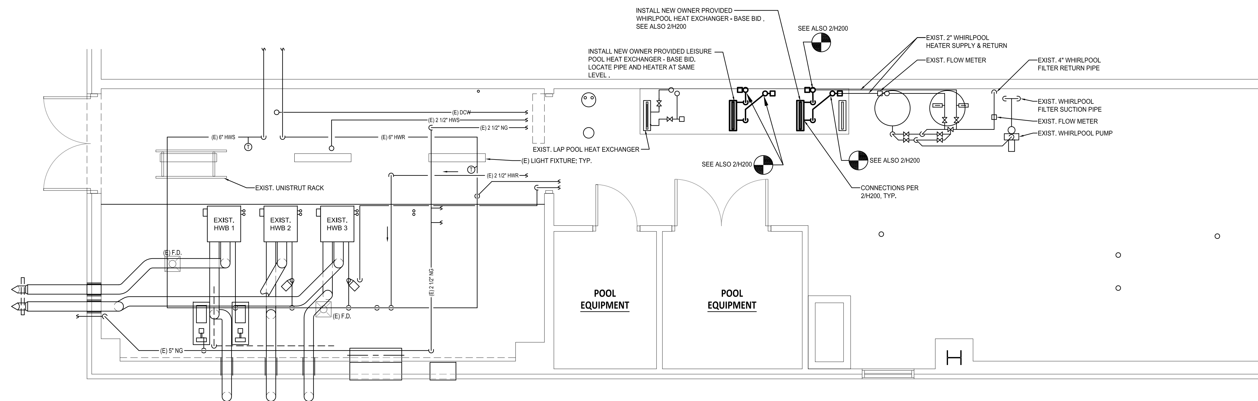
2 Lower Level Water Piping Plan - Revised H101 scale: 1/4" = 1'-0"
