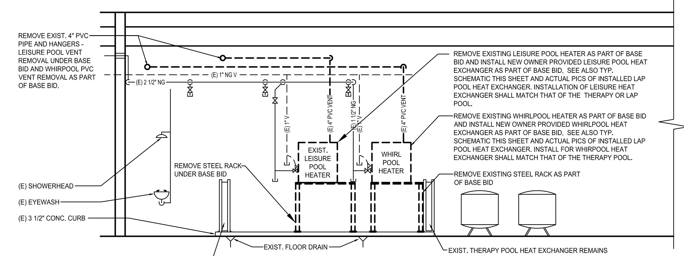
1 Section - Looking West H200 scale: 1/4" = 1'-0"
