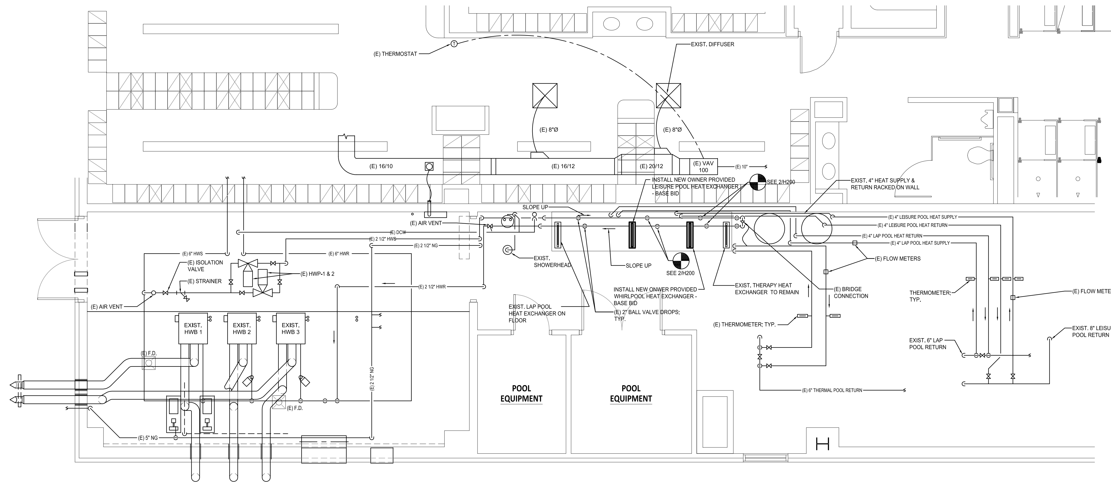
1 Upper Level Water Piping Plan - Revised H101 scale: 1/4" = 1'-0"
