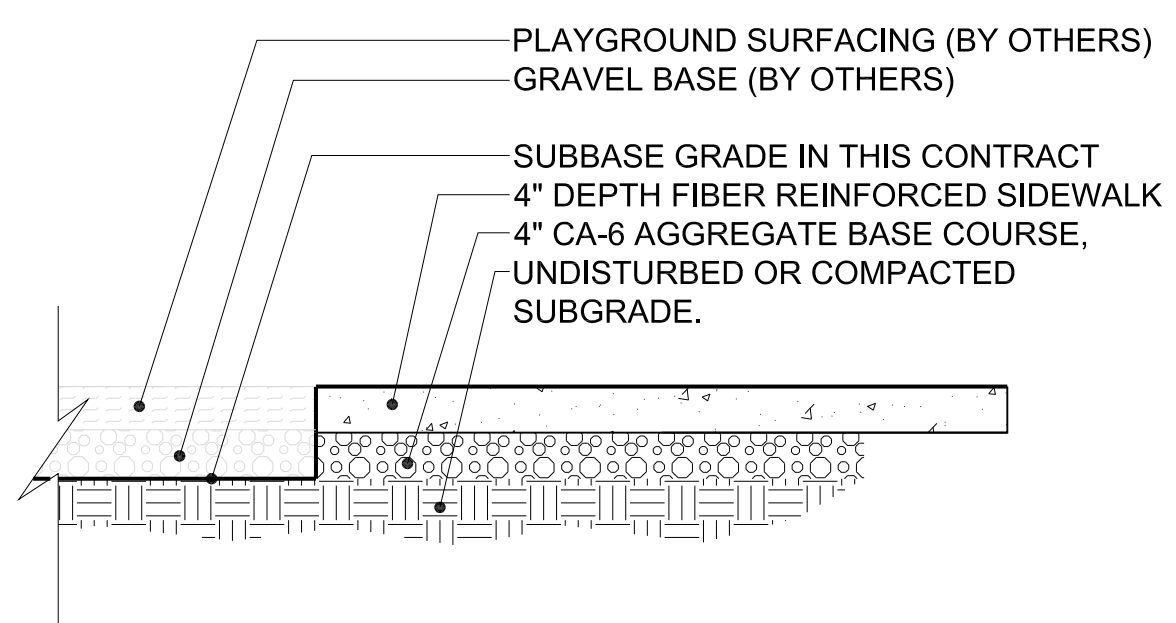
1 Walk/Playground Edge Transition 5 NOT TO SCALE
