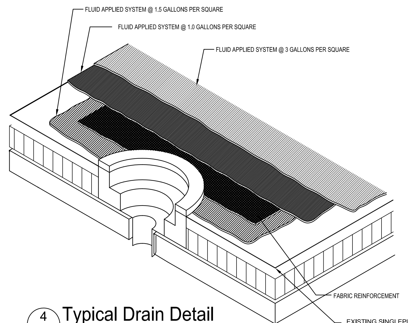
4 Typical Drain Detail
