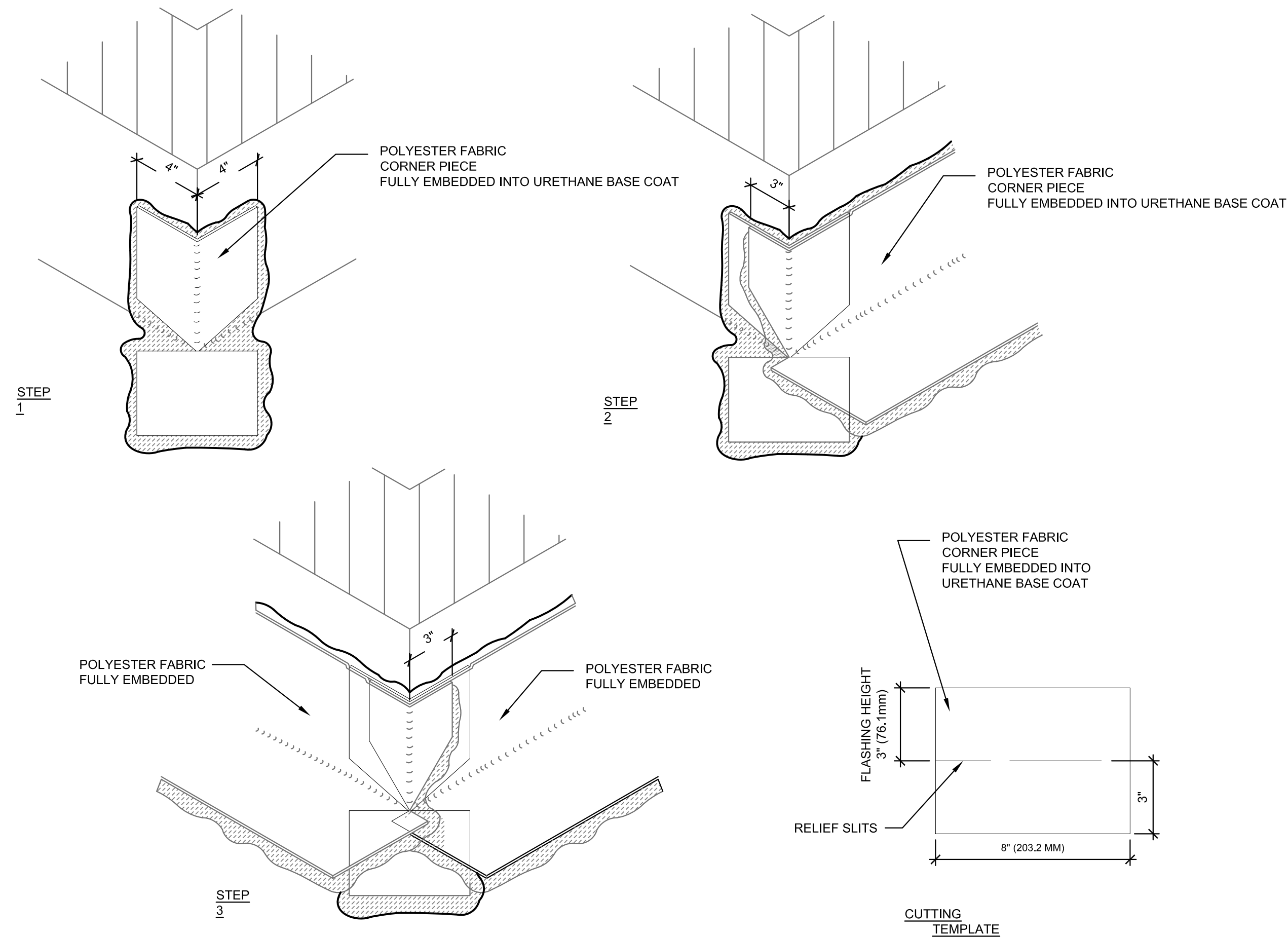
2 Typical Outside Corner Detail (inside similar)
