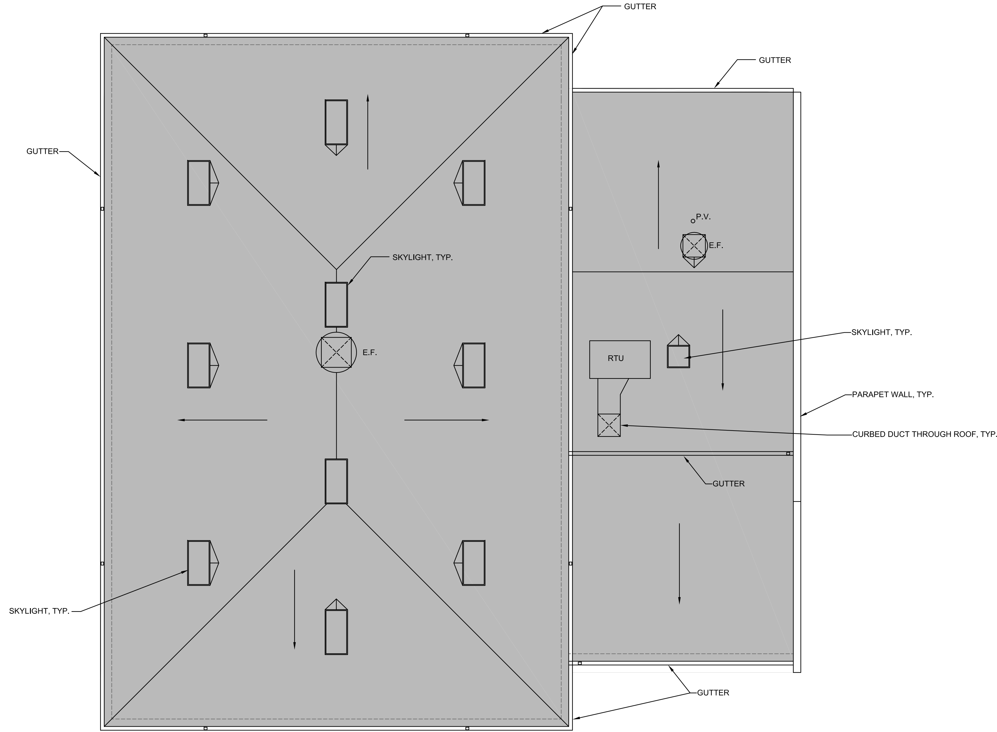
1 ROOF PLAN
