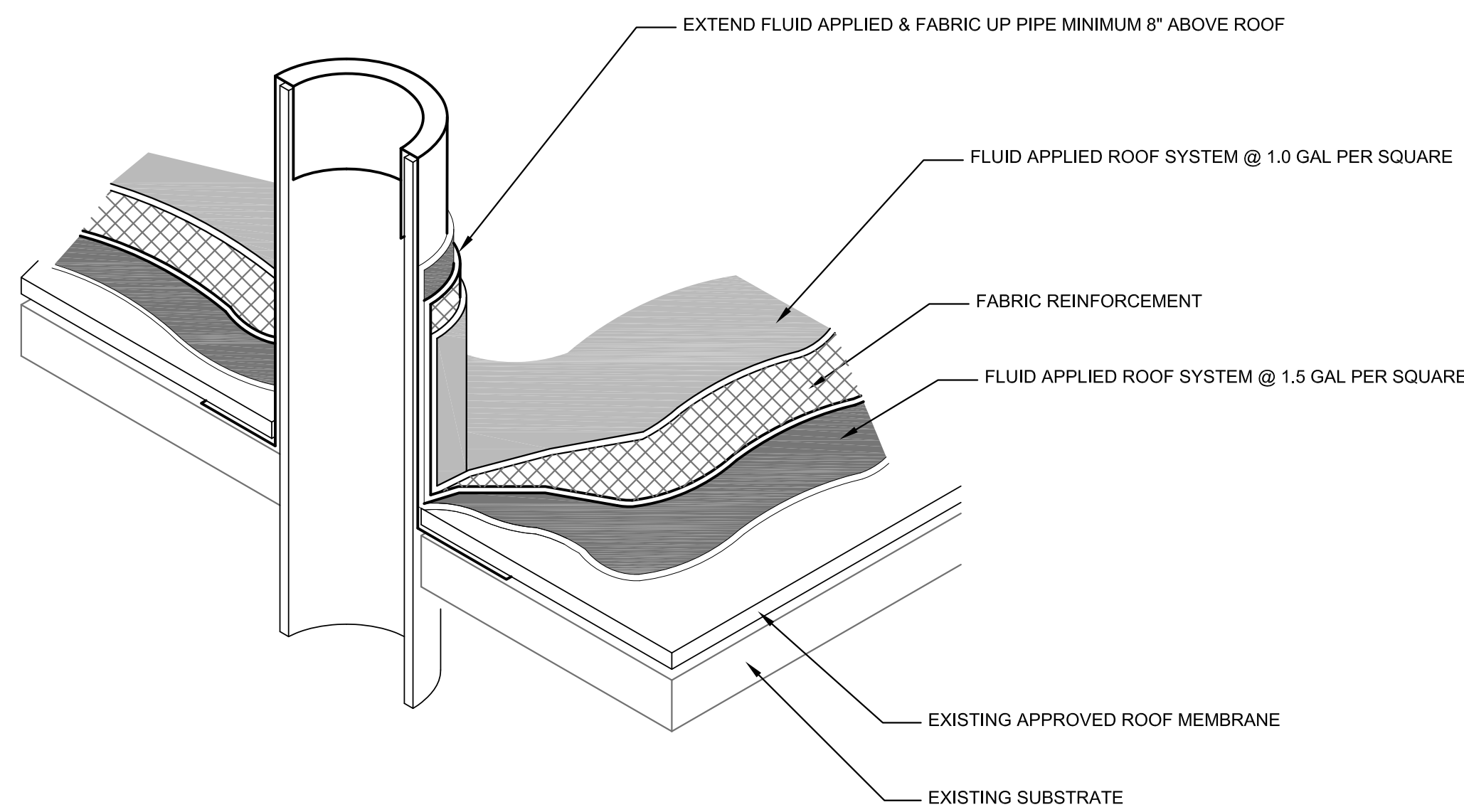
3 Typical Pipe Penetration Detail
