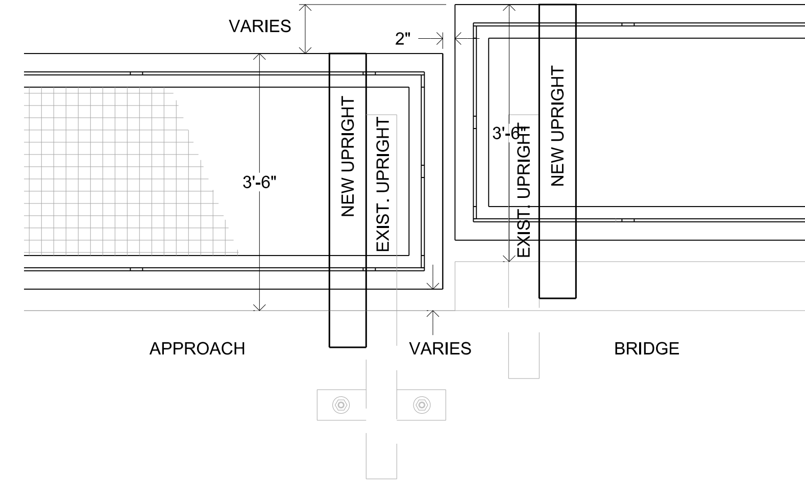
6 3 Approach and Bridge Junction - Elevation 3/4" = 1'-0"
