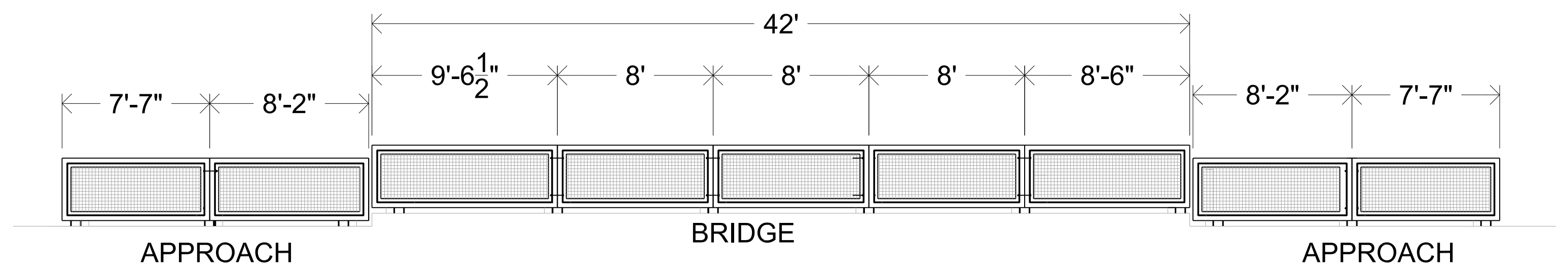
2 Panel Lengths 2 1" = 5'-0"
