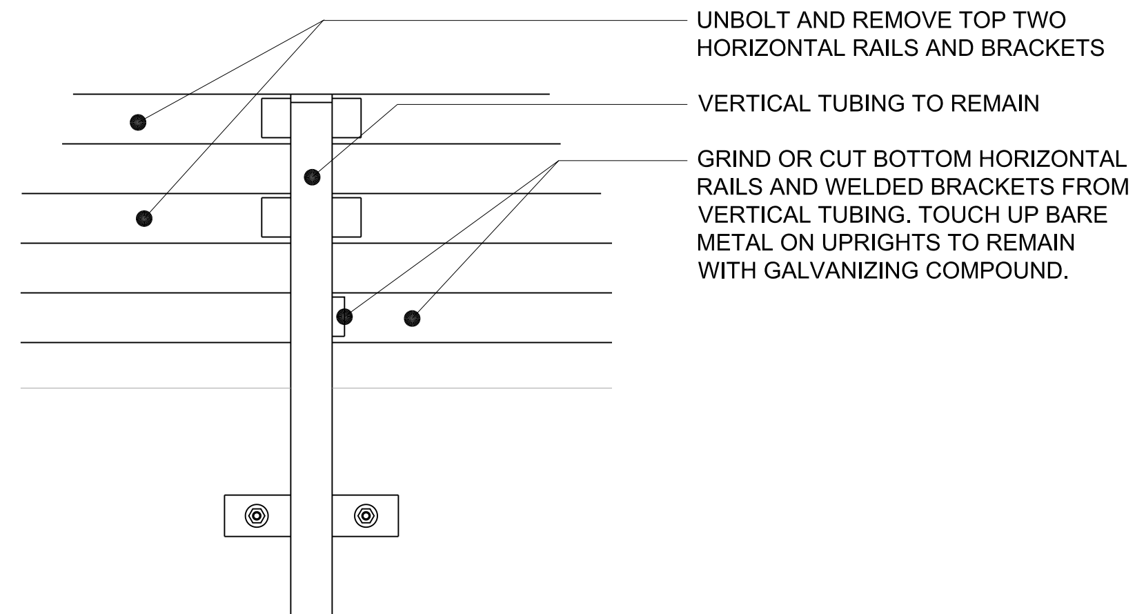
4 Demolition - Angled Approach Railing 2 3/4" = 1'-0"
