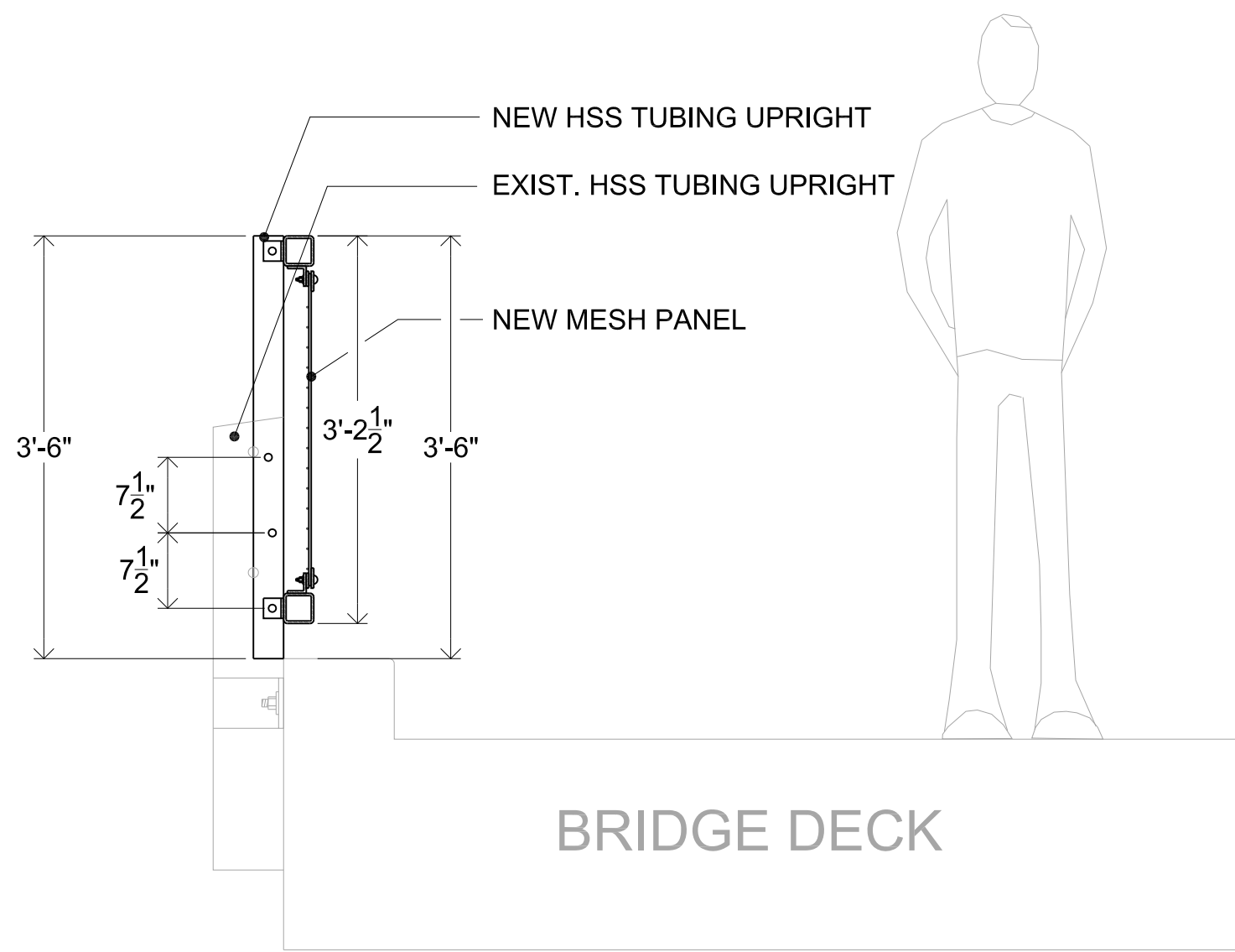
1 3 Bridge Railing - Section 3/4" = 1'-0"
