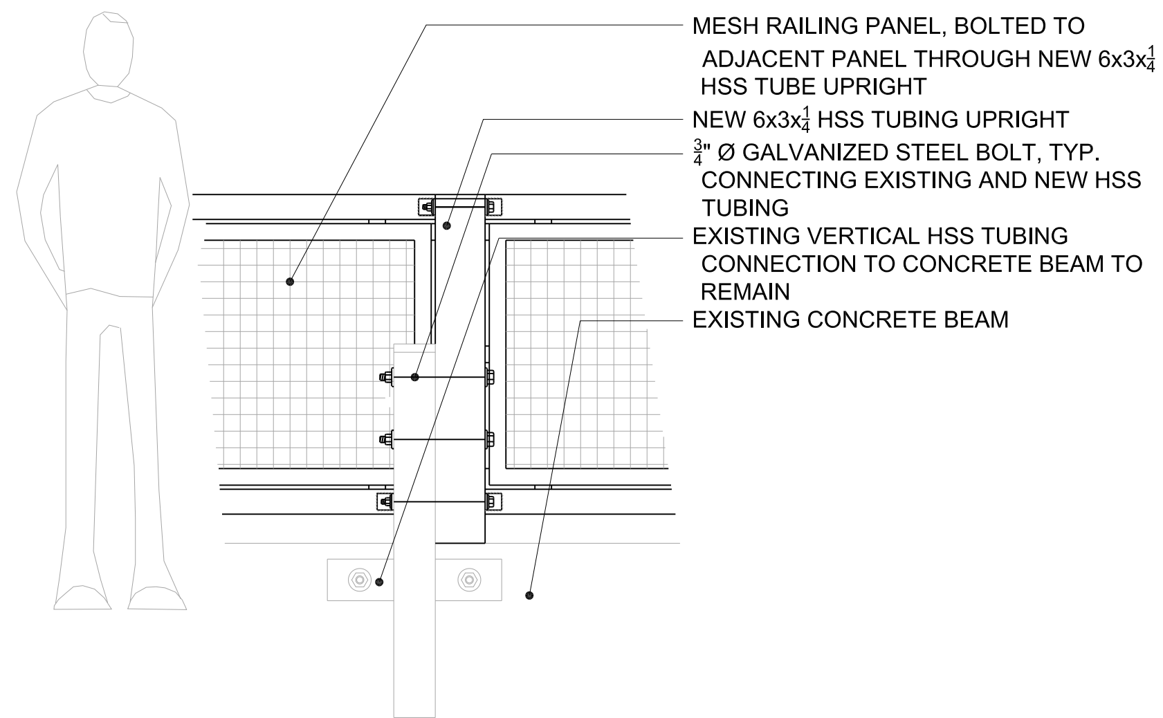
2 3 Bridge Railing - Elevation 3/4" = 1'-0"
