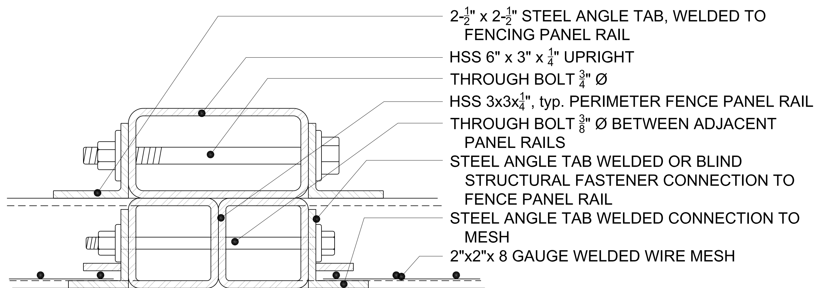
5 3 Panel to Upright Connection Detail 1/2" = 1'-0"
