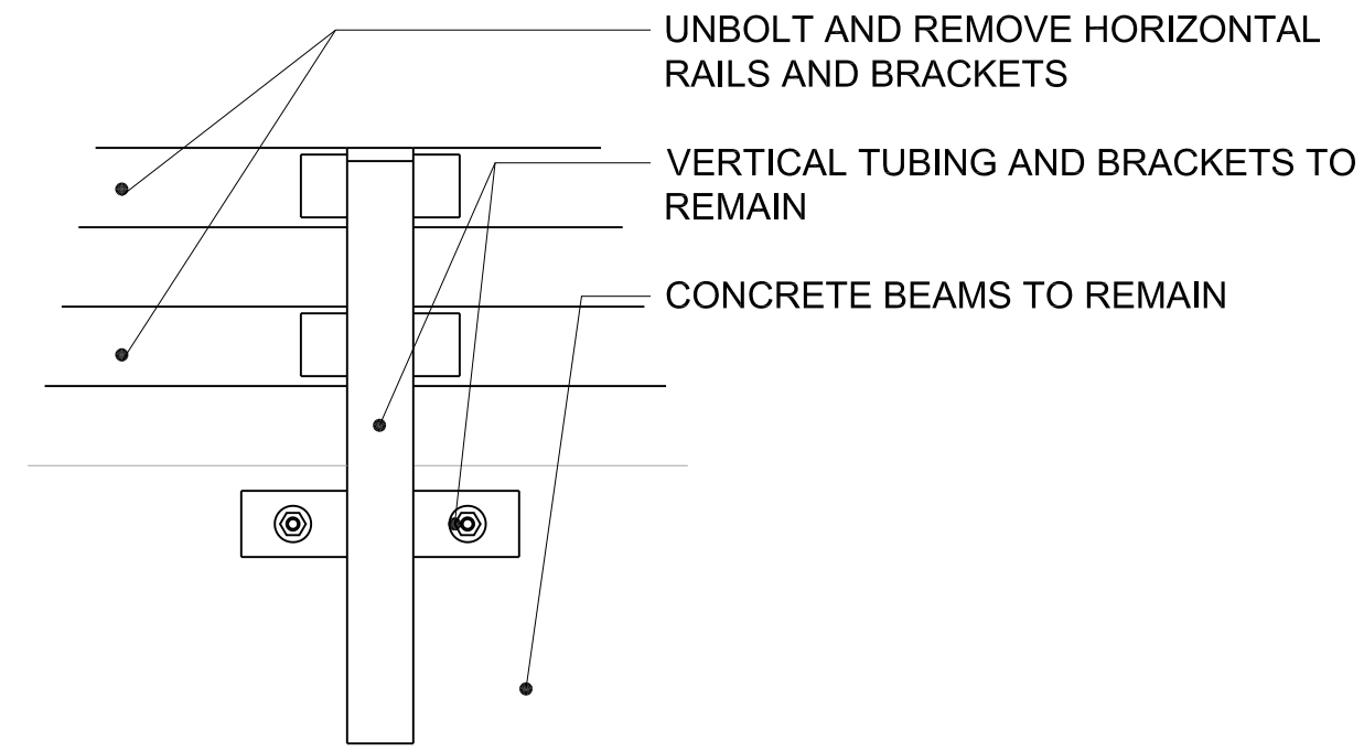
3 Demolition - Bridge Railing 2 3/4" = 1'-0"
