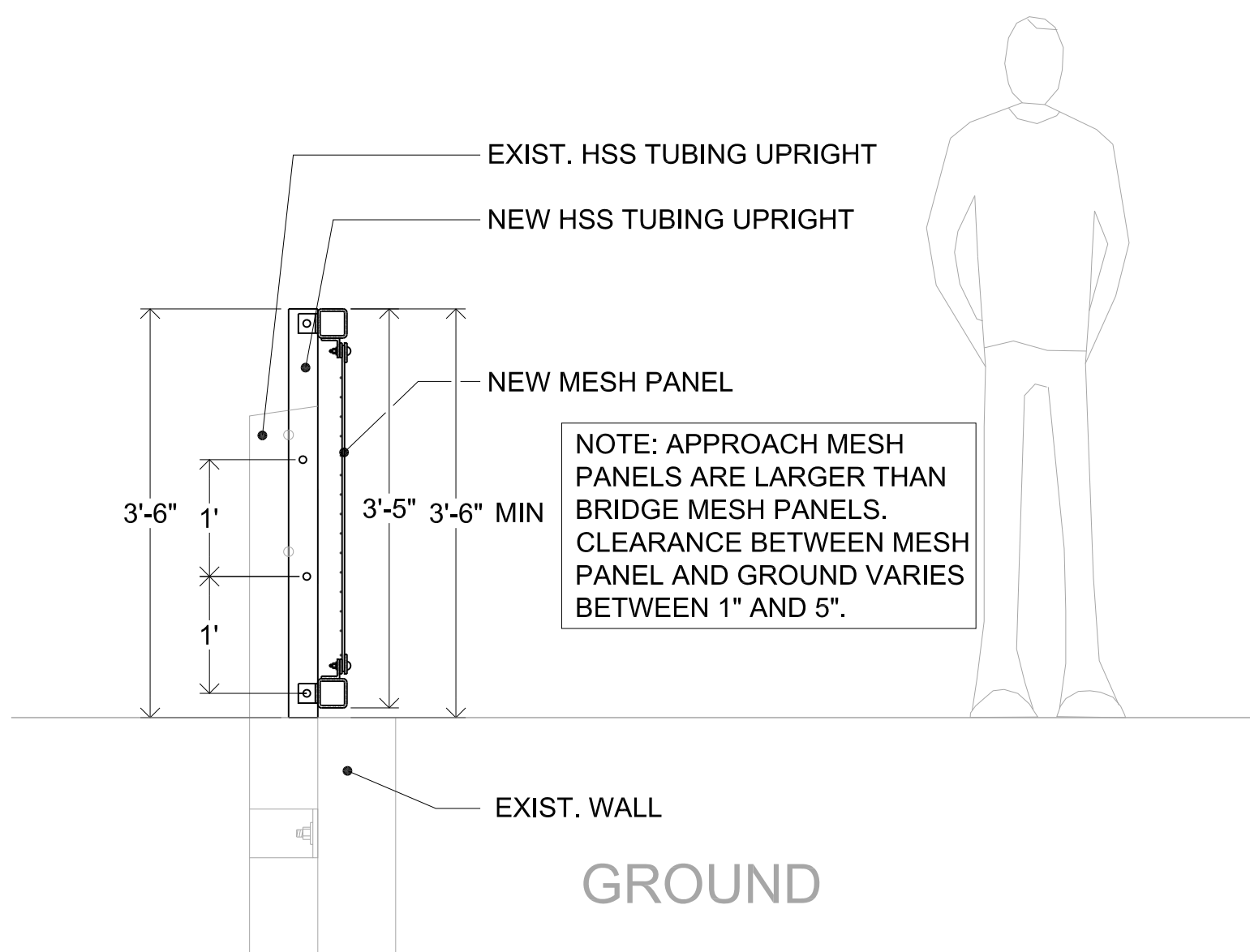
3 3 Approach Railing - Section 3/4" = 1'-0"
