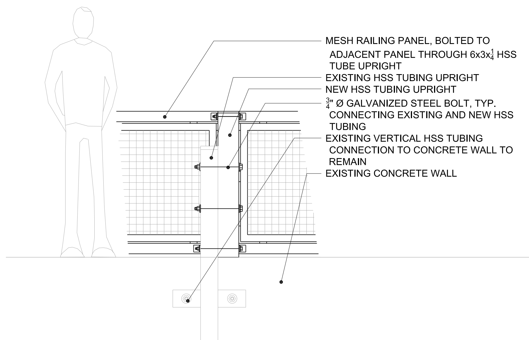
4 3 Approach Railing - Elevation 3/4" = 1'-0"
