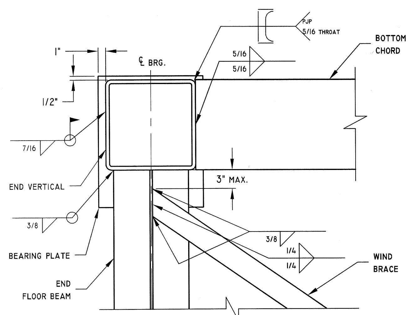
7 WIND BRACE/END FLOOR BEAM CONNECTION SCALE: 1 1/2" = 1' 0"
