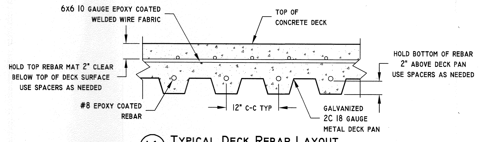
16 TYPICAL DECK REBAR LAYOUT SCALE: NTS
