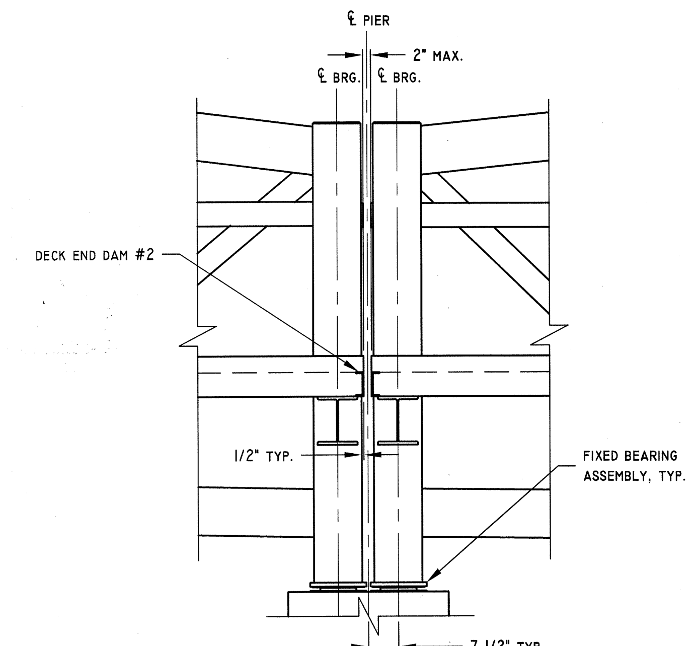
14 TRUSS ELEVATION @ PIER SCALE: 1/2" = 1' 0"
