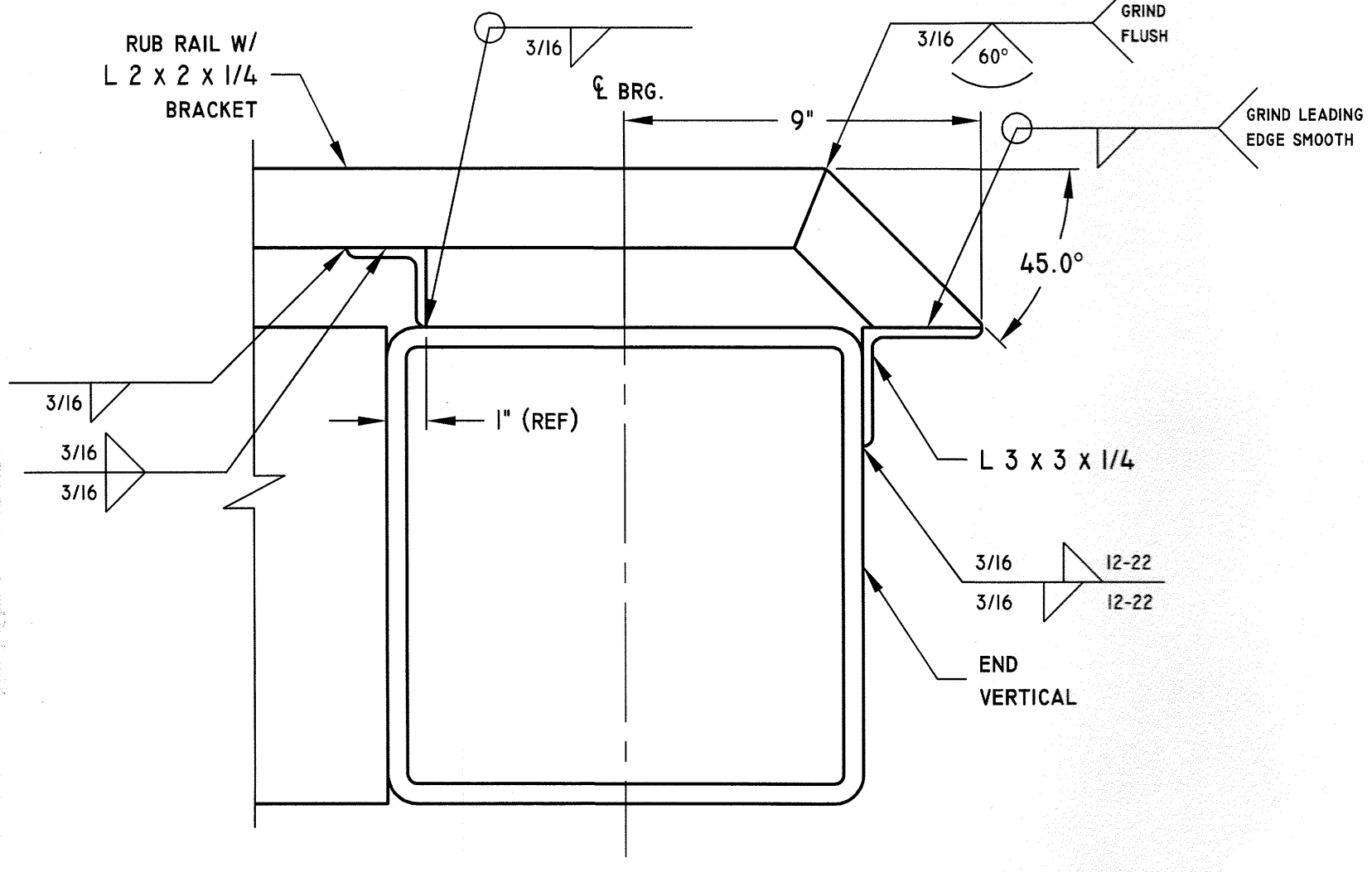
15 TYPICAL RUB RAIL CONNECTION @ ABUTMENT (EXP) SCALE: NTS
