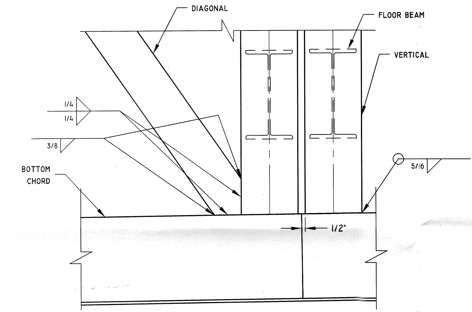
10 DIAGONAL/BOTTOM CHORD CONNECTION DETAIL SCALE: 1 1/2" = 1' 0"
