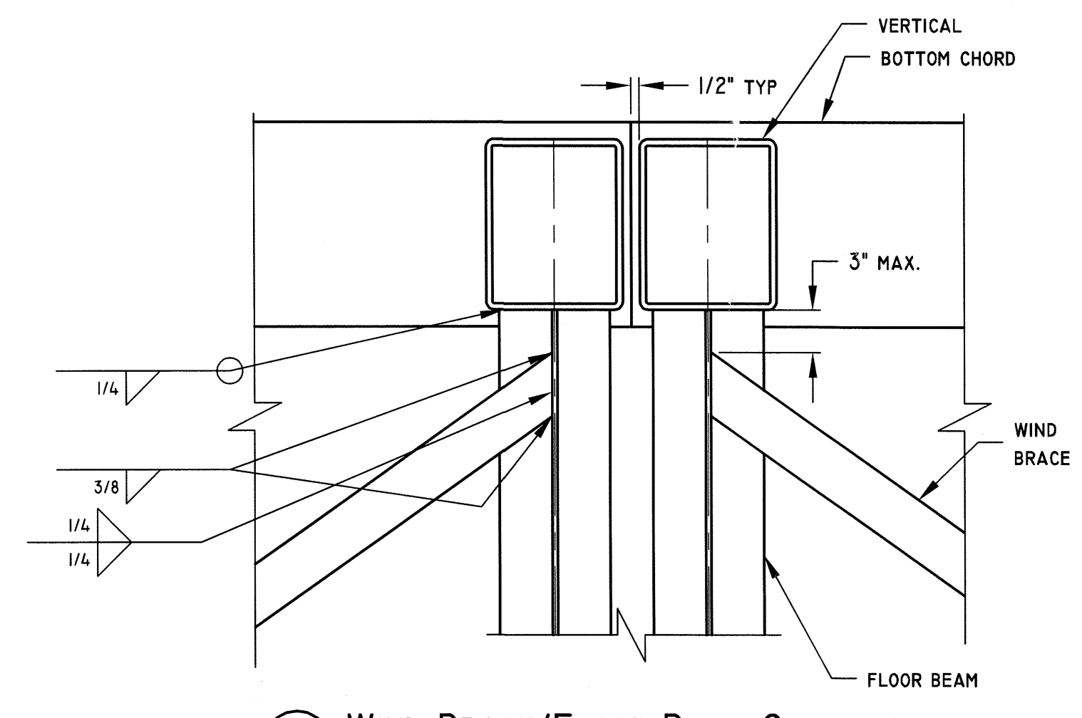
8 WIND BRACE/FLOOR BEAM CONNECTION SCALE: 1 1/2" = 1' 0"
