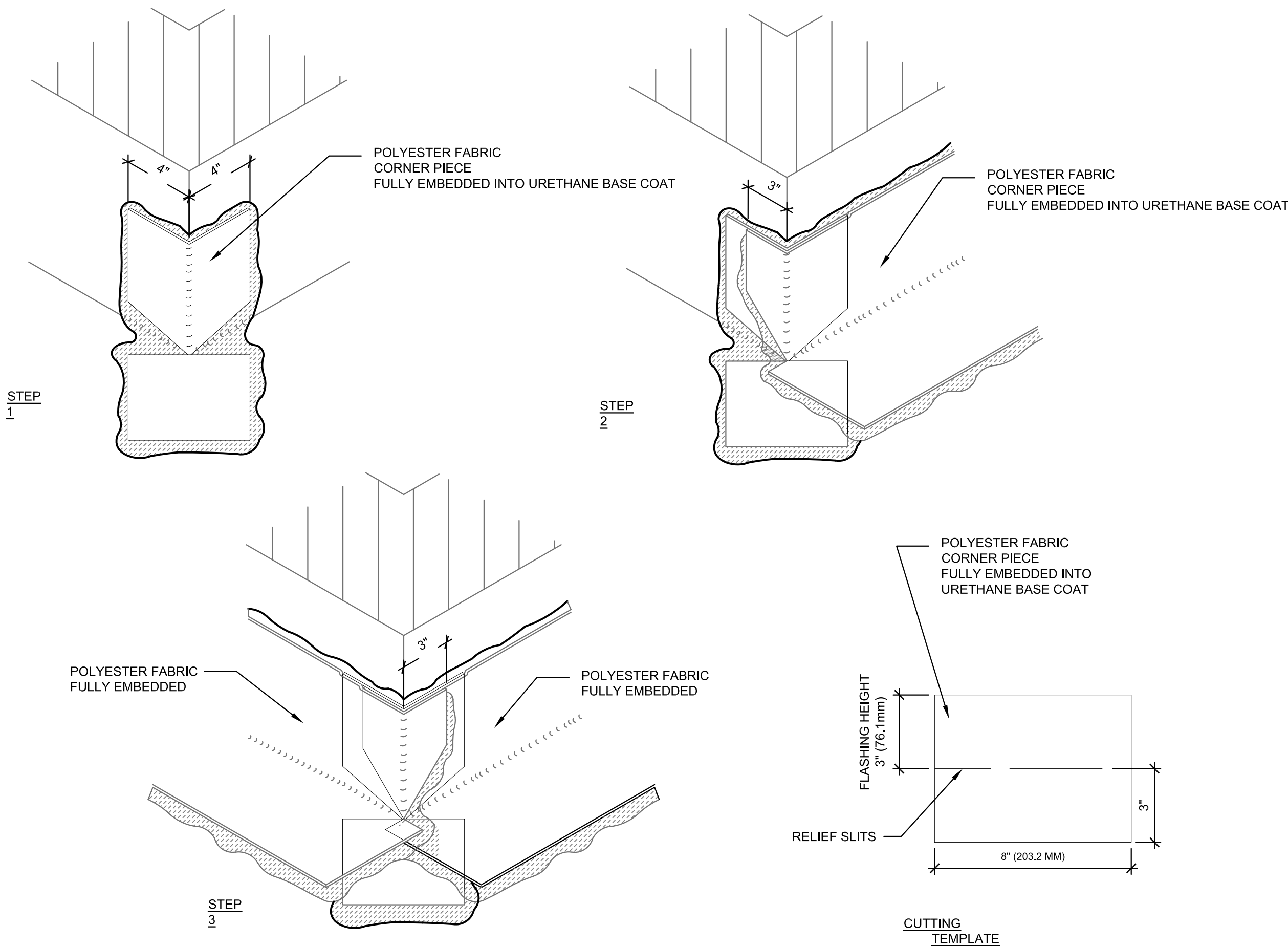
1 Typical Outside Corner Detail (inside similar)
