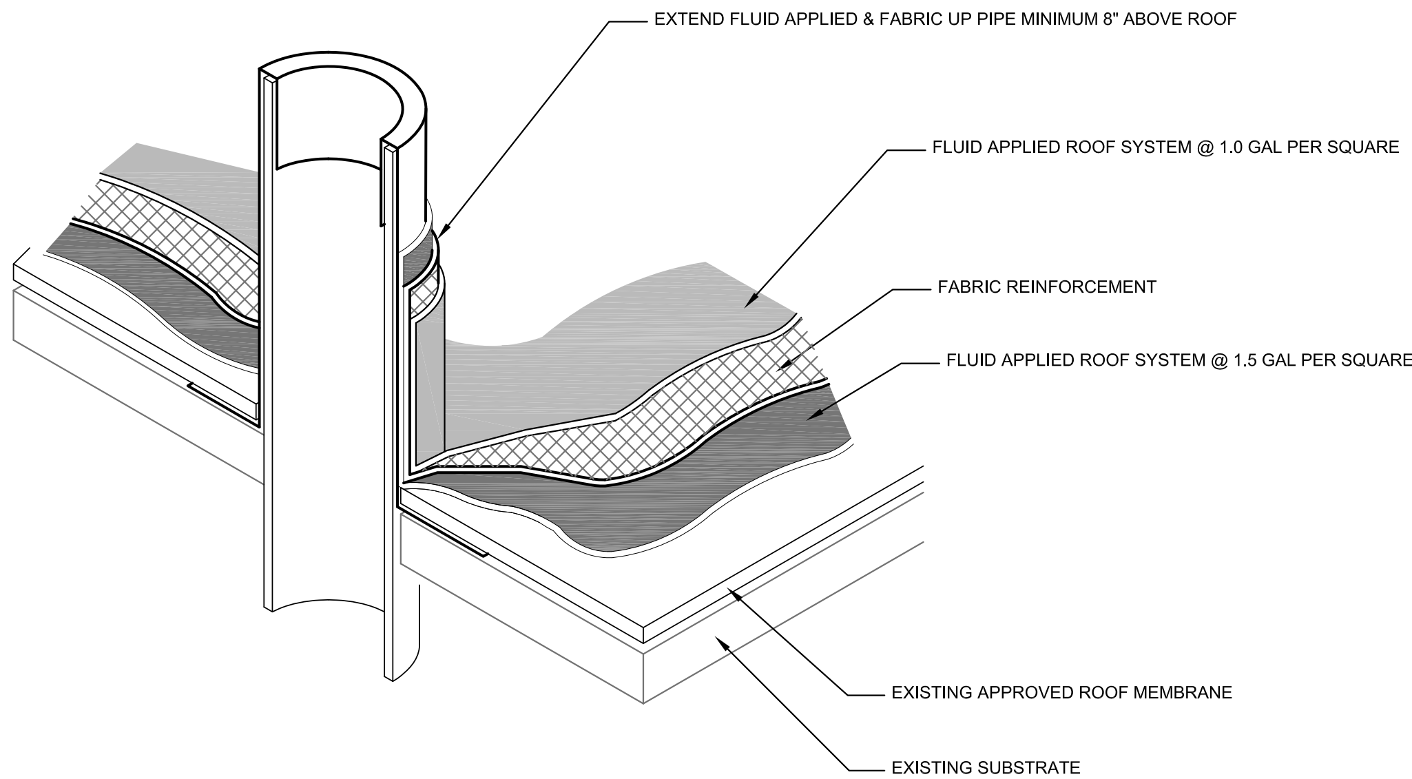
2 Typical Pipe Penetration Detail
