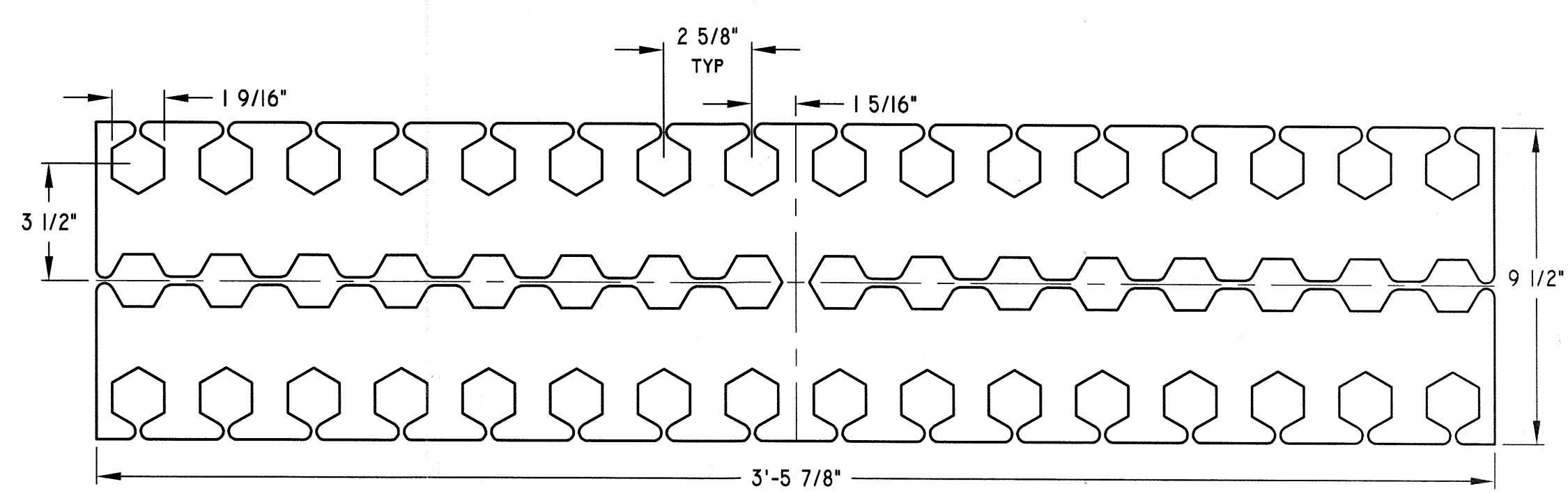
CHORD SPLICE SOCKET - SS SCALE: 3" = 1' 0" MAT'L: 3/16 PLATE PIECES REQ'D: 32
