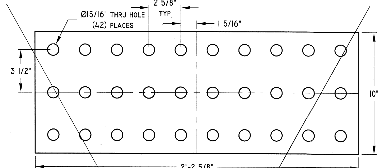
BOTTOM CHORD SPLICE PLATE - SP-2 SCALE: 3" = 1' 0" MAT'L: 1/2 PLATE PIECES REQ'D: N/A
