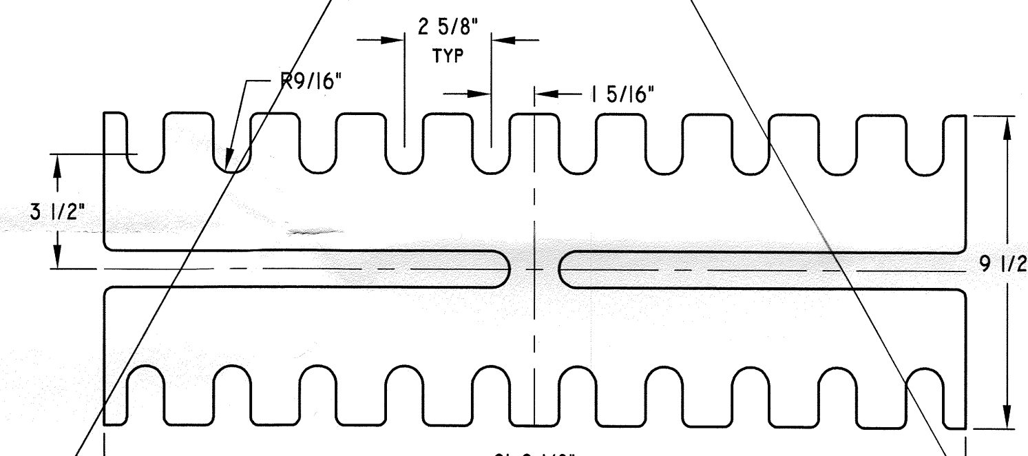
TOP CHORD SPLICE RETAINER - SR-1 SCALE: 3" = 1' 0" MAT'L: 3/16 PLATE PIECES REQ'D: N/A
