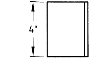
RUB RAIL BRACKET - RB-1 SCALE: 3" = 1' 0" MAT'L: 3 x 3 x 1/4 ANGLE PIECES REQ'D: 100
