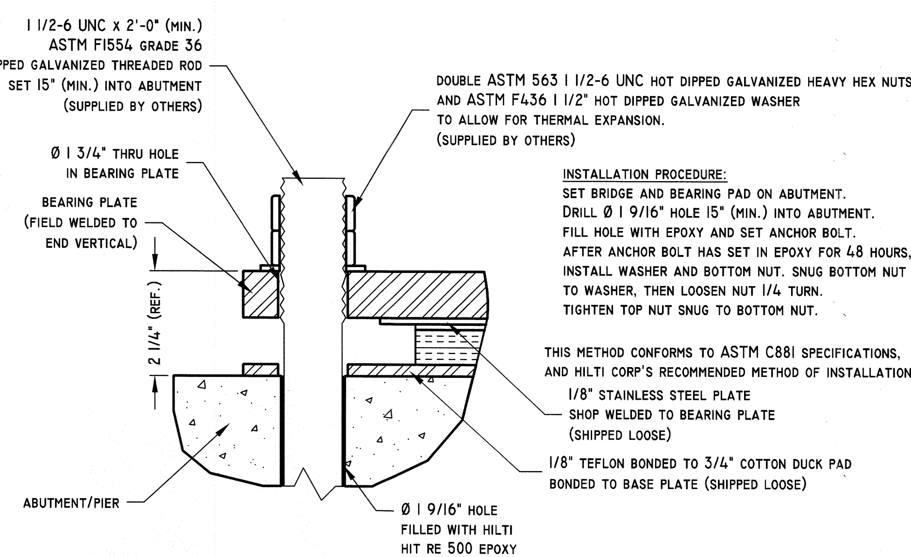
20 TYPICAL ANCHOR BOLT INSTALLATION DETAIL BRIDGE SPANS OVER 150 FT.
