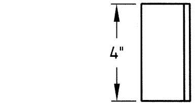
RUB RAIL BRACKET - RB-2 SCALE: 3" = 1' 0" MAT'L: 2 x 2 x 1/4 ANGLE PIECES REQ'D: 8
