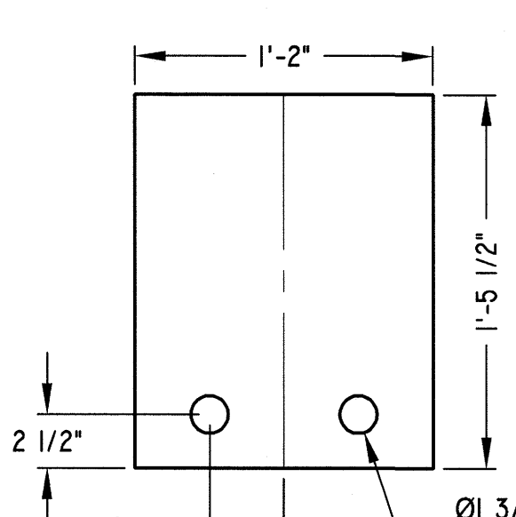
BASE PLATE SCALE: 1 1/2" = 1' 0" MAT'L: 1/4 PLATE PIECES REQ'D: 8
