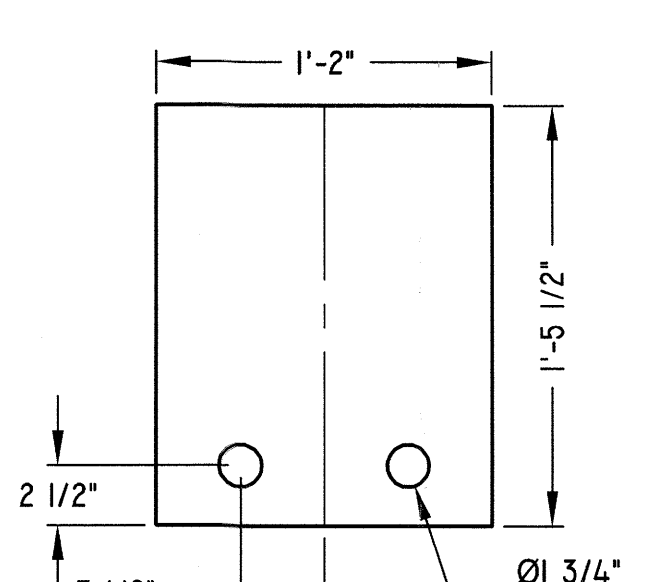
FIXED BEARING PLATE SCALE: 1 1/2" = 1' 0" MAT'L: 1" PLATE PIECES REQ'D: 4
