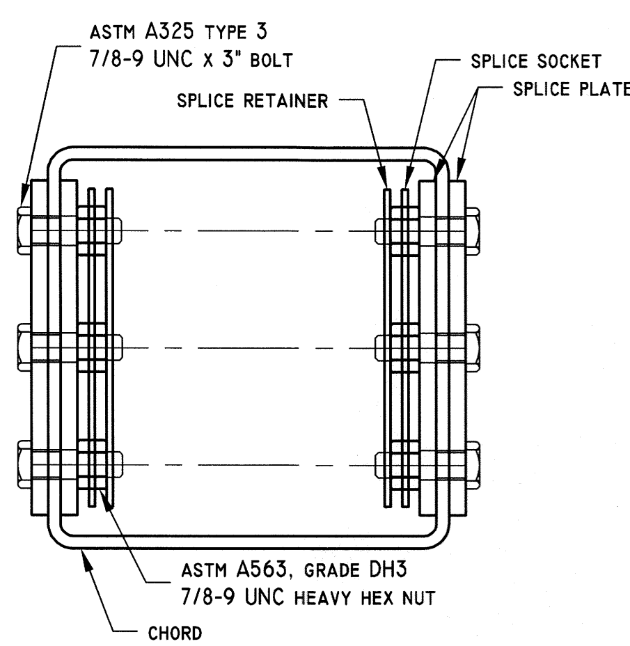
19 TYPICAL FIELD SPLICE ASSEMBLY DETAIL SCALE: NTS
