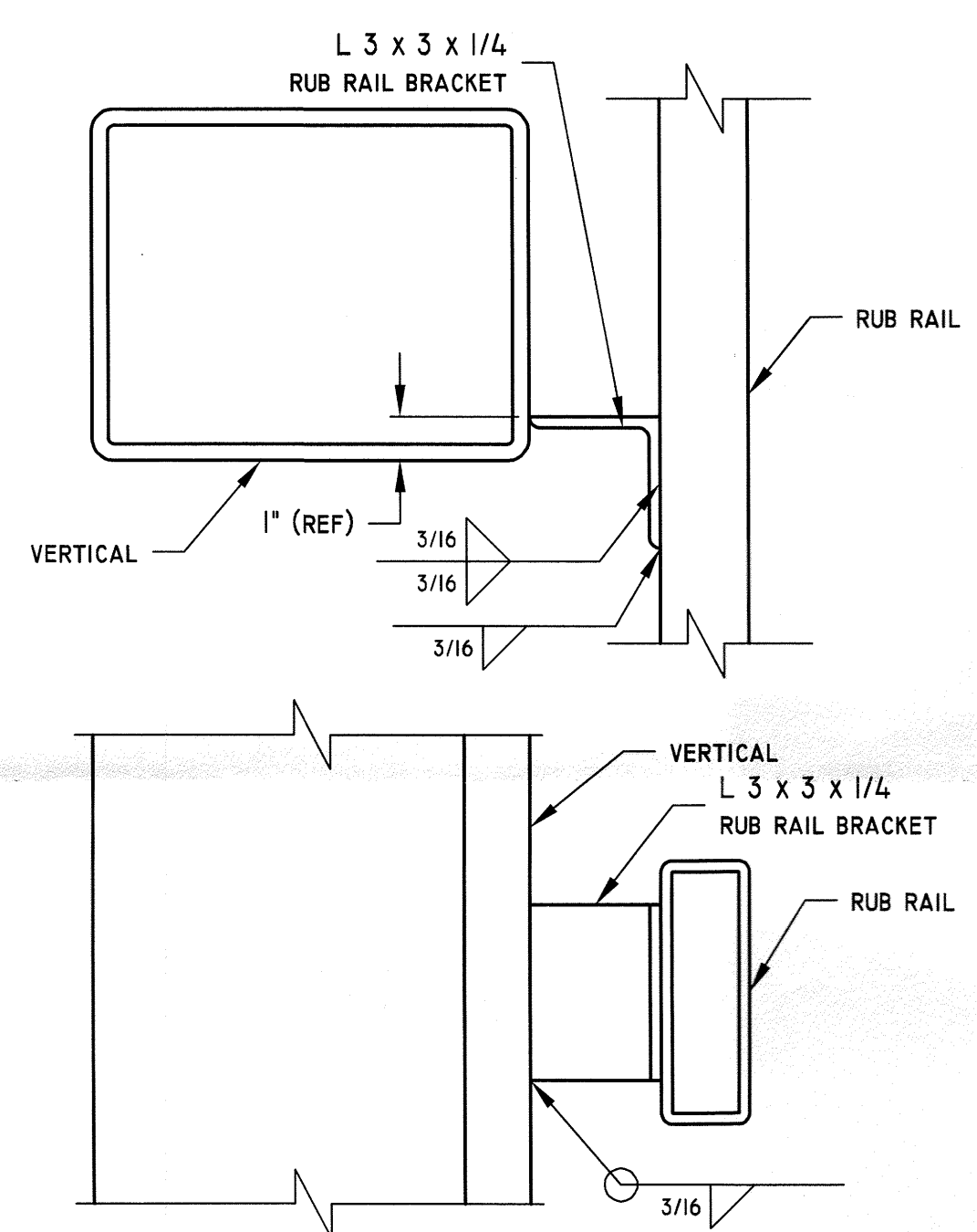
11 TYPICAL RUB RAIL CONNECTION SCALE: NTS
