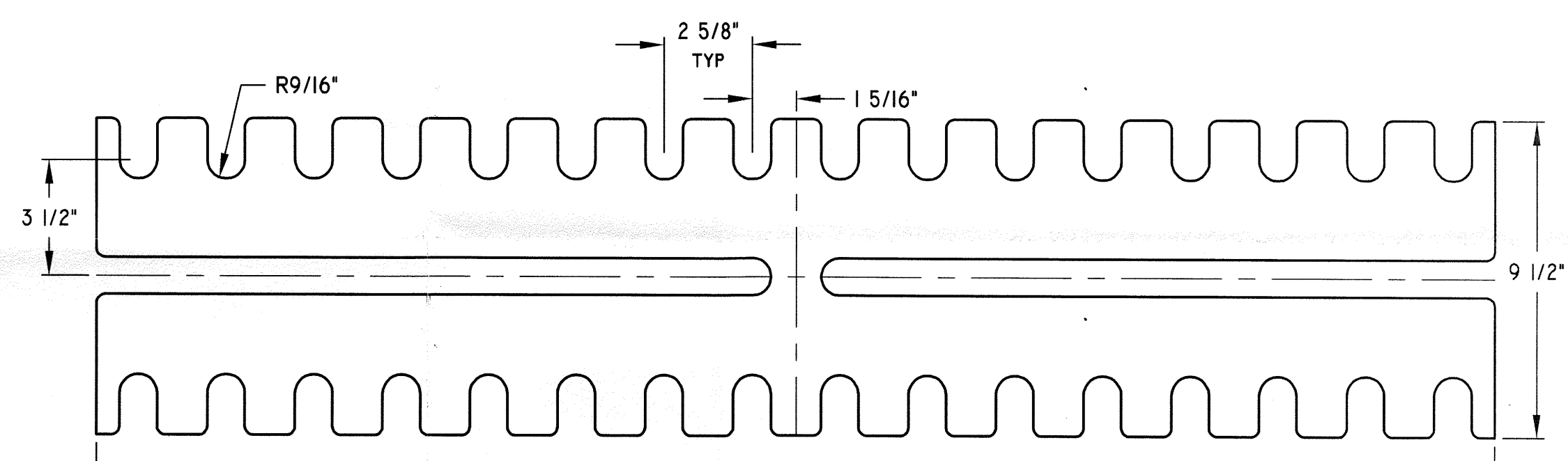
CHORD SPLICE RETAINER - SR SCALE: 3" = 1' 0" MAT'L: 3/16 PLATE PIECES REQ'D: 32
