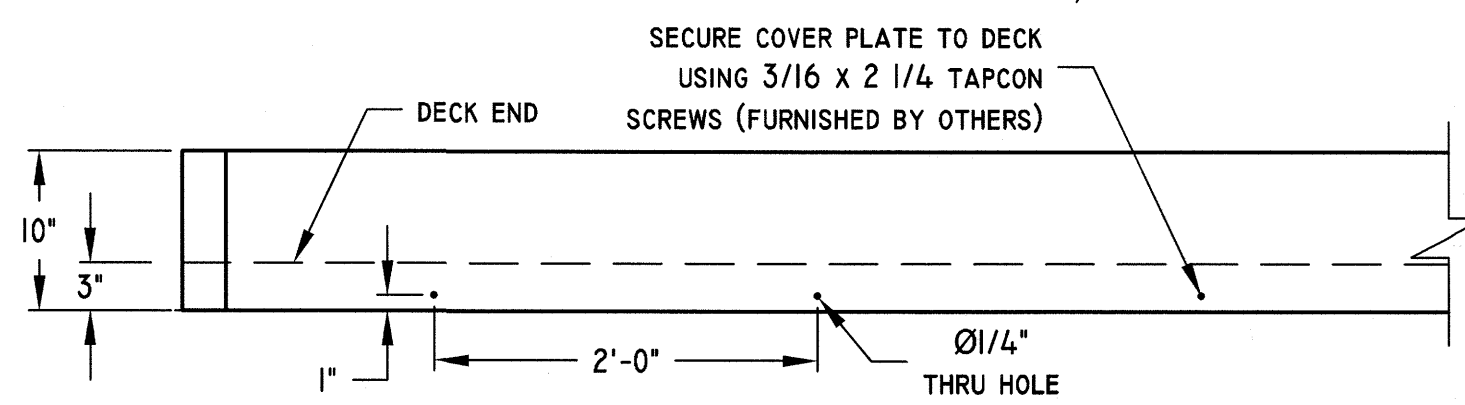
17 TYPICAL JOINT COVER DETAIL SCALE: NTS
