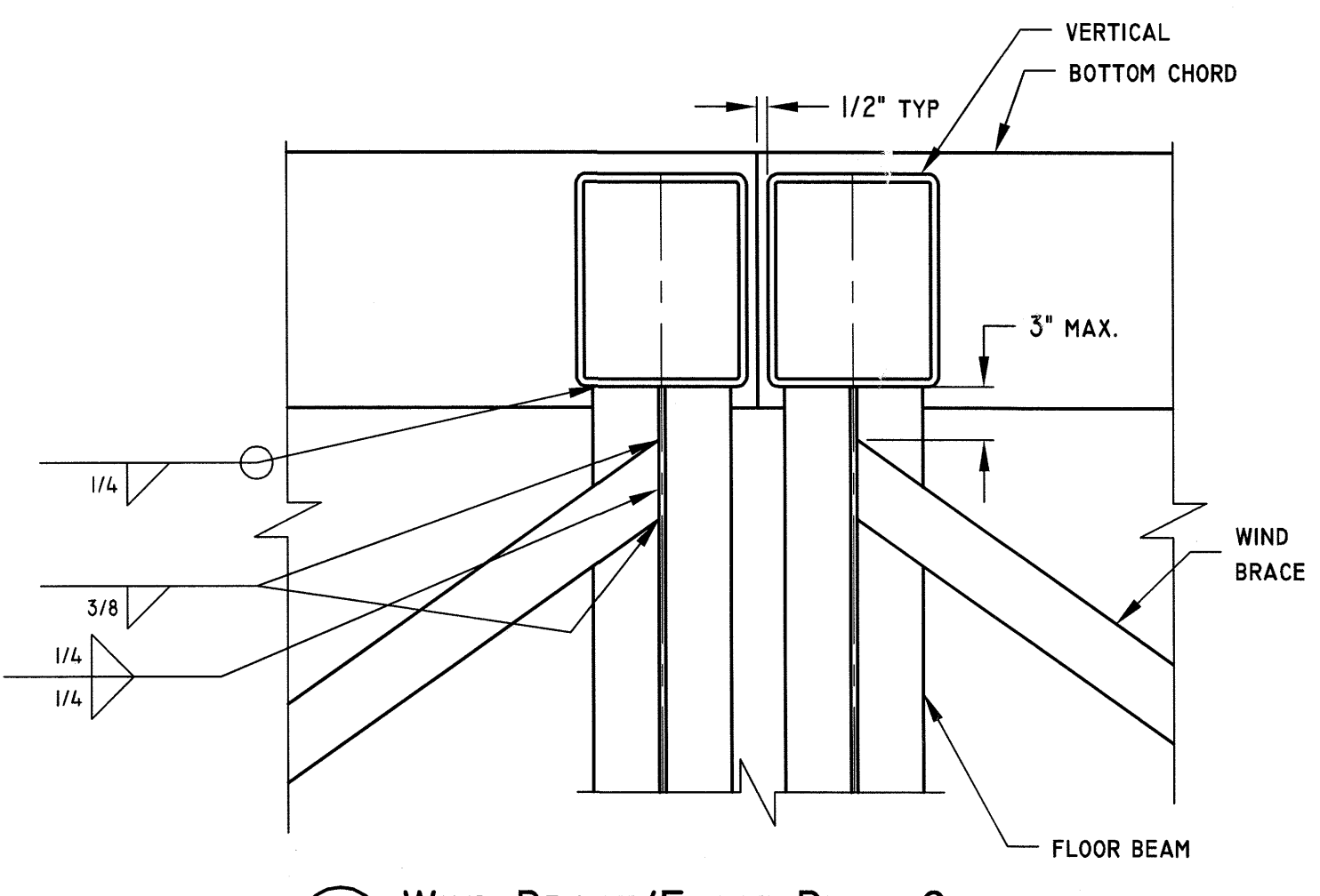
8 WIND BRACE/FLOOR BEAM CONNECTION SCALE: 1 1/2" = 1' 0"
