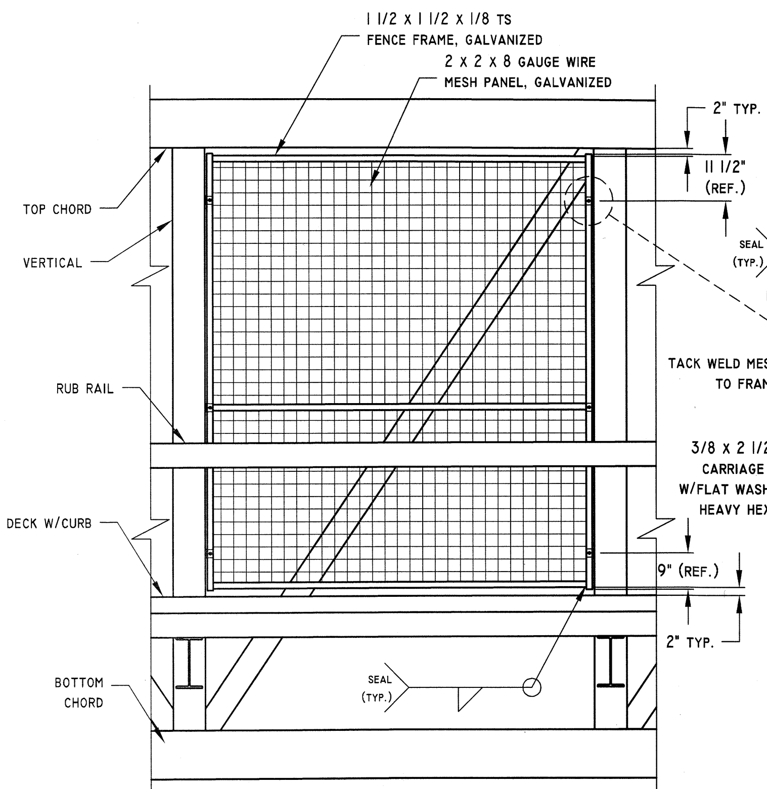
18 TYPICAL SAFETY FENCE PANEL DETAIL SCALE: 1/2" = 1' 0"
