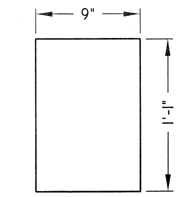
TEFLON PLATE SCALE: 3" = 1' 0" MAT'L: 1/8 PIECES REQ'D: 8
