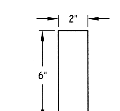
DECK END CAP - DC-2 SCALE: 3" = 1' 0" MAT'L: 1/4 PLATE PIECES REQ'D: 4
