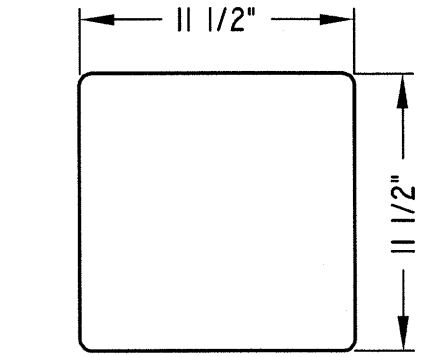
VERTICAL END CAP - EC SCALE: 3" = 1' 0" MAT'L: 1/4 PLATE PIECES REQ'D: 8
