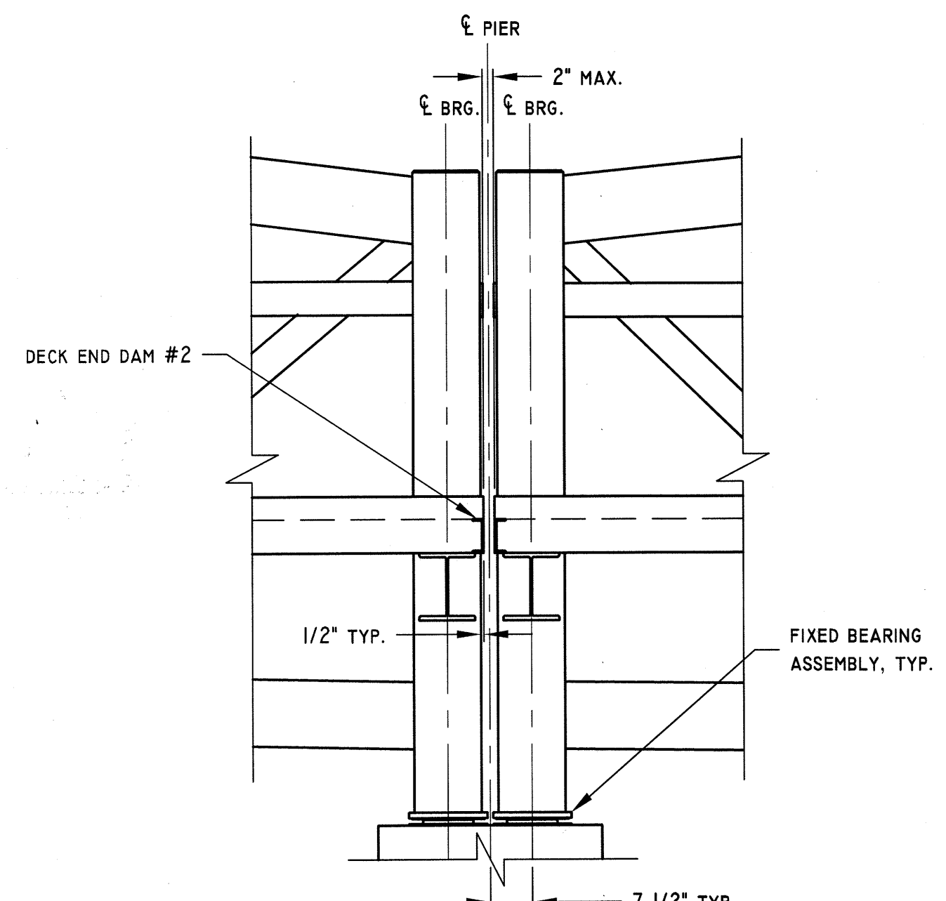
14 TRUSS ELEVATION @ PIER SCALE: 1/2" = 1' 0"
