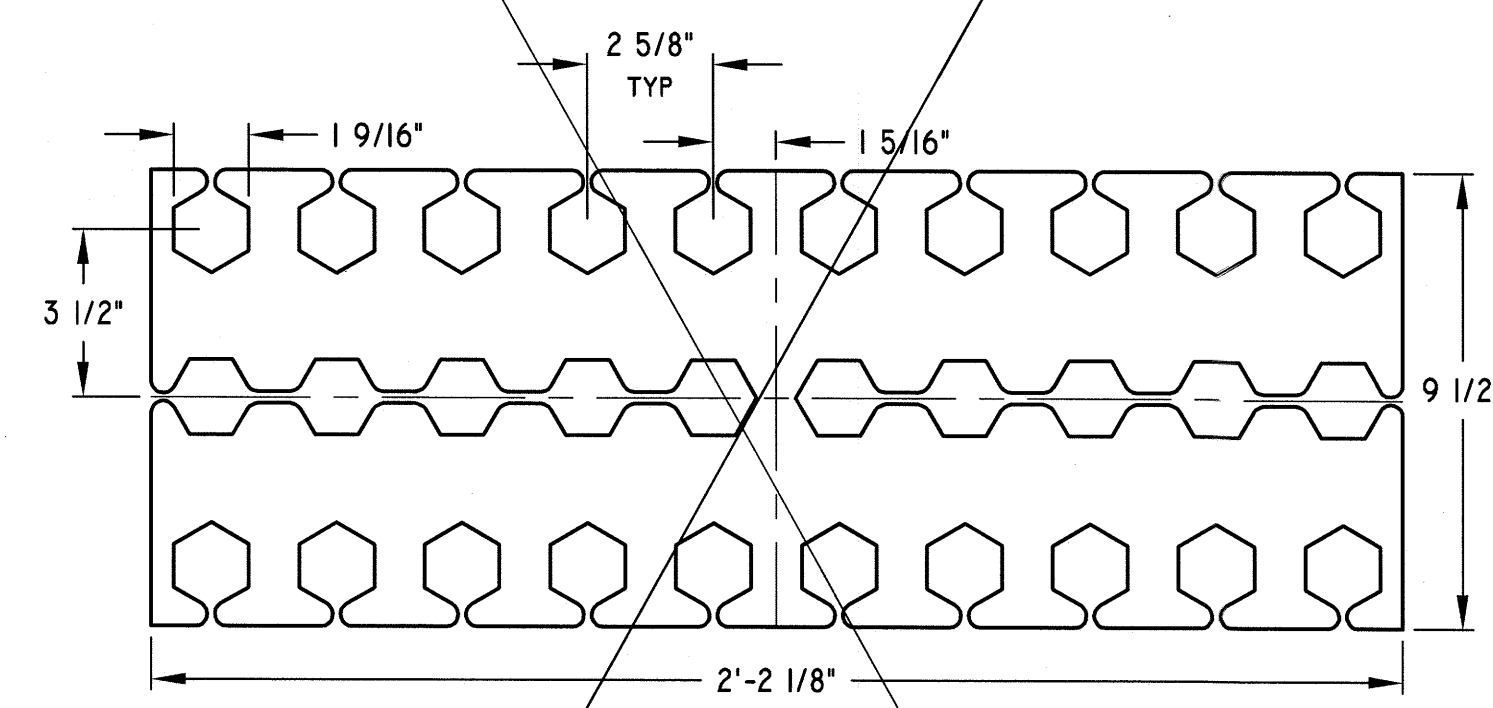
BOTTOM CHORD SPLICE SOCKET - SS-2 SCALE: 3" = 1' 0" MAT'L: 3/16 PLATE PIECES REQ'D: N/A
