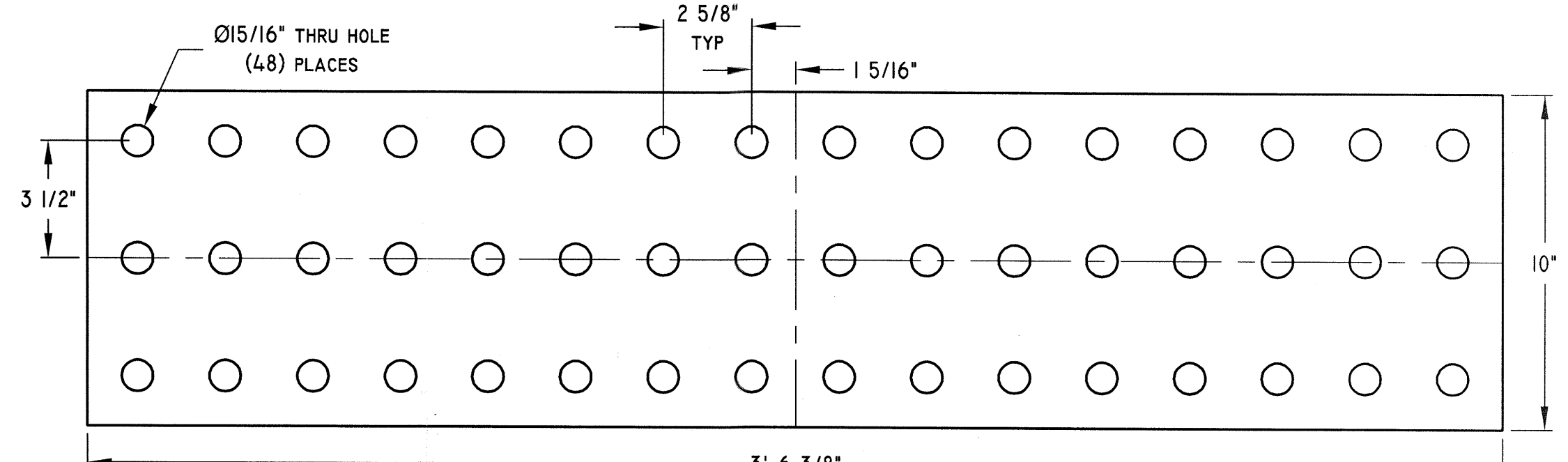
CHORD SPLICE PLATE - SP SCALE: 3" = 1' 0" MAT'L: 3/4 PLATE PIECES REQ'D: 64
