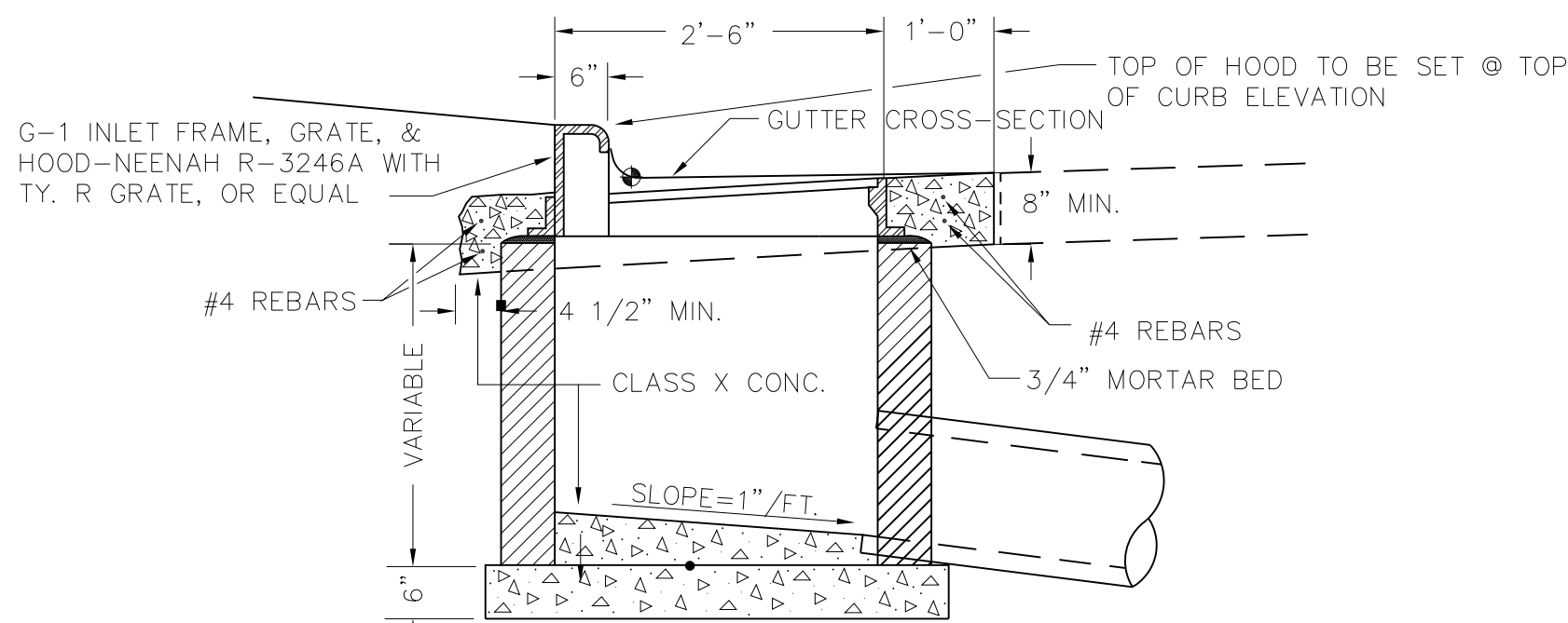
SECTION B-B
