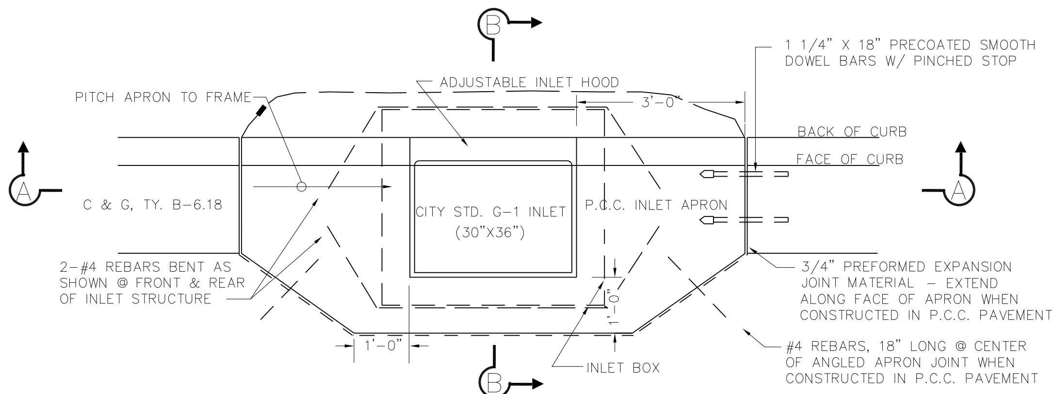
CITY STANDARD G-1 INLET DETAIL
