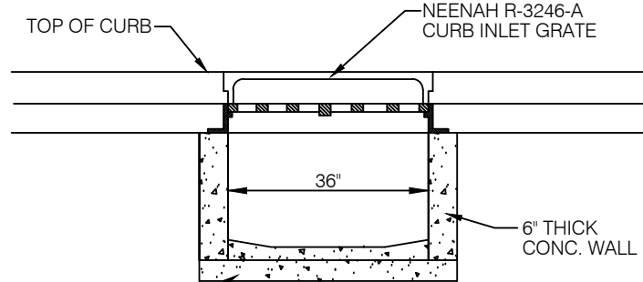
FRONT SECTION
