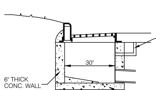
SIDE SECTION
