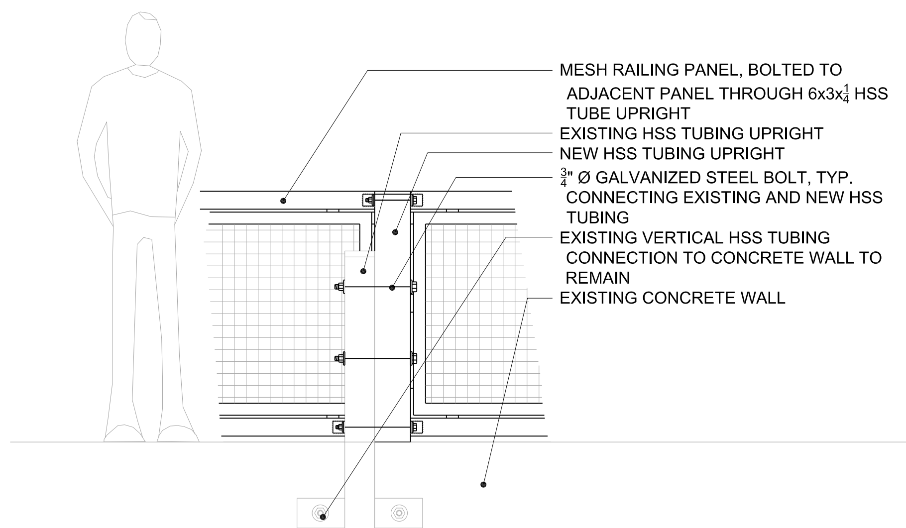
4 3 Approach Railing - Elevation 3/4" = 1'-0"
