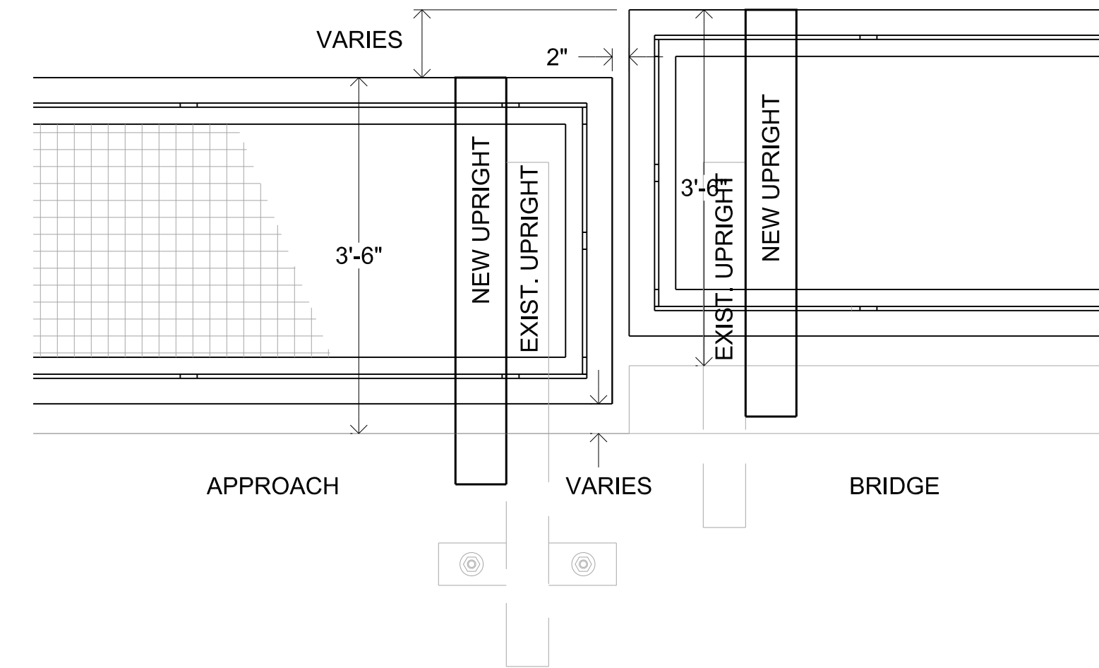
6 3 Approach and Bridge Junction - Elevation 3/4" = 1'-0"
