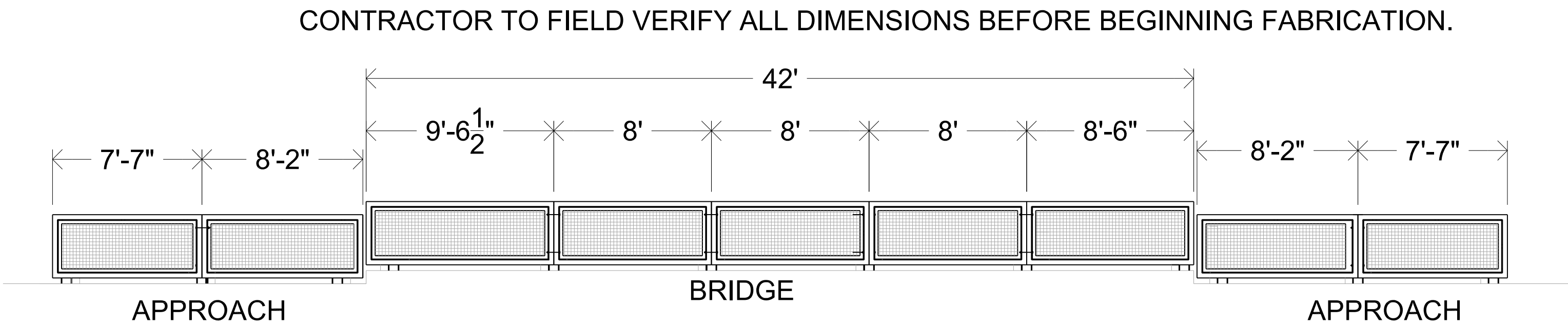
2 Panel Lengths 2 1" = 5'-0"
