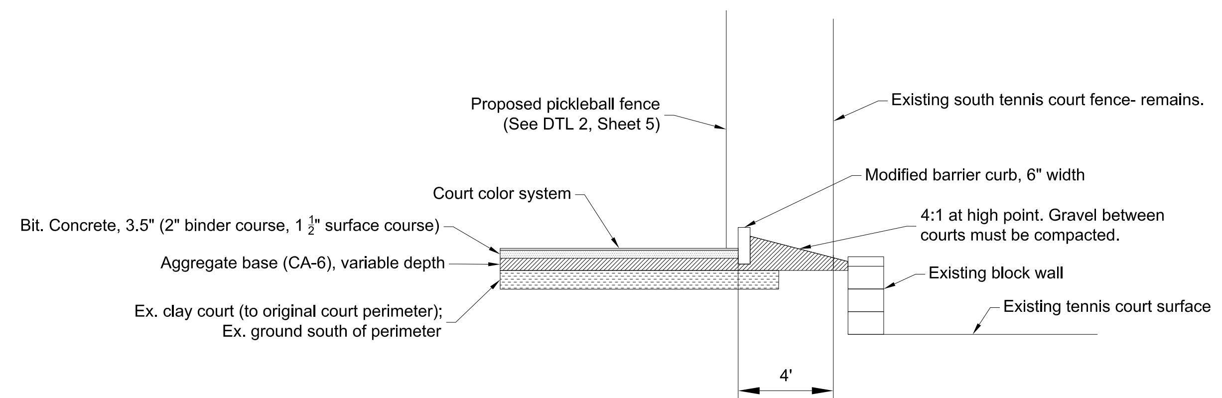
5.1 ADD ALTERNATE 1 Section- Southern Edge 4 NOT TO SCALE
