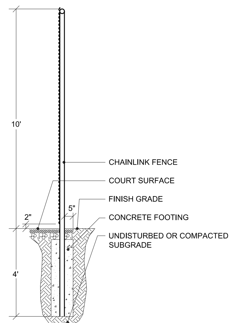
2 New Chain Link Fence 4 NOT TO SCALE
