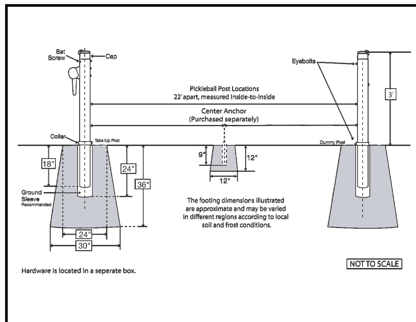
3 Pickleball Net Post and Anchor 4 NOT TO SCALE
