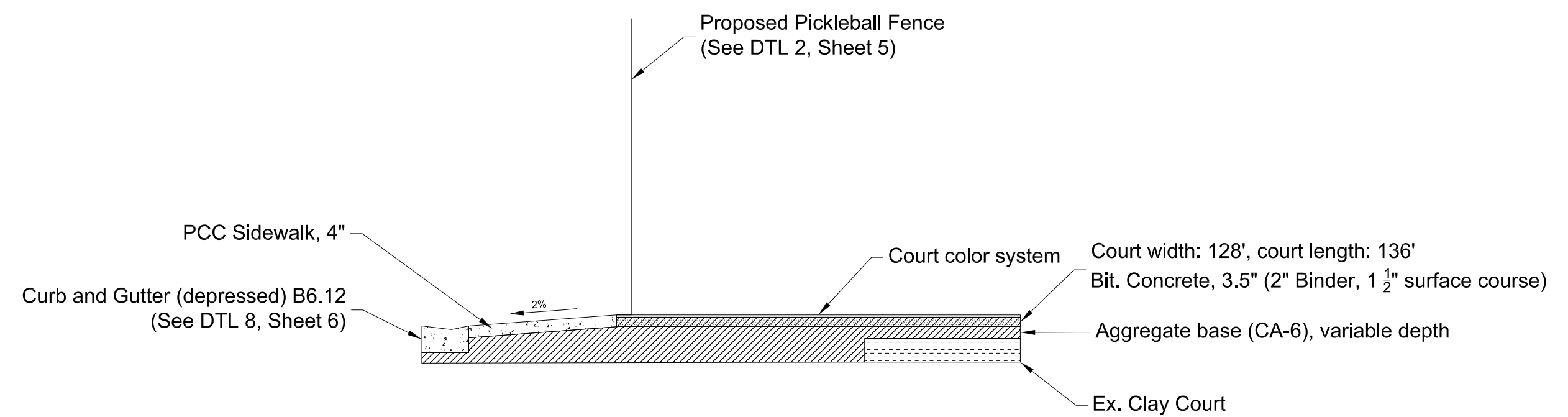
4 Northern Edge Section- With Sidewalk 4 NOT TO SCALE
