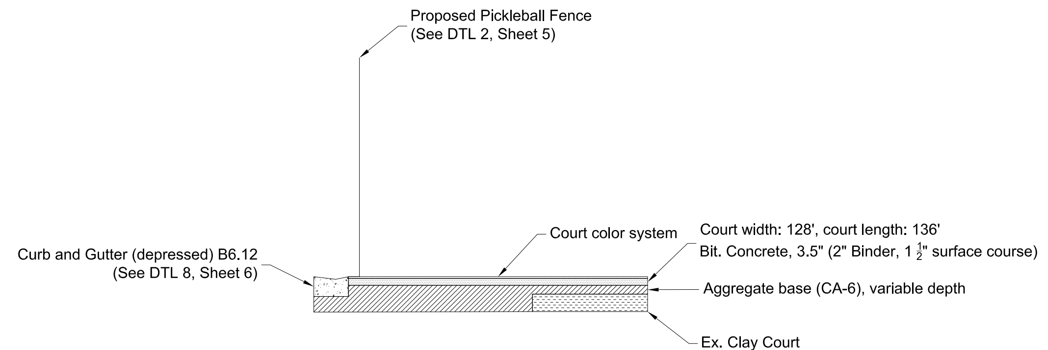
4.1 Northern Edge Section- Without Sidewalk 4 NOT TO SCALE
