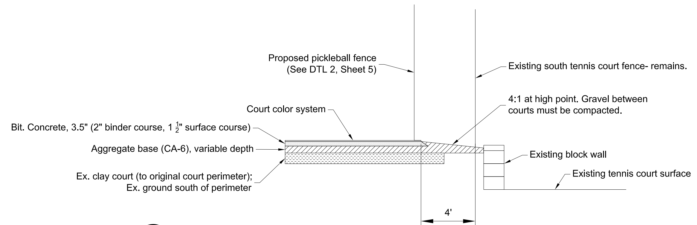
5 Typ Section- Southern Edge 4 NOT TO SCALE
