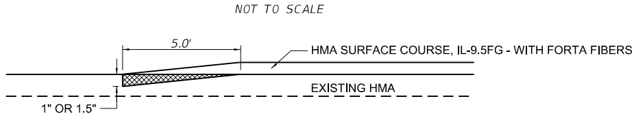
BUTT JOINT DETAIL (TYPICAL ALL LOCATIONS)
