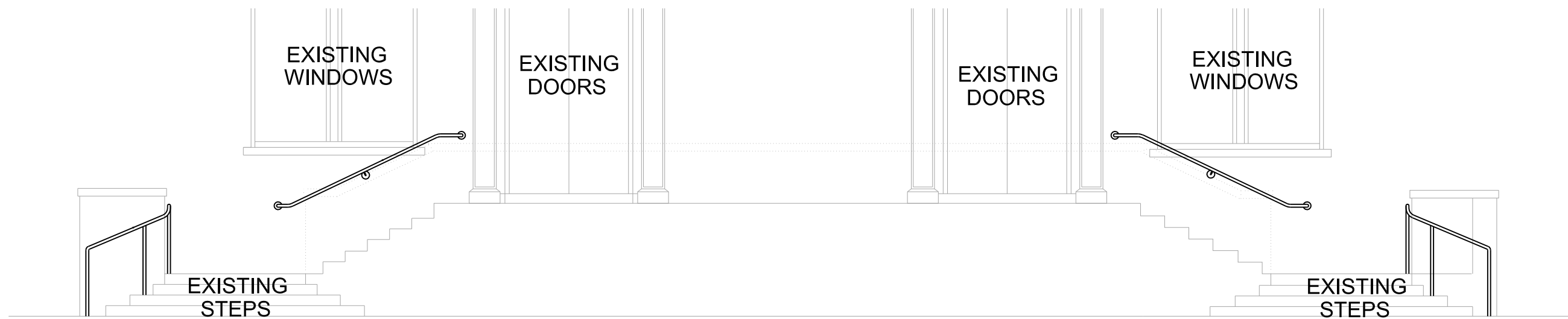
2 ELEVATION VIEW 2 1" = 5'-0"
