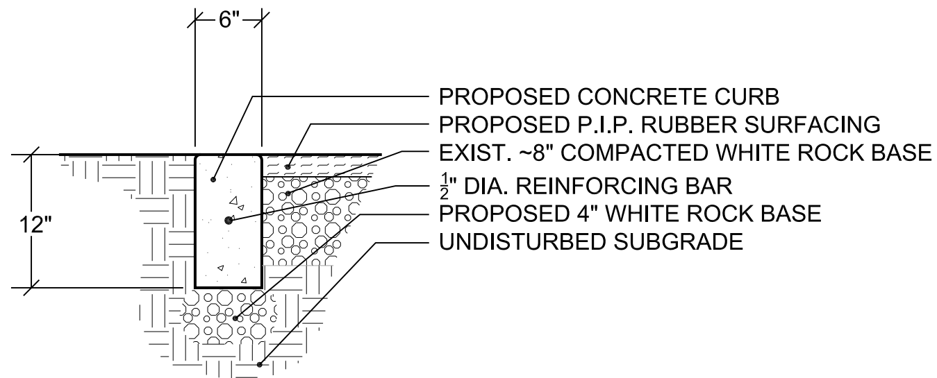
1 Concrete Curbing Detail 1" = 1'-0"
