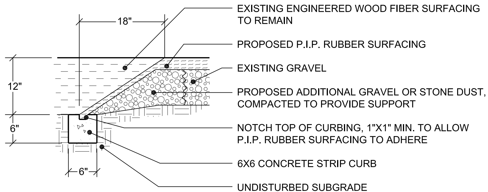
2 Transition Between PIP Rubber and Loose Fill Surfacing 1" = 1'-0"
