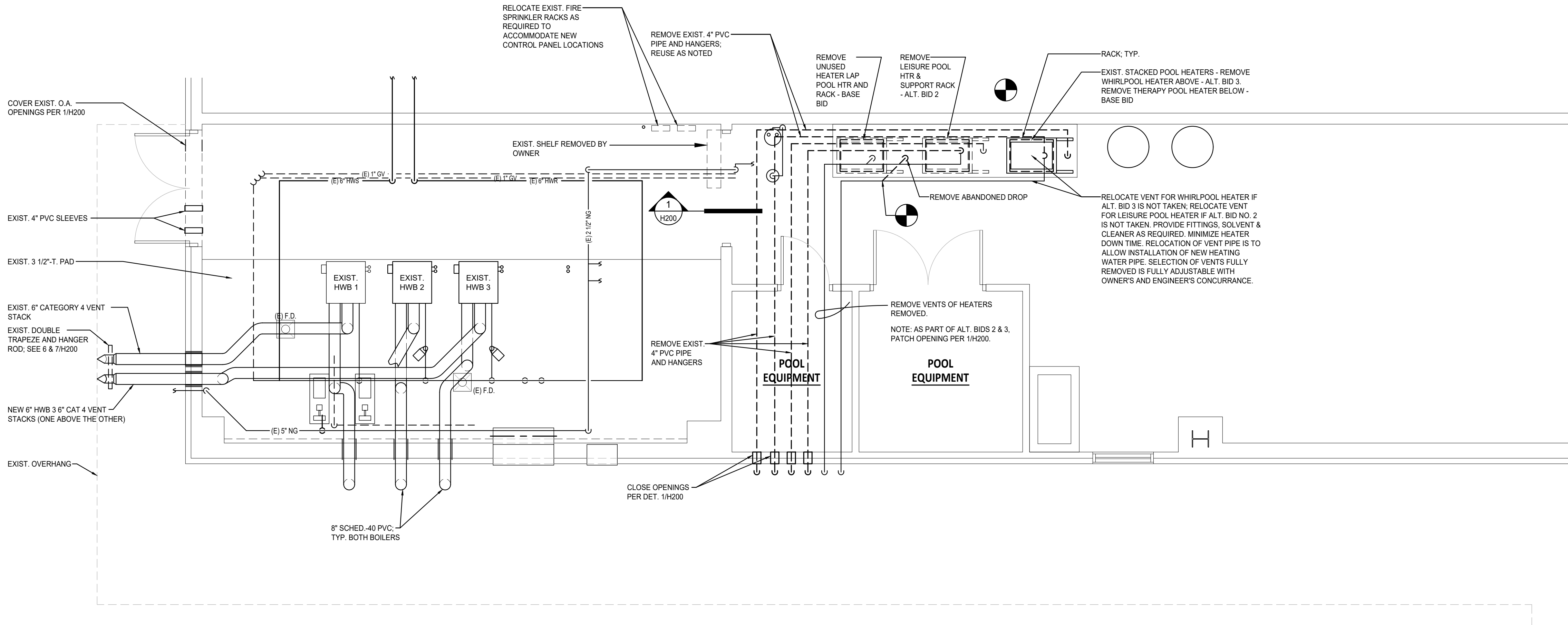
2 Pool Heater Vent Pipe Plan - Demolition scale: 1/4" = 1'-0"
