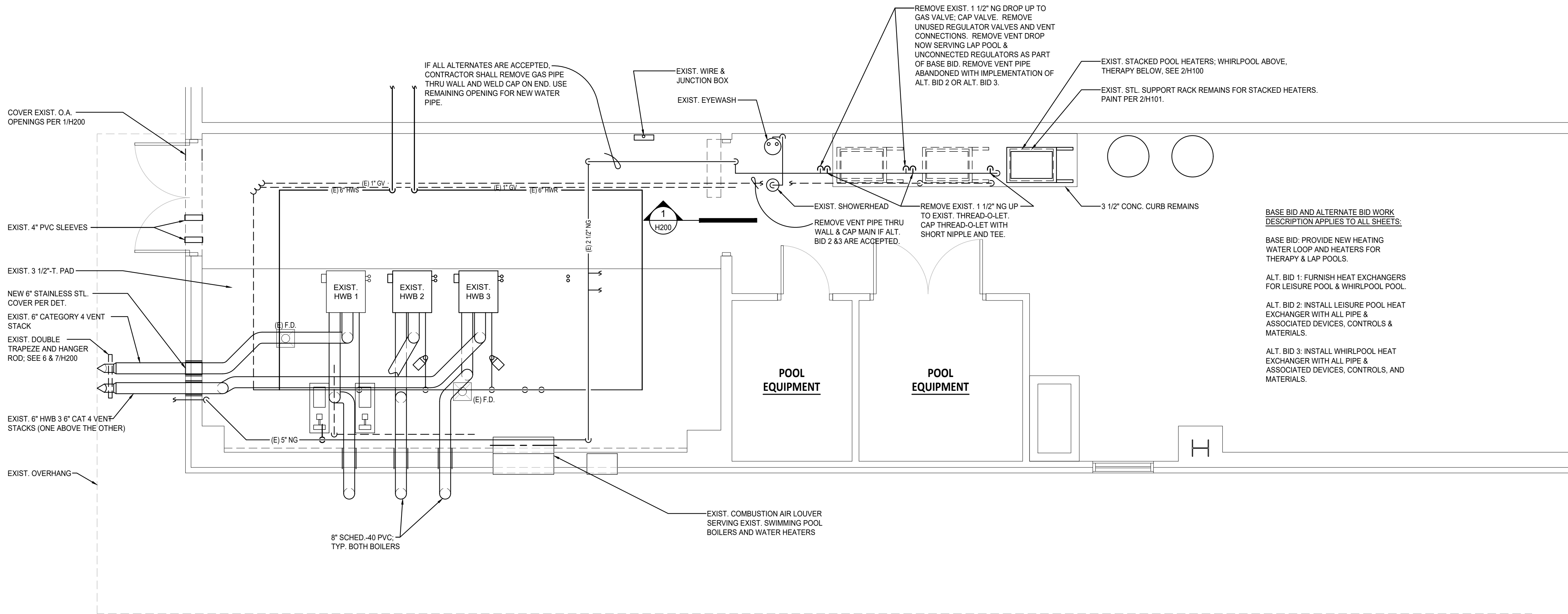
1 Natural Gas Pipe Pool Heater Plan - Demolition scale: 1/4" = 1'-0"
