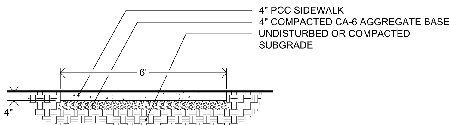
2 PCC Sidewalk S1 NOT TO SCALE
