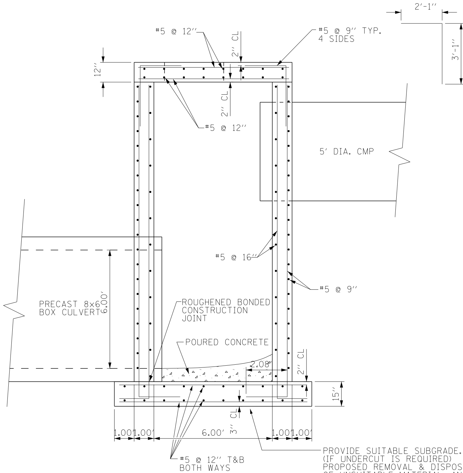
SECTION VIEW DROP STRUCTURE DETAIL
