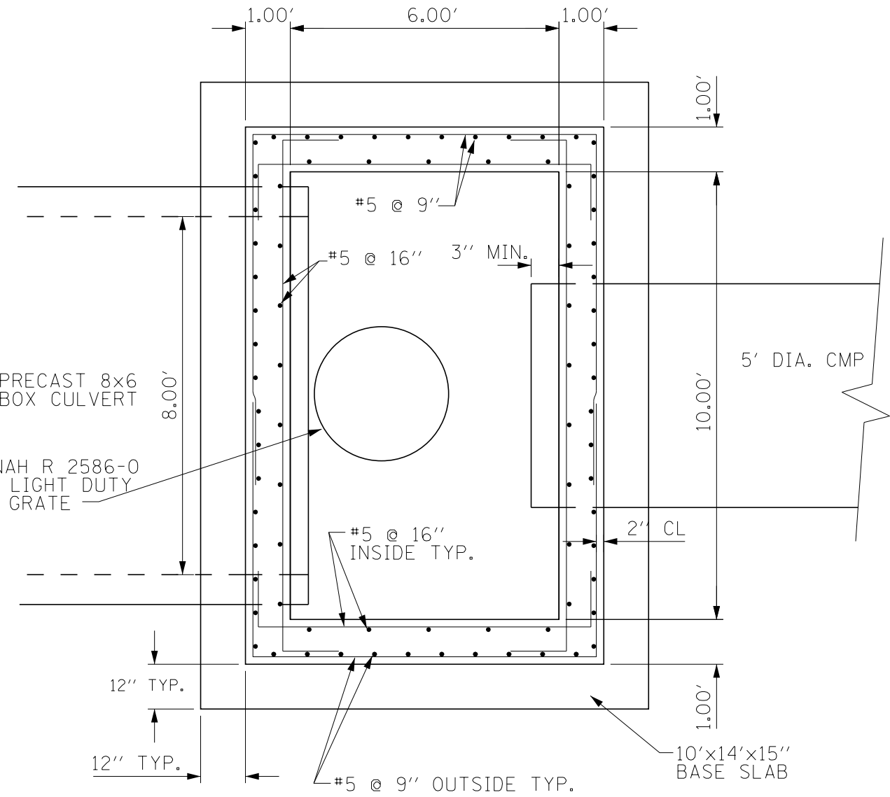
PLAN VIEW
