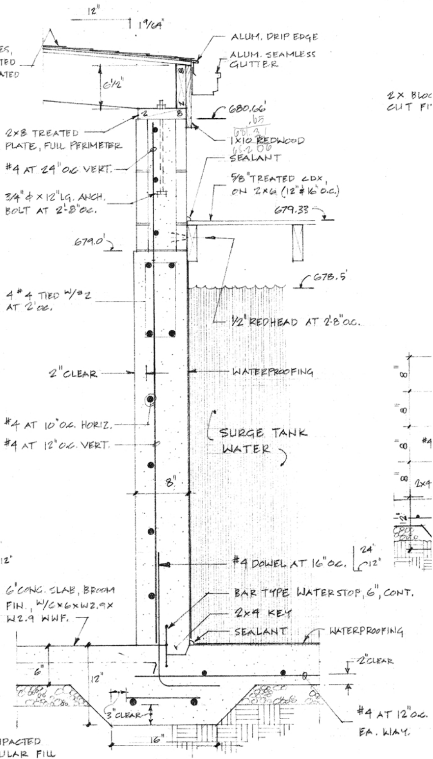
2 PUMP RM-SURGE TANK WALL SECTION 1/2" = 1'-0"
