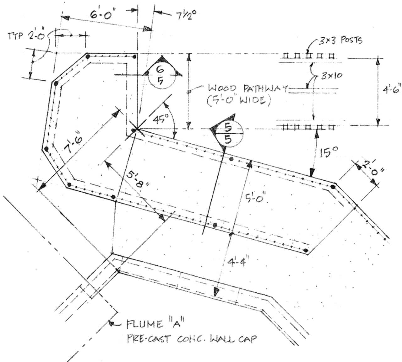
4 5 RAMP DETAIL - PLAN 1/4" = 1'-0"
