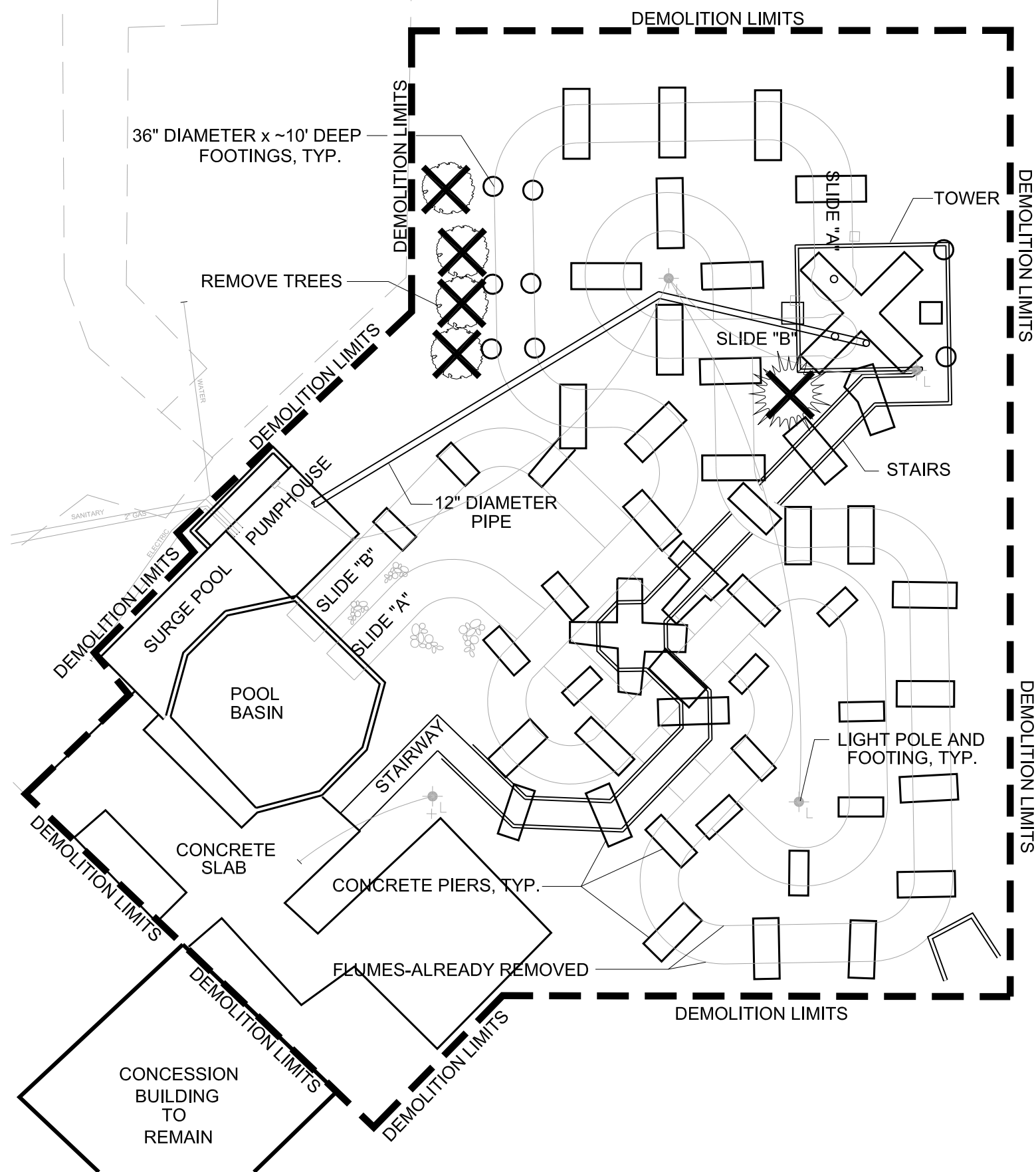
1 1 1"=20' Demolition Plan/Existing Conditions
