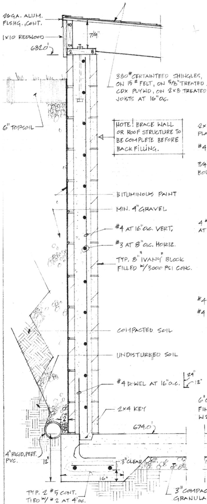
1 PUMP RM. WALL SECTION 1/2" = 1'-0"
