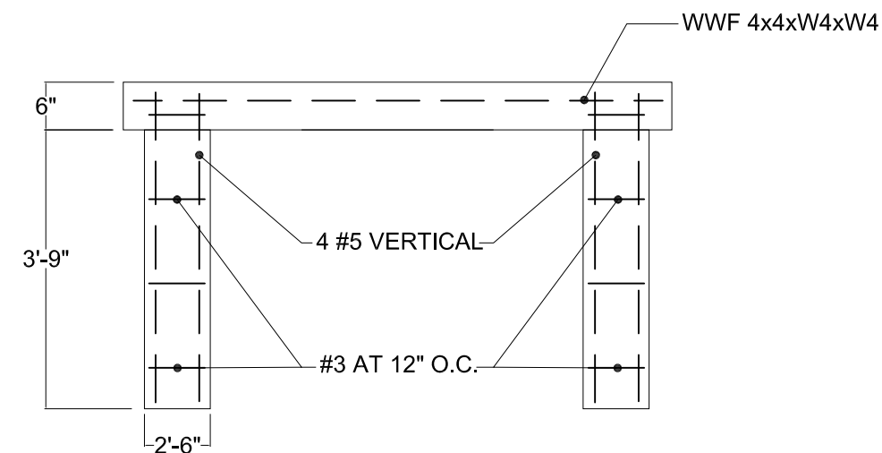
2 1 NTS Typical Pier Section
