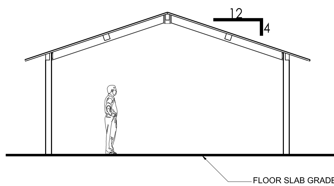
5 Elevation View, Side Shelter NOT TO SCALE
