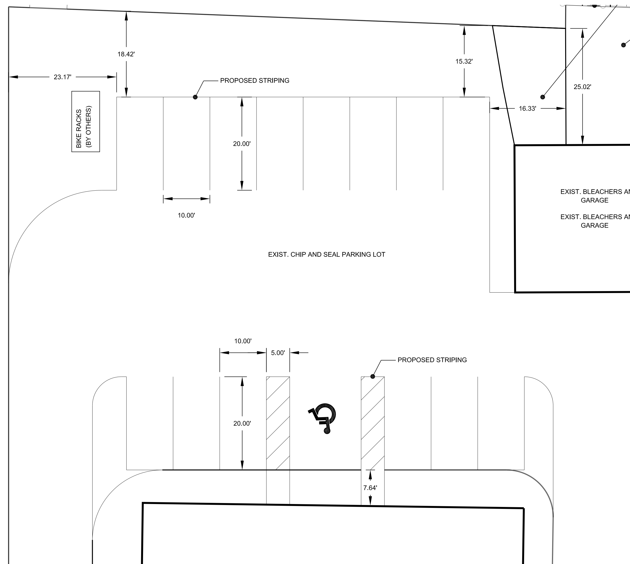
6 Parking Lot Striping NOT TO SCALE
