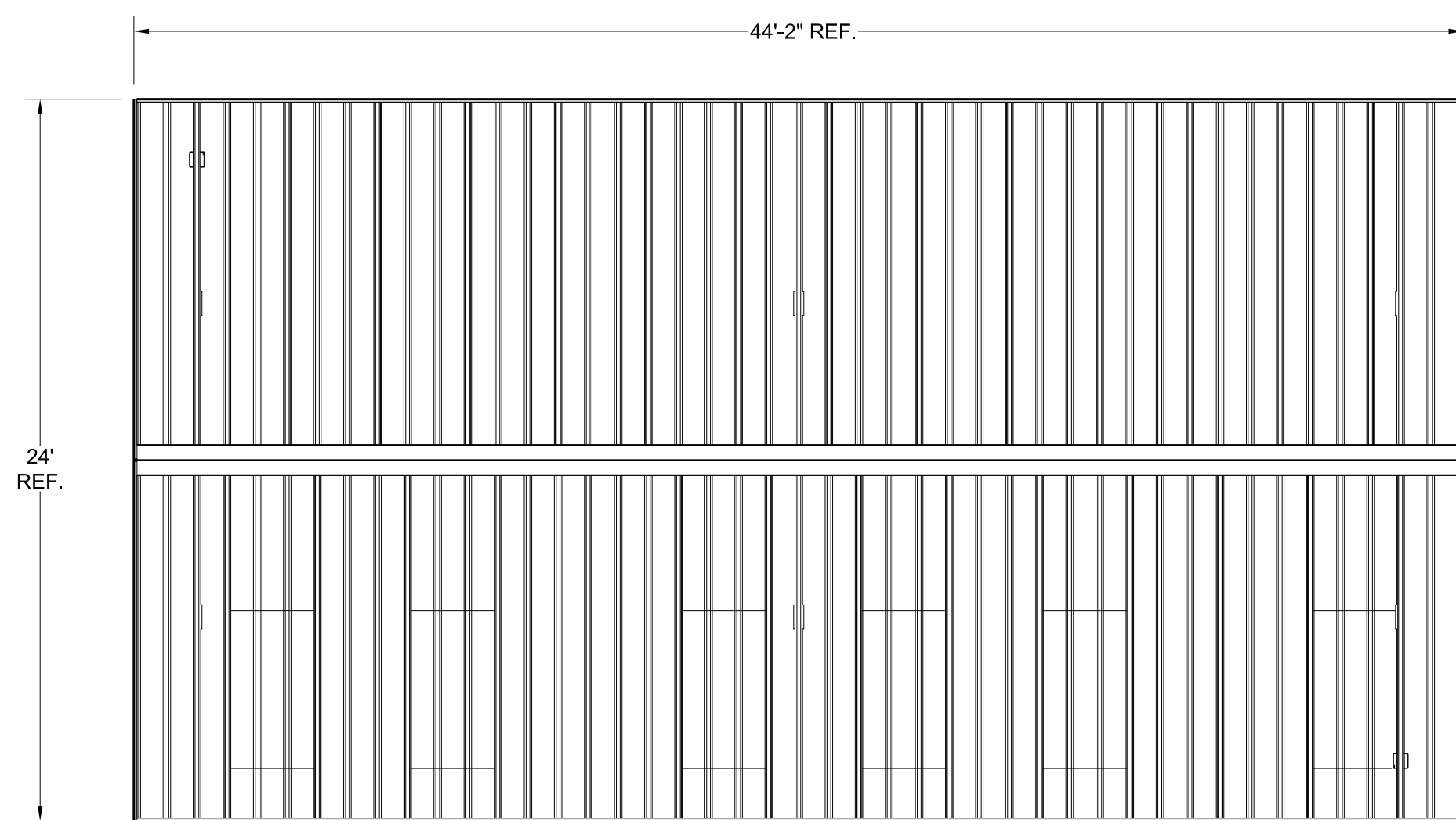
3 Plan View - Shelter NOT TO SCALE
