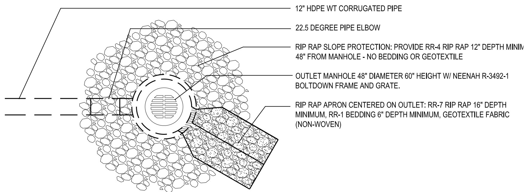
3 Outlet Detail 2 NOT TO SCALE
