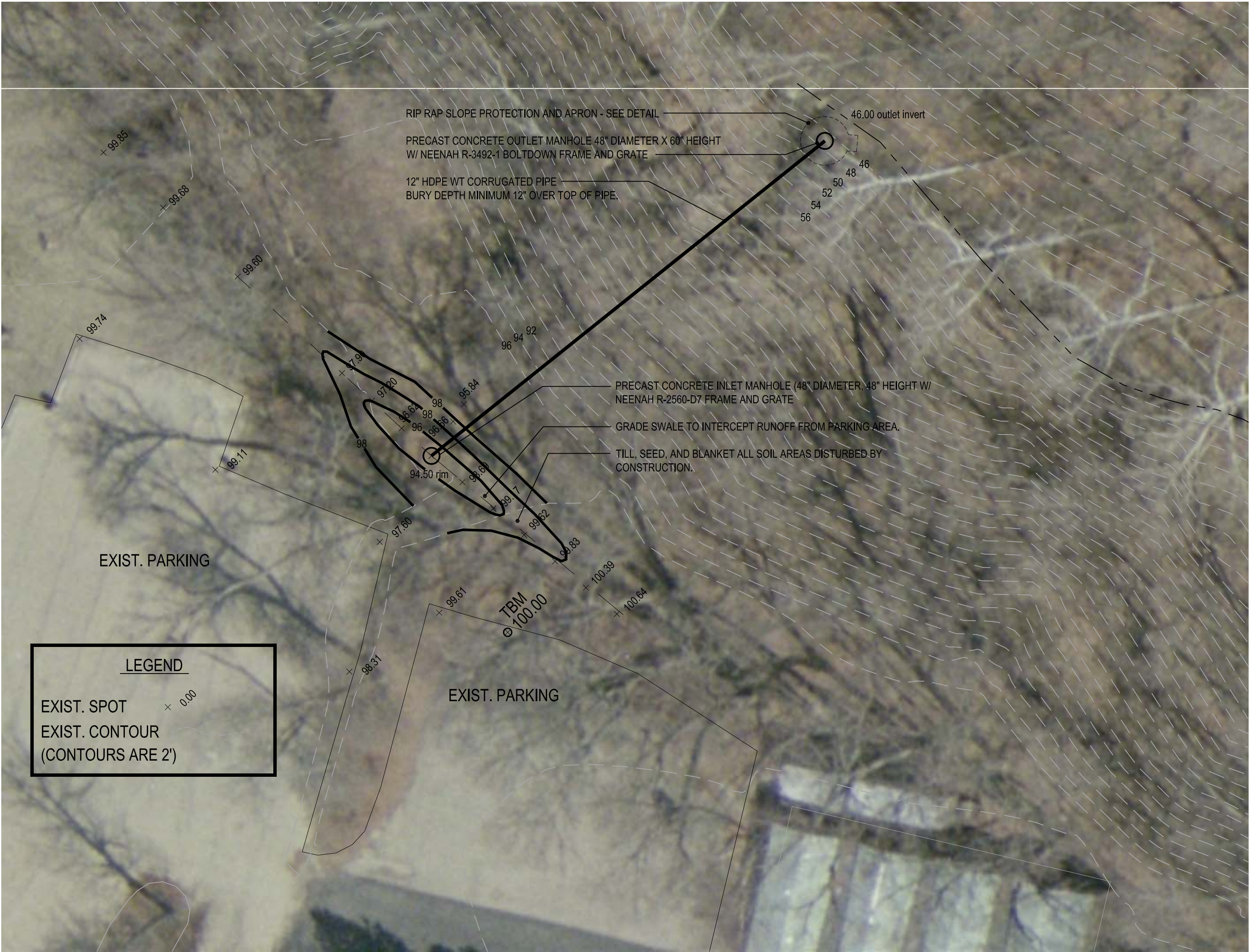
1 Site Plan 2 1" = 20'
