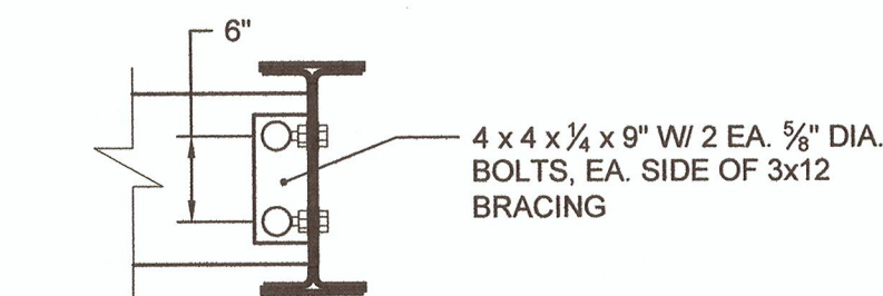
3 Brace Beam Connection Detail 1 NOT TO SCALE
