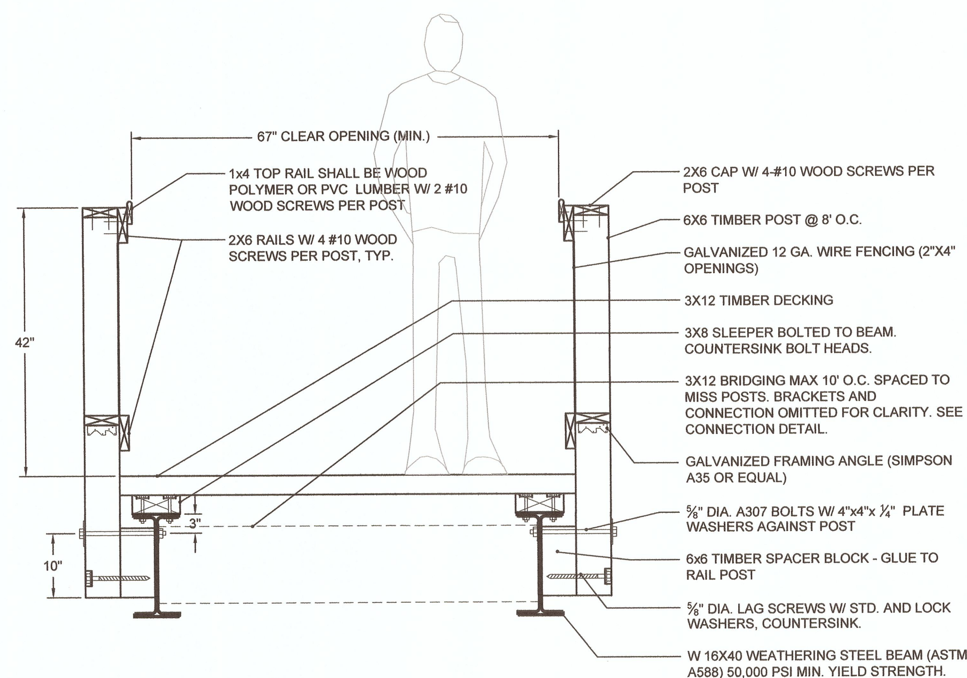
2 Typical Section 1 NOT TO SCALE
