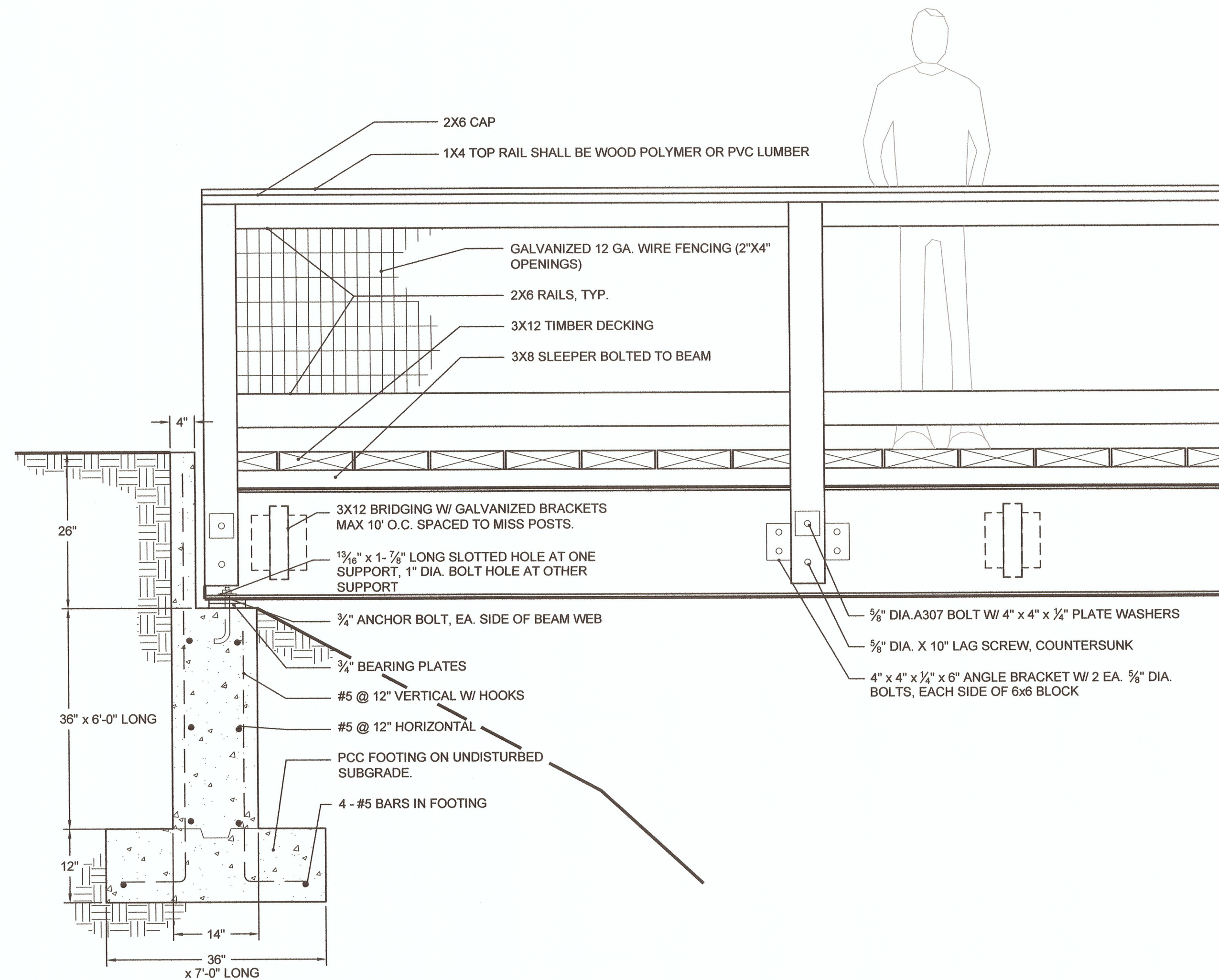
1 Section / Elevation 1 NOT TO SCALE
