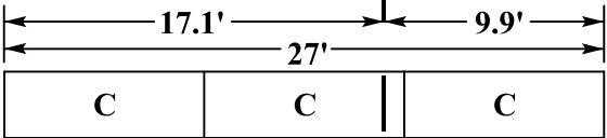
Gabion Wall Layer #2
