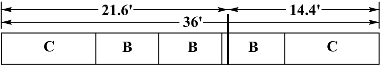
Gabion Wall Layer #5
