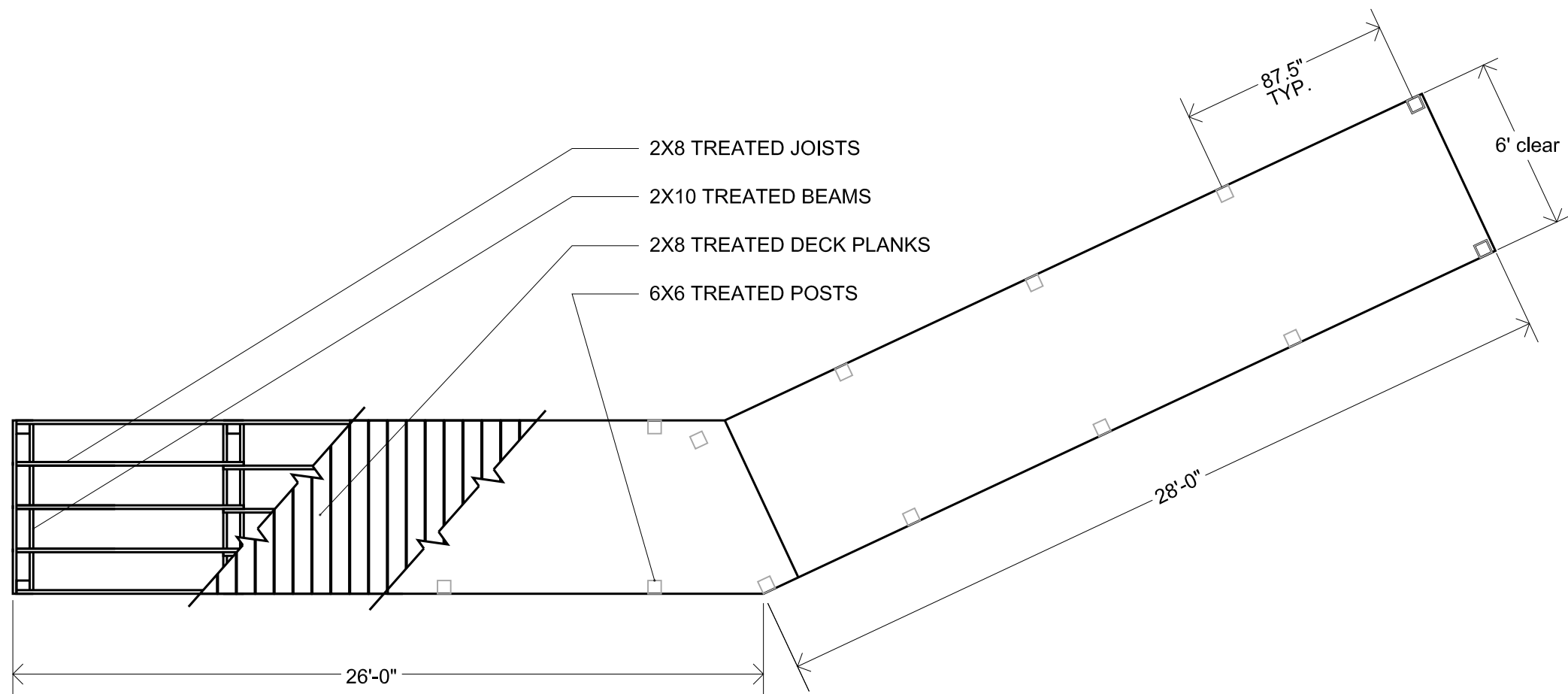
3 Boardwalk Plan View 5 NOT TO SCALE
