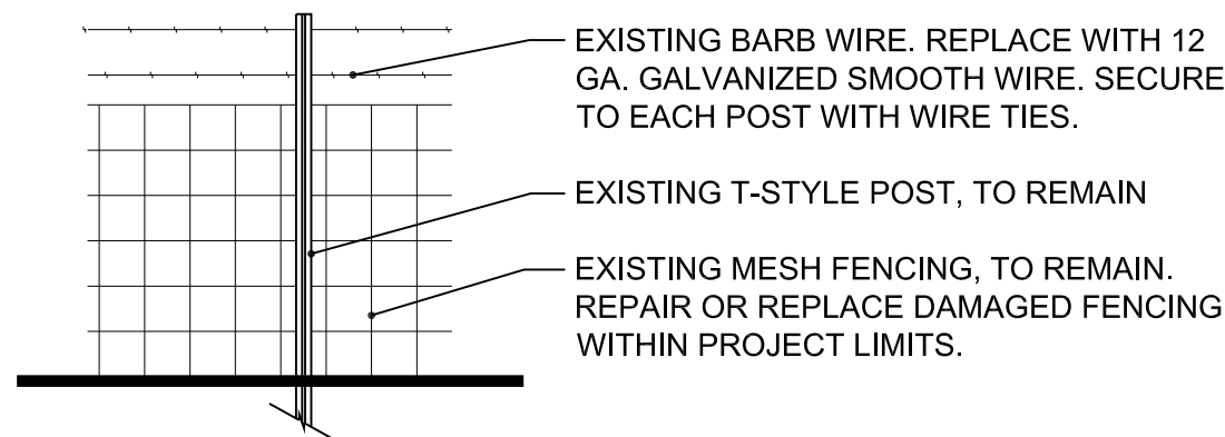
6 Existing Fence Modification 5 NOT TO SCALE
