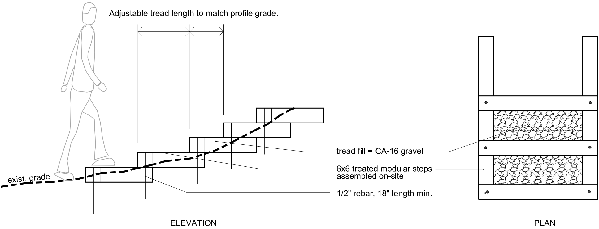
2 Tunnel Approach Steps 5 NOT TO SCALE
