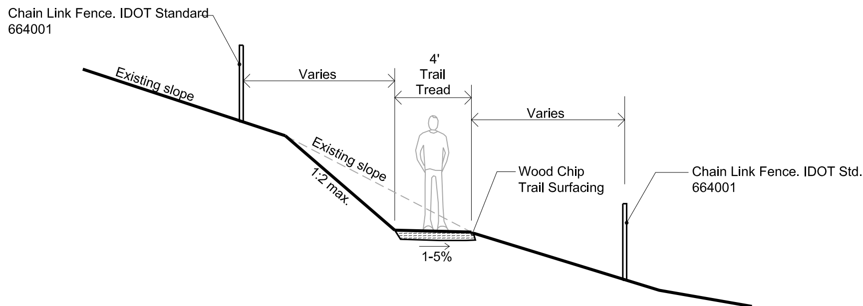
1 Trail in Cut Condition 5 NOT TO SCALE
