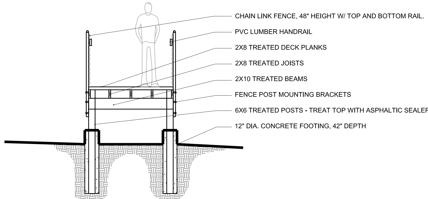
5 Boardwalk Cross Section 5 NOT TO SCALE
