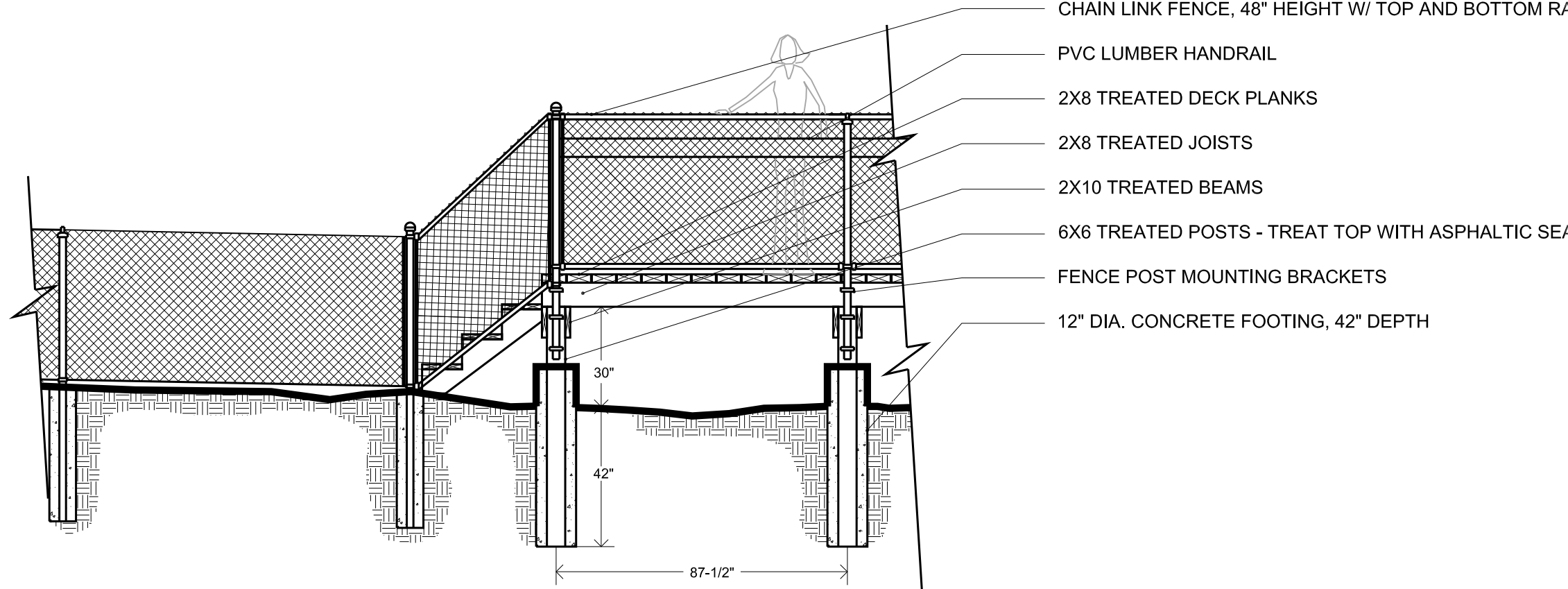
4 Boardwalk Elevation at Approach 5 NOT TO SCALE
