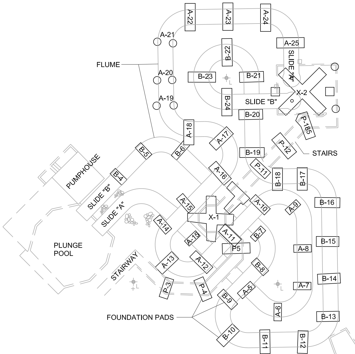
1 Structure Plan 1 1"=20"
